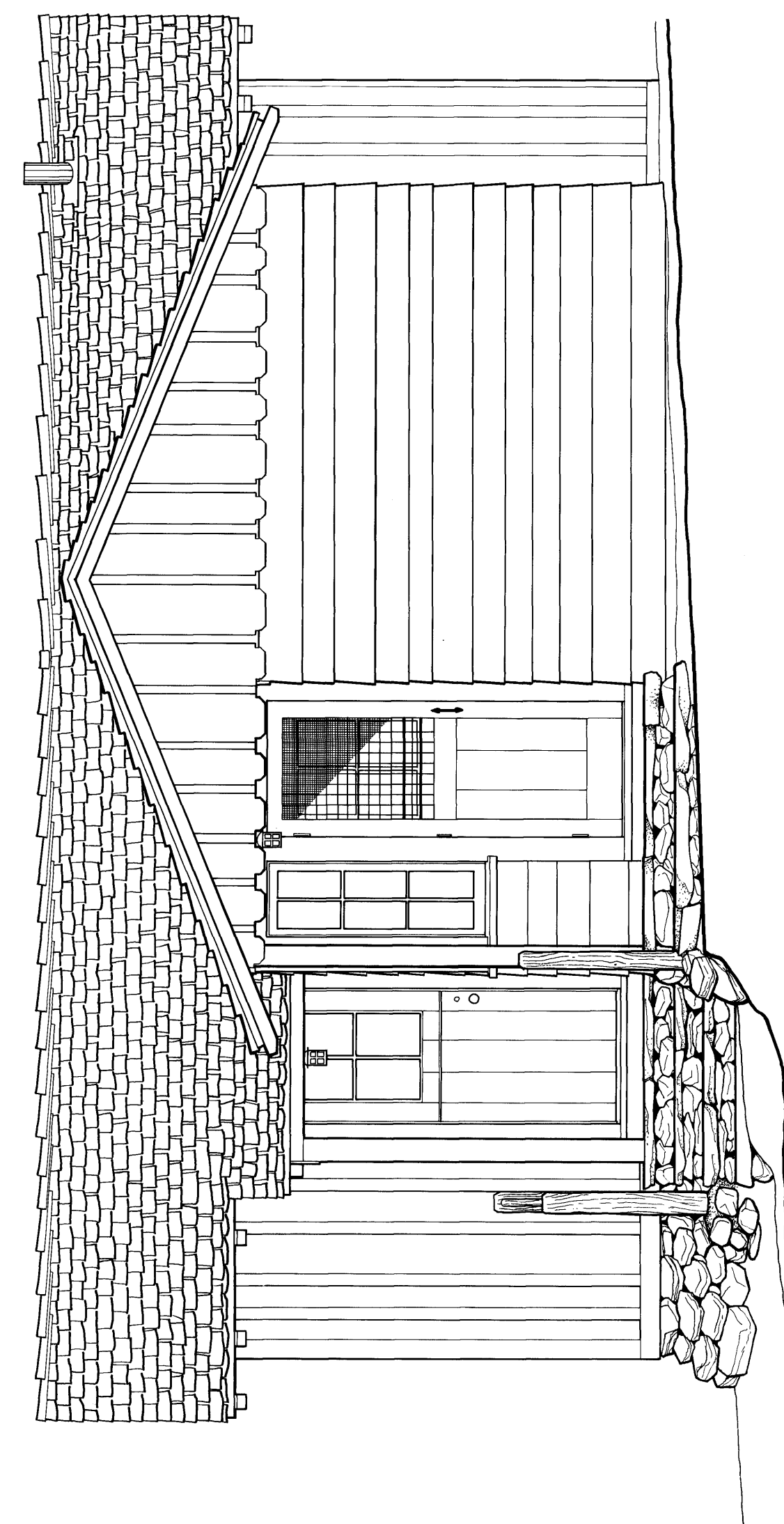
EAST ELEVATION
