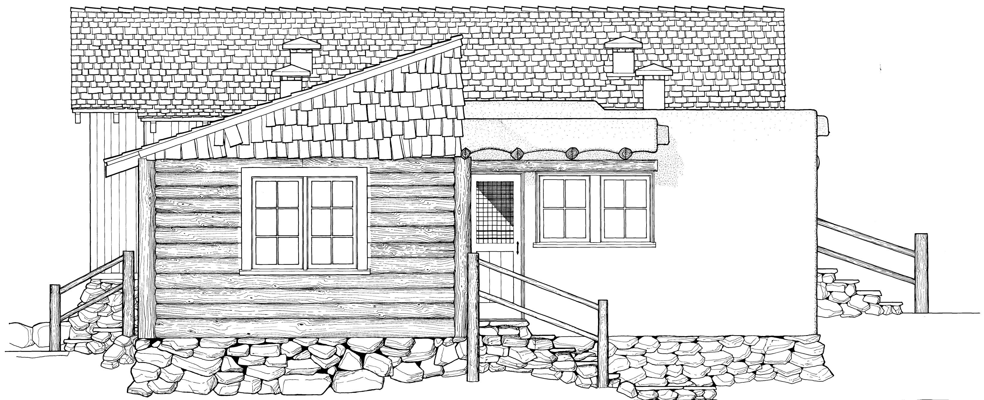
SOUTH ELEVATION
