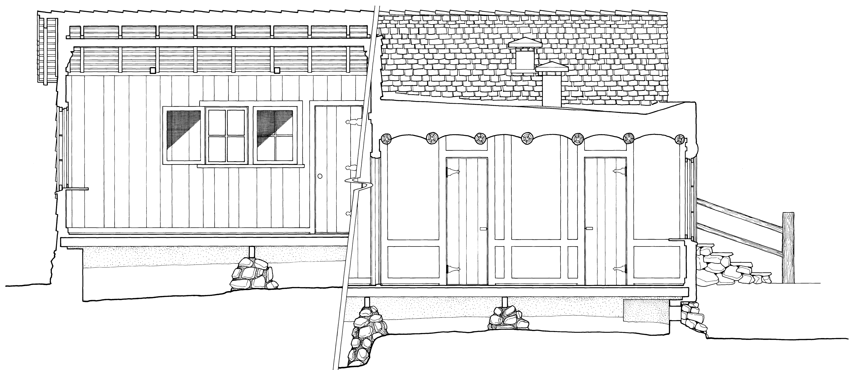
EAST/WEST SECTION
