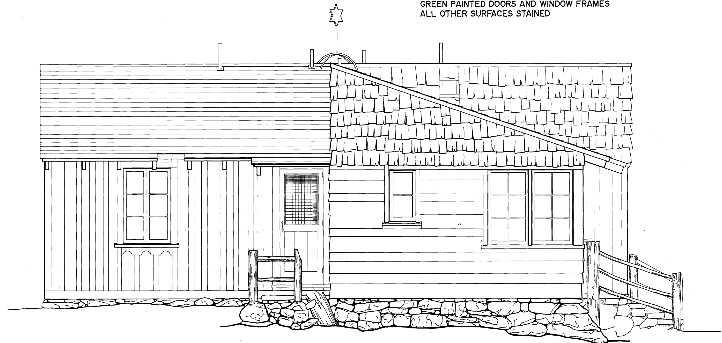
WEST ELEVATION
