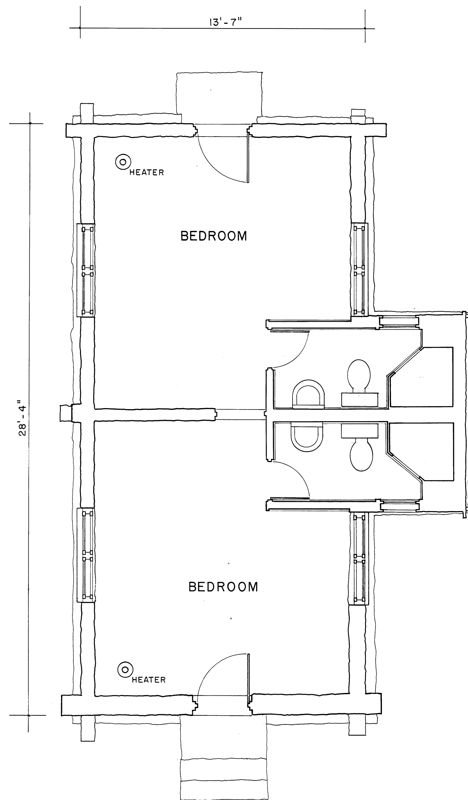
PLAN
