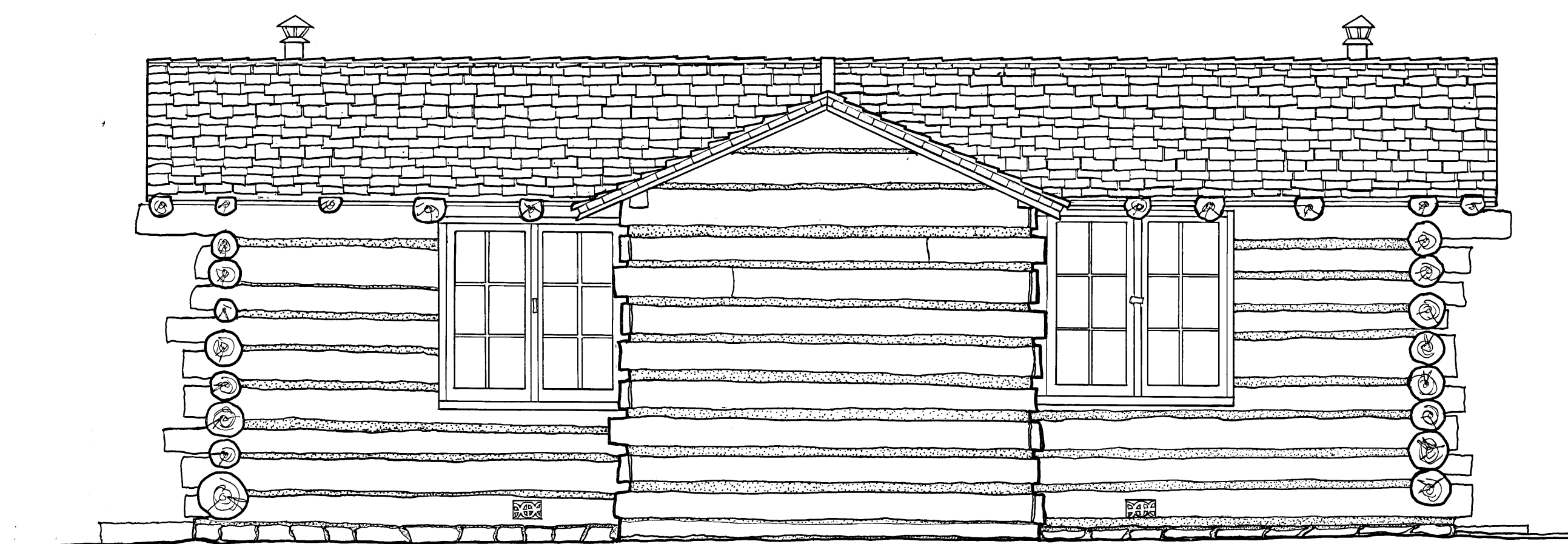
EAST ELEVATION
