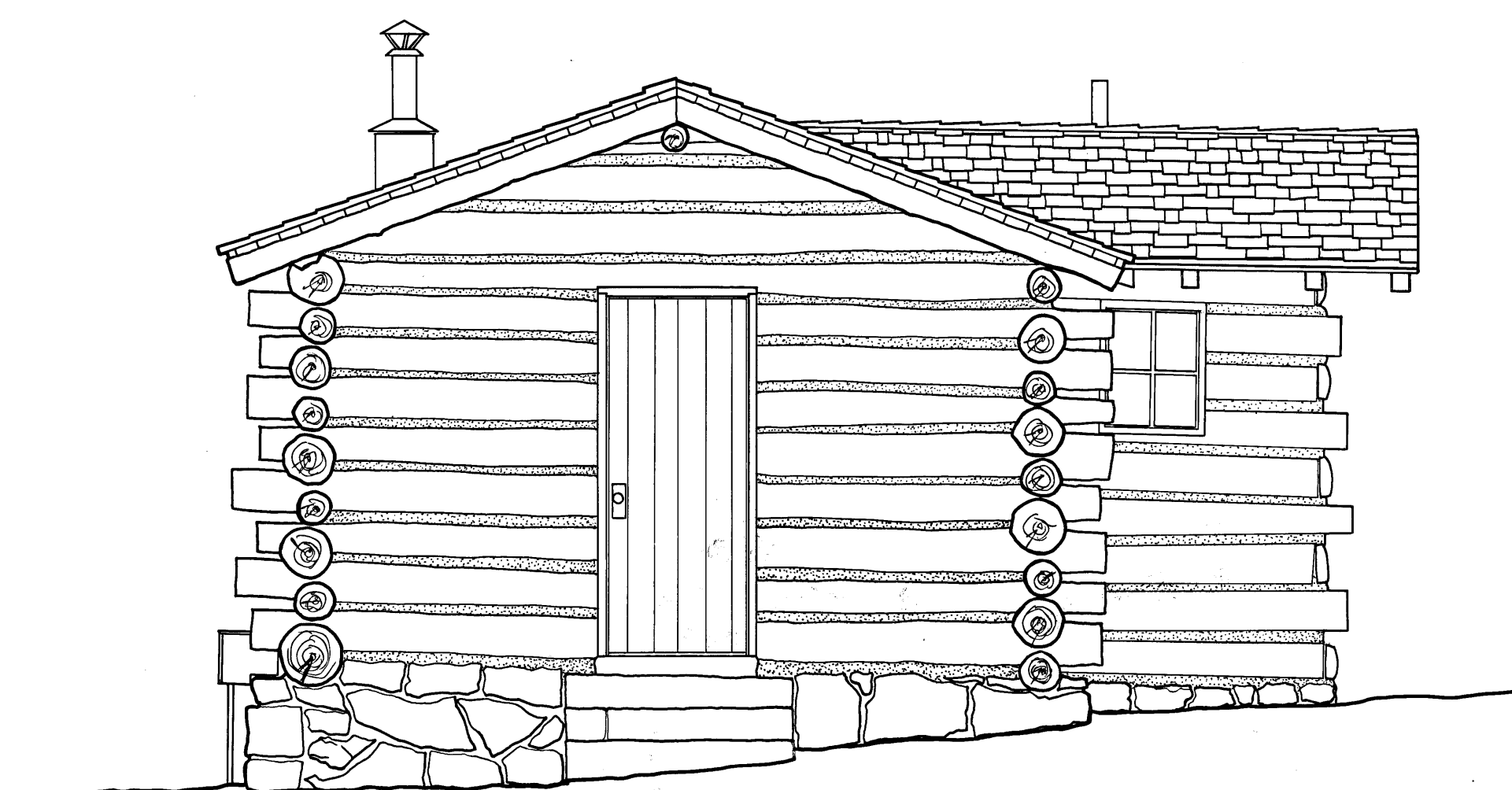
SOUTH ELEVATION
