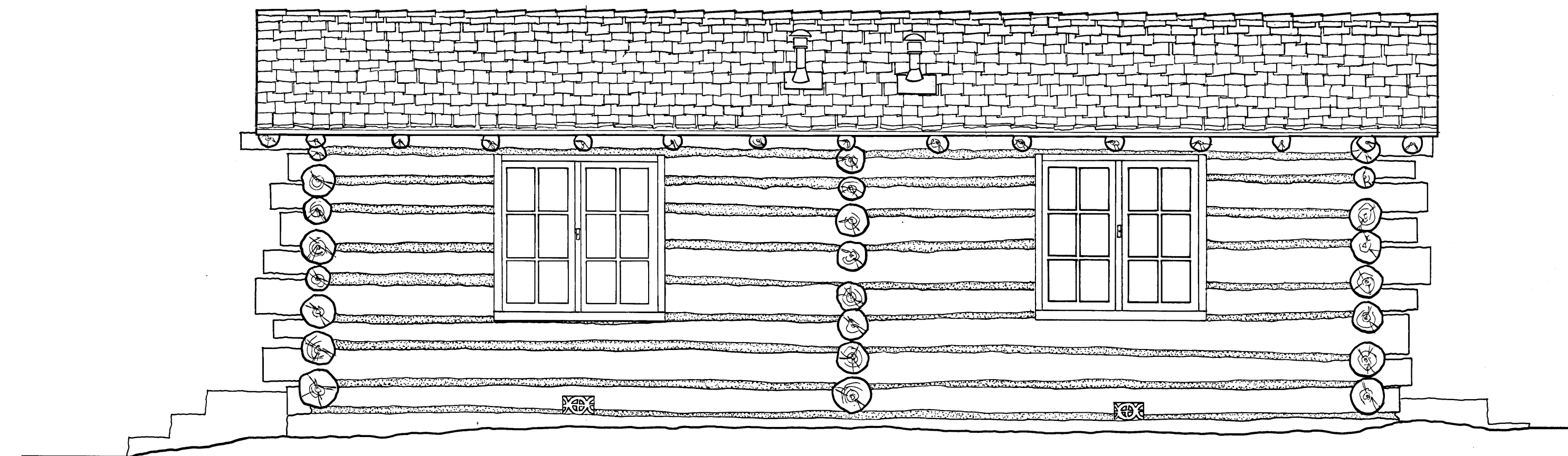
EAST ELEVATION
