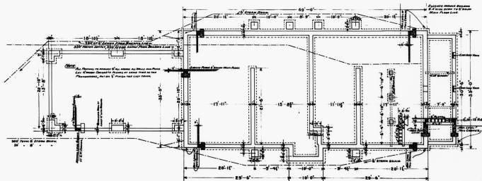
FOUNDATION PLAN. SCALE 1/4" = 1'-0"
