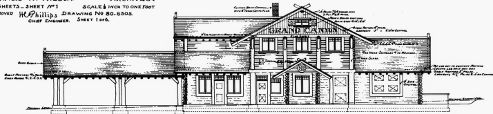
FRONT ELEVATION
