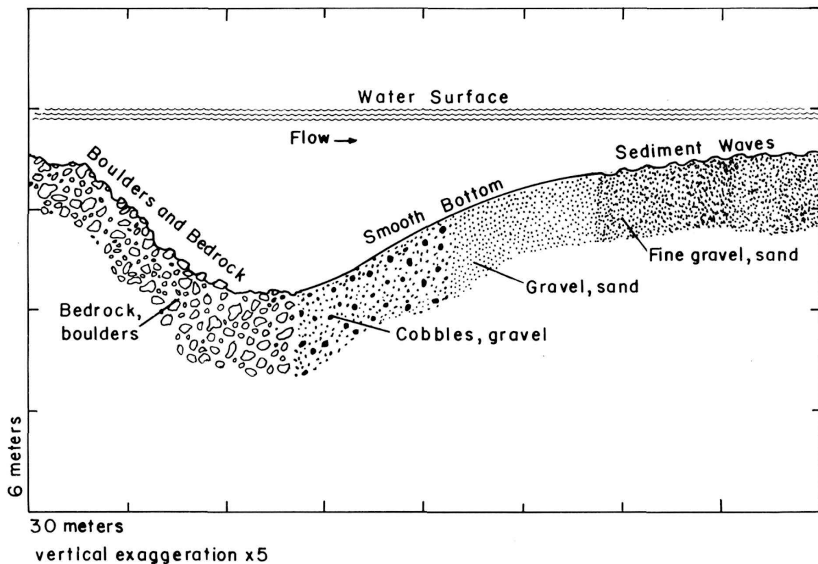
Figure 3. Generalized scour-hole profile, location of side-scan sonar patterns, and bed material.
