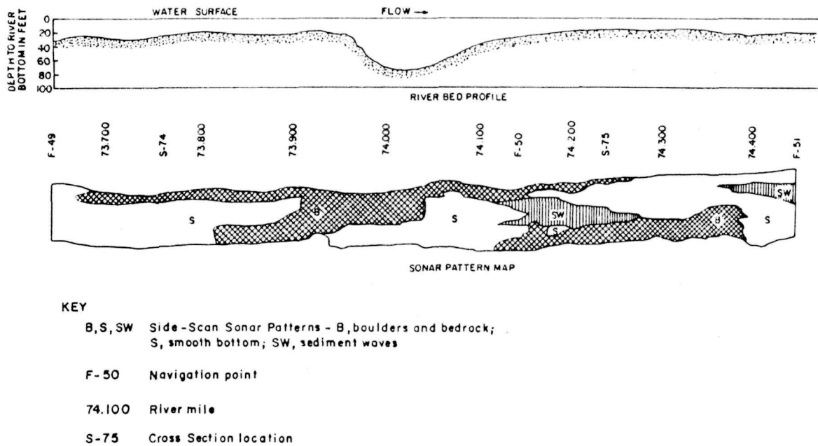
Figure 4. Example of a sonar-pattern map of reach F49F51.
