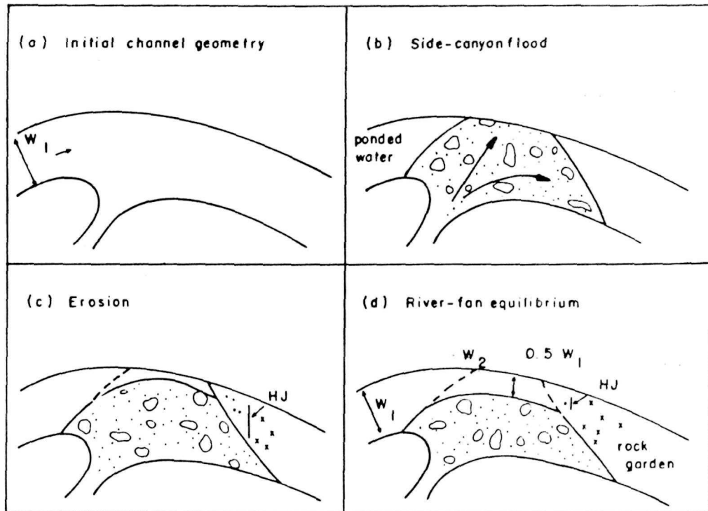
Figure 6. Processes involved in contouring the river channel at rapids.
