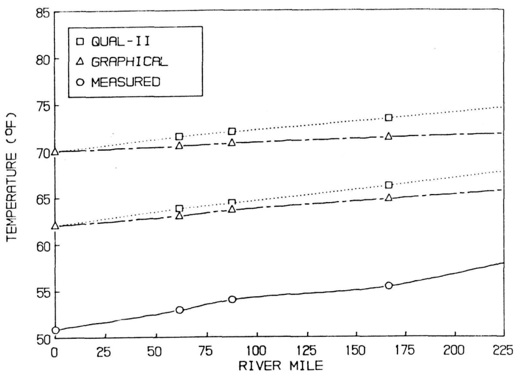
Figure 3. Average modeled (Graphical and Qual-II models) and measured August Colorado River temperature (degrees F).
