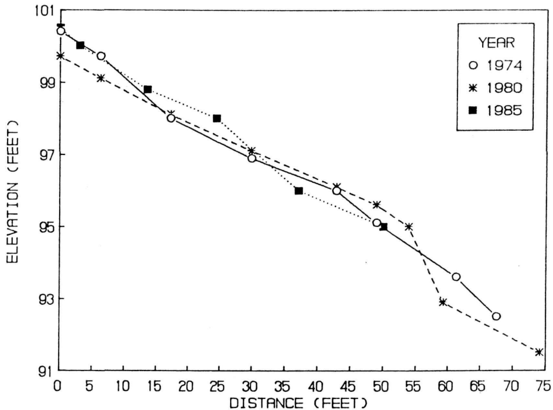
Figure 2. Plotted profile of Nankoweap Beach (RM 53.0R)
