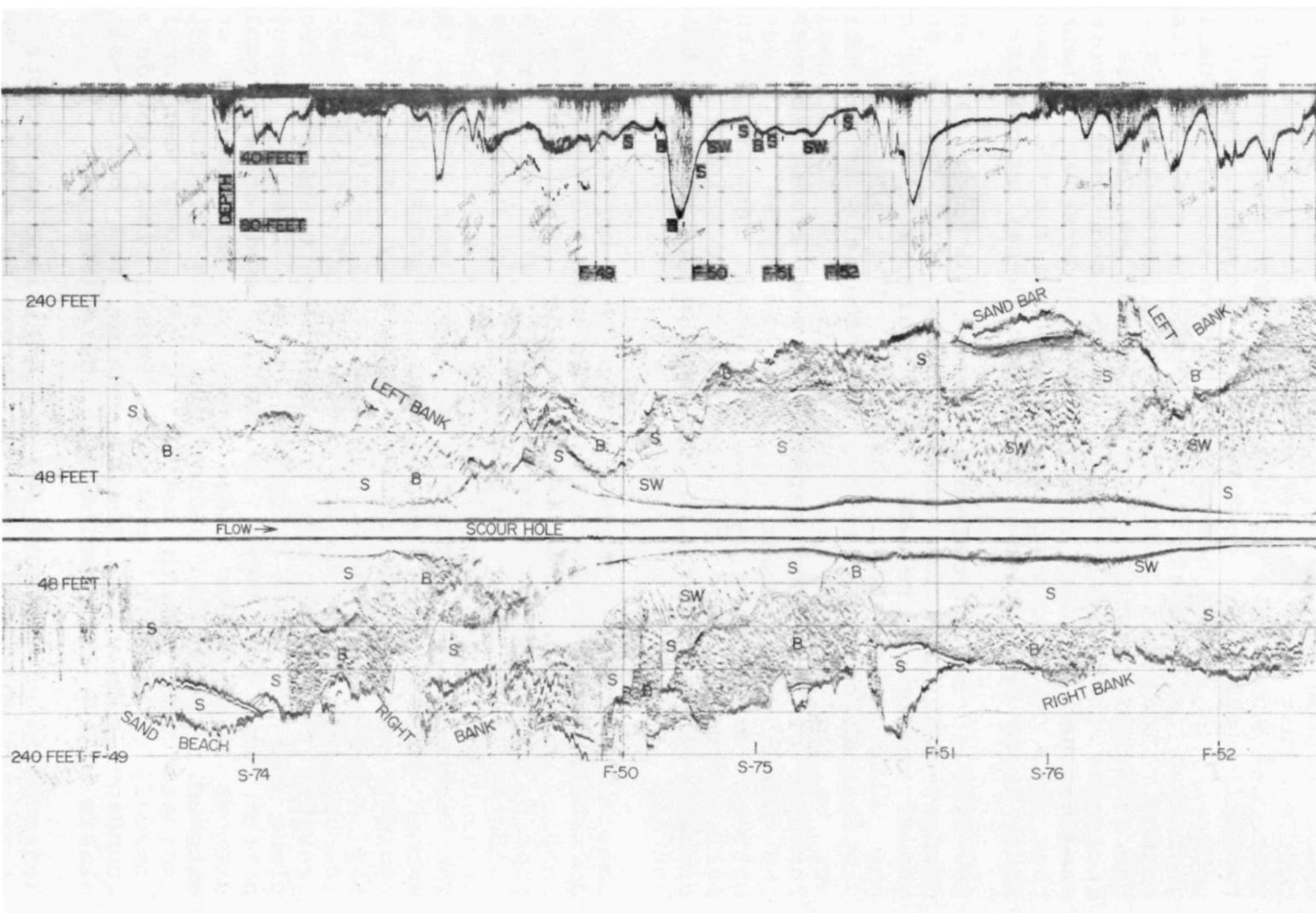
Figure 2. Uncorrected side-scan sonar and Fathometer charts.
