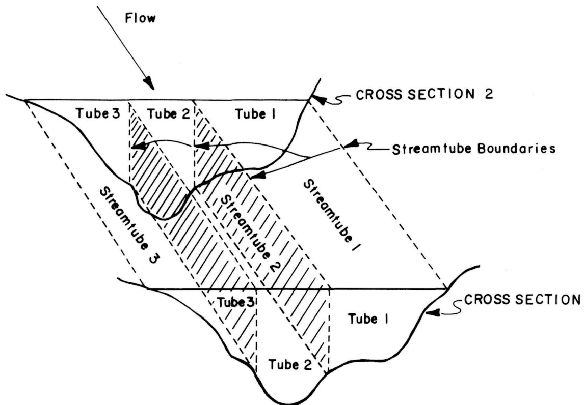
Figure 1. Three-dimensional plot of a channel with three streamtubes.
