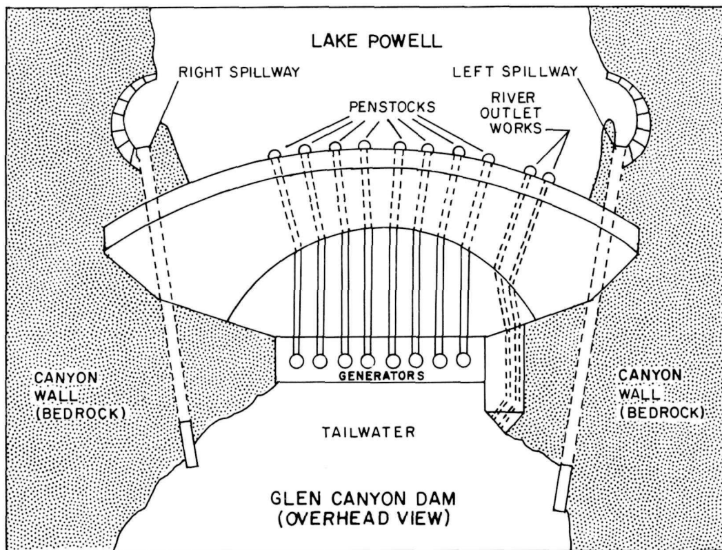
Figure 1a. Overhead view of Glen Canyon Dam.
