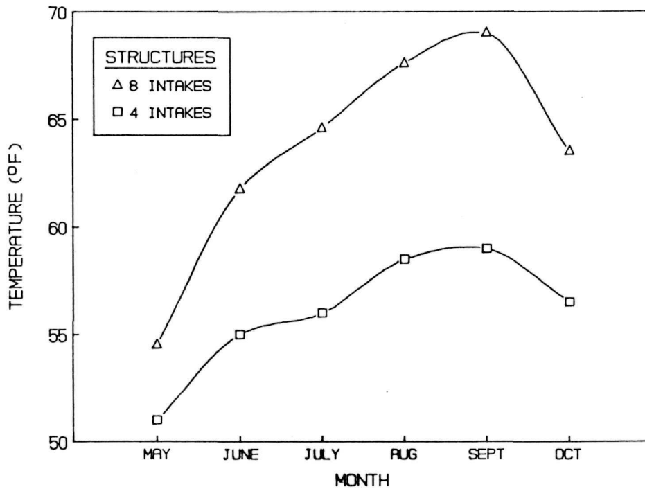
Figure 2. Predicted release temperatures from Glen Canyon Dam for eight and four multiple-level intake structures.
