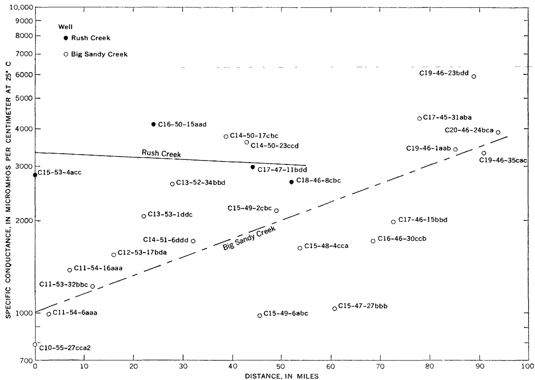
FIGURE 9.—Change in specific conductance downstream along Big Sandy Creek and along Rush Creek.
