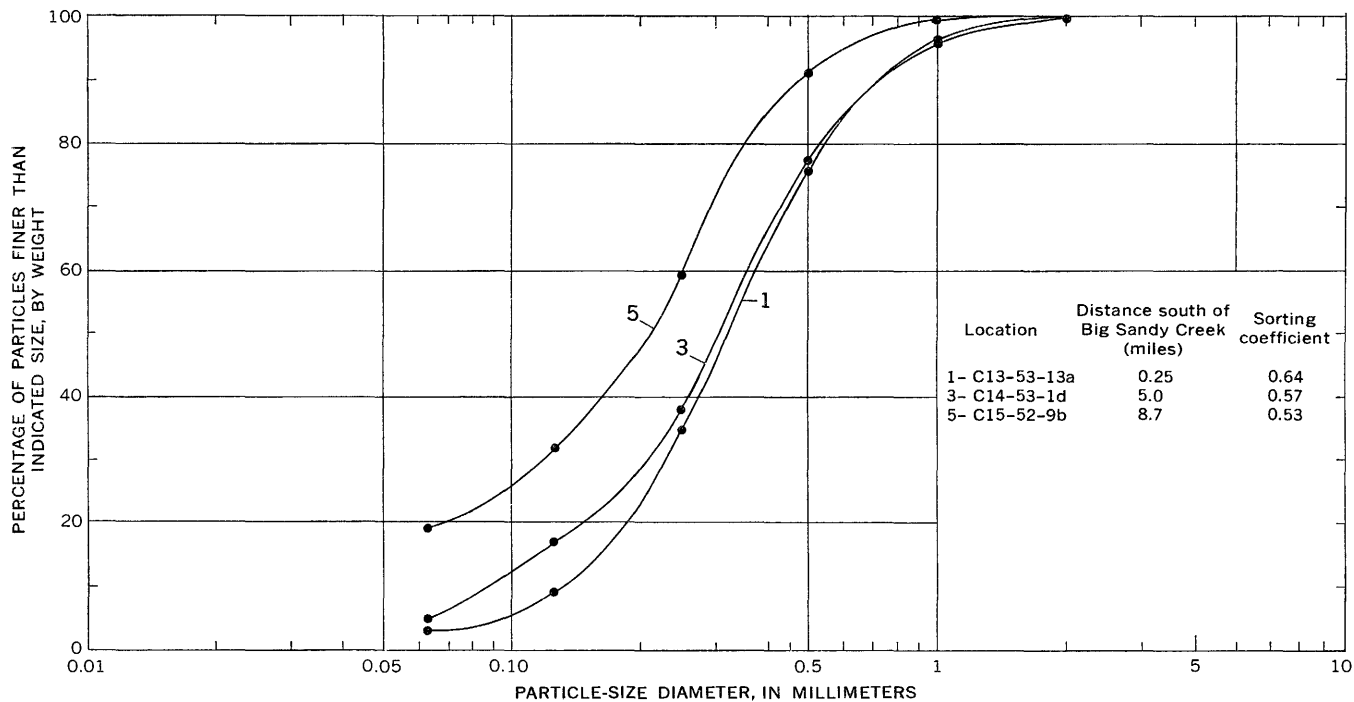
FIGURE 5.—Particle-size distribution curves of dune sand south of Big Sandy Creek.
