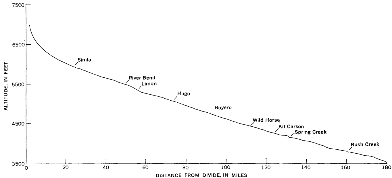
FIGURE 4.—Profile of Big Sandy Creek.
