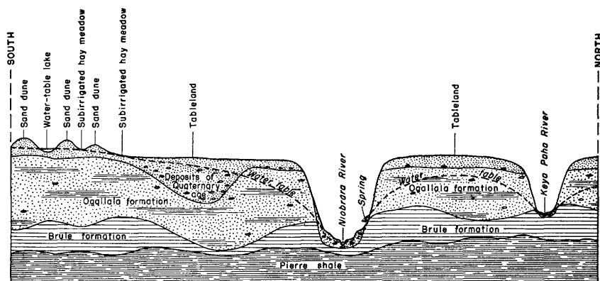
FIGURE 24.—Schematic cross section of the lower Niobrara River basin a few miles east of the mouth of Minnechaduzza Creek.
