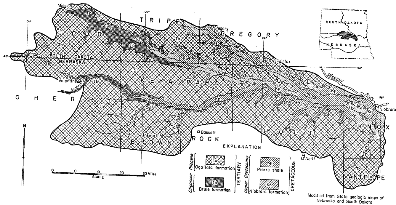
FIGURE 23.—Map showing the areal distribution of Cretaceous and Tertiary rocks in the lower Niobrara River basin and in the Ponca Creek basin.
