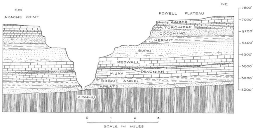
TEXT-FIGURE 25.—Cross-section showing the profile and sequence of rocks in the Grand Canyon at approximately Mile 119. The profile of the canyon in this area is dominated by the broad flat Esplanade Terrace which is carved on top of the Supai Formation. The thick Hermit Shale has eroded back from the rim of the inner gorge.
