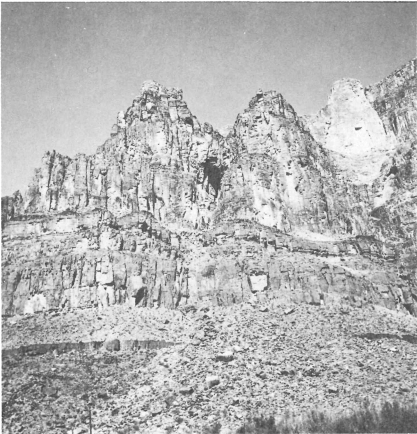
TEXT-FIGURE 91.—Bat Cave and abandoned cable anchorage at Mile 265.9. Bat guano was mined from the large cave shown in the central part of the picture and was transported by cable across the river and up to the South Rim.
