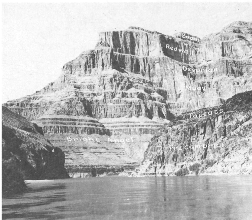
TEXT-FIGURE 89.—The canyon profile at Mile 256. The Redwall Limestone forms the uppermost bold cliff and is underlain by the well-bedded Devonian limestone and the thick sequence of poorly defined cliffs of the Muav Formation. The Bright Angel Shale forms the slopes visible downstream through the V-shaped gorge. The contact between the Precambrian metamorphic rocks and the Tapeats Sandstone is several feet above river level.
