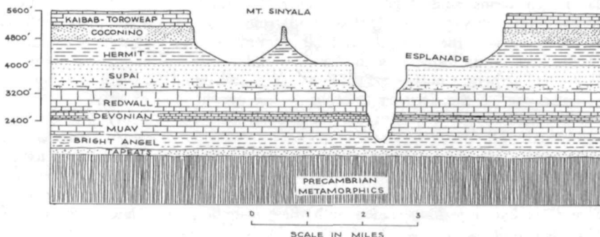
TEXT-FIGURE 43.—Cross-section across the Grand Canyon near Havasu Creek. The profile of the canyon is divisible into an outer rim held by the Kaibab and Toroweap formation, the broad Esplanade on top of the Supai Formation, and the inner gorge carved into the lower Paleozoic formations.
