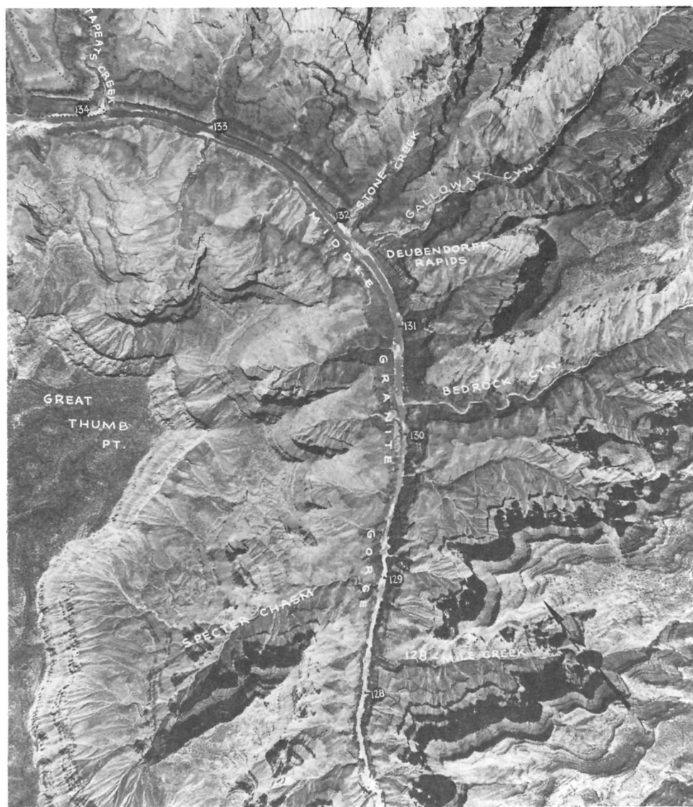
TEXT-FIGURE 31.—Vertical aerial photograph of the Colorado River from Mile 128 to Mile 134 in Middle Granite Gorge.
