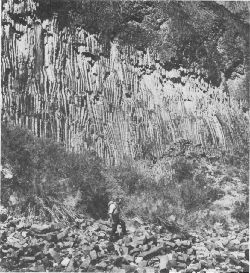
TEXT-FIGURE 61.—Columnar jointing developed in intracanyon flows at Mile 186.5, resulting from contraction of the lava as it cooled.
