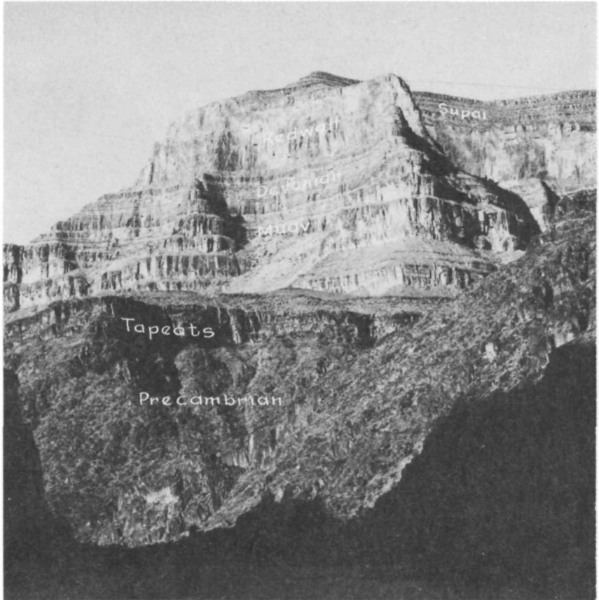
TEXT-FIGURE 78.—View of Lower Granite Gorge seen from Mile 225. The Precambrian metamorphic rocks here form the somber rugged V-shaped gorge which contrasts sharply with stratified formations above. The Esplanade is the even surface on the skyline.
