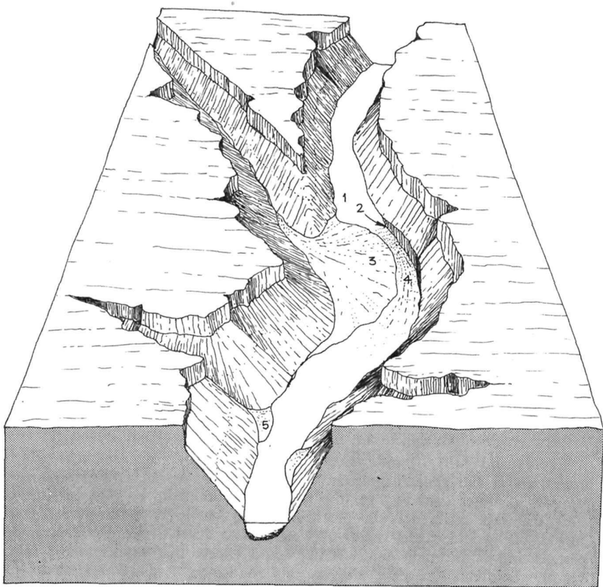
TEXT-FIGURE 14.—Diagram showing the origin of the rapids in the Colorado River. Broad fans of coarse debris accumulate at the mouths of steep tributaries and obstruct the flow of the main river. 1. quiet water; 2. eroded face; 3. and 5. debris fans; 4. rapids.
