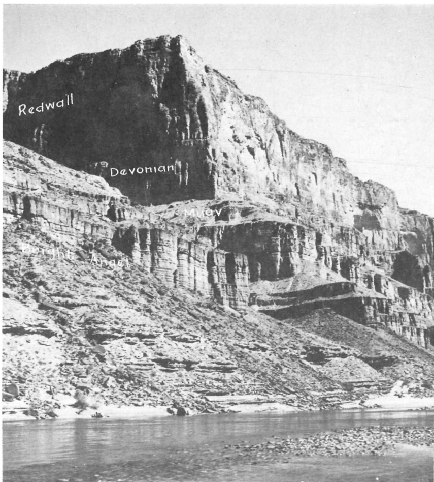
TEXT-FIGURE 30.—Bright Angel Shale is exposed near river level and forms the steep slope ascending to the base of the Muav and Redwall formations at Mile 122.
