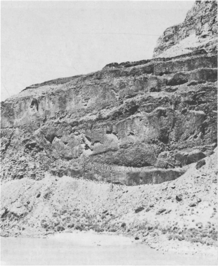
TEXT-FIGURE 59.—A cross-section of a lava-buried channel through which the Colorado River formerly flowed. The lava fill caused the river to excavate a new channel and displaced the canyon to the left around a meander bend. For scale, the black dot in the center of the sand bar in the foreground is a large rubber raft.
