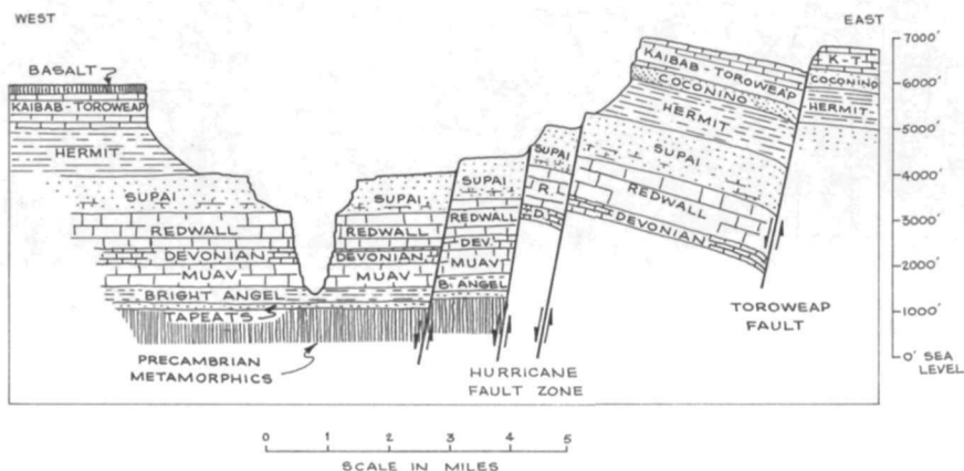
TEXT-FIGURE 72.—Cross-section across the western Grand Canyon near Mile 210.
