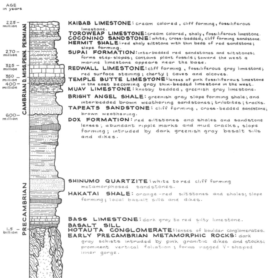
TEXT-FIGURE 4.—Sequence of rock formations exposed in the Grand Canyon.
