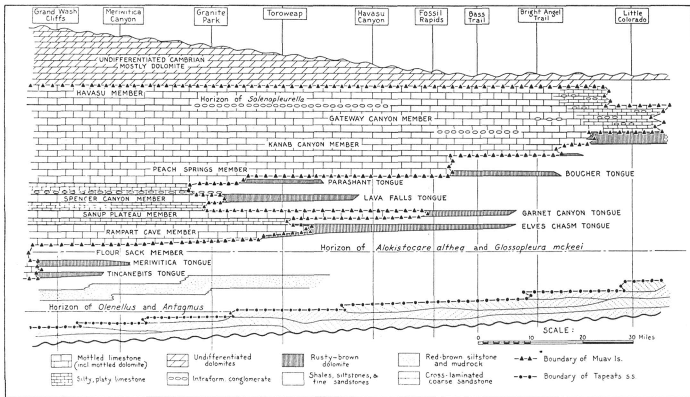
TEXT-FIGURE 47.—Diagrammatic section of Cambrian rocks seen in the western Grand Canyon between Grand Wash Cliffs, on the west, and Phantom Ranch (Bright Angel Trail), on the east. Gradual change of Muav Limestone in the west into Bright Angel Shale toward the east is evident in the interfingering of the two formations. Time planes are horizontal, as shown by trilobite zones. Actual thickness changes from approximately 1,500 feet in the west to only approximately 800 feet in the east. (From McKee and Resser, 1945, Fig. 1)
