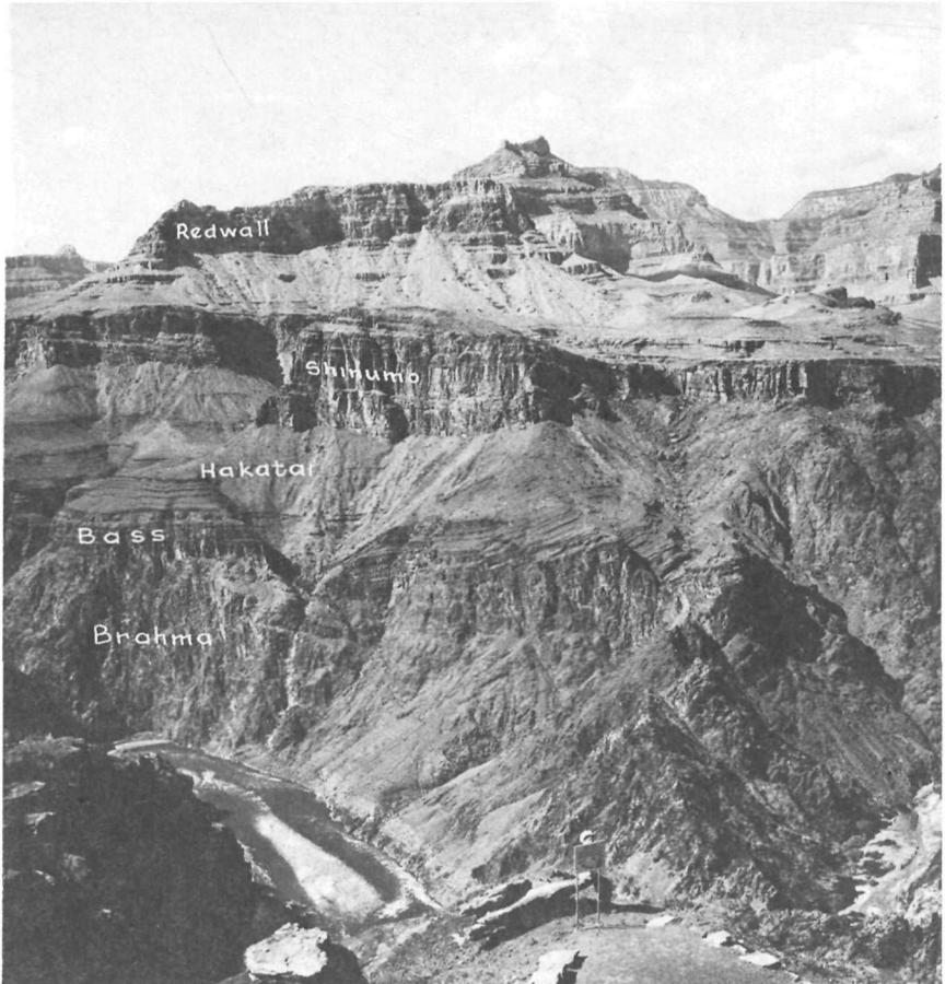
TEXT-FIGURE 10.—View of the Granite Gorge from The Tipoff on the Kaibab Trail. The rugged exposures of Precambrian metamorphic rocks are overlain here by the tilted red strata of the Precambrian Grand Canyon Series. Bass, Hakatai and Shinumo formations are exposed beneath Cheops Pyramid. Under the Paleozoic rocks the Hakatai Shale forms the slope below the Shinumo cliff and above the small cliff of Bass Limestone. The gravel bars in the center of the Colorado River are a result of overloading of the river with debris brought in by Bright Angel Creek. Bright Angel Trail follows the shadowed bank near river in the lower left of the photograph.
