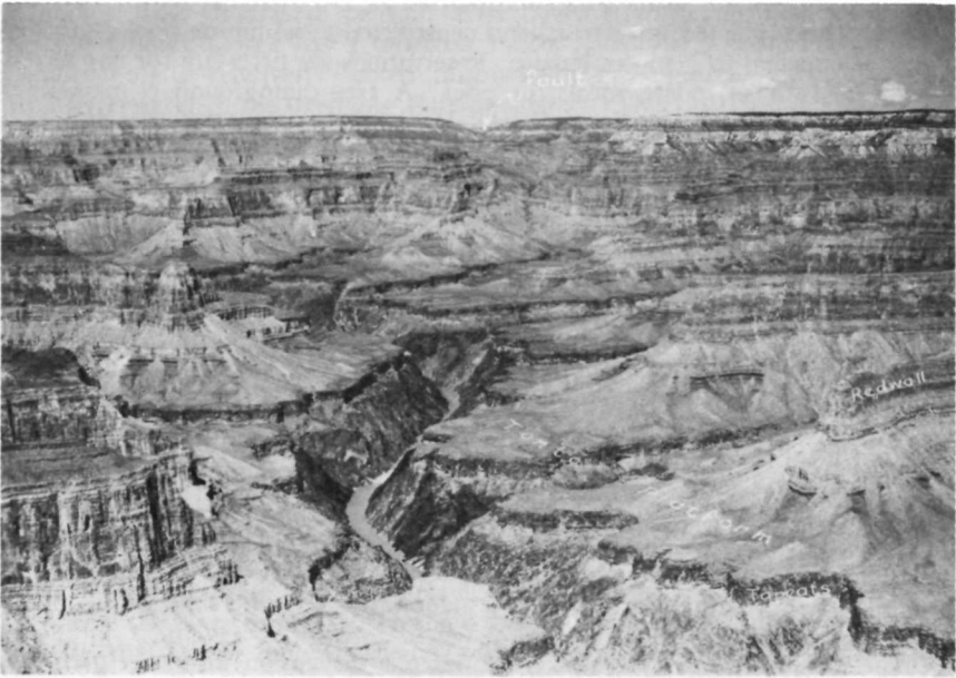
TEXT-FIGURE 13.—View of Grand Canyon, northwest from Pima Point on the South Rim, showing the inner gorge, Tonto Platform and the overlying sequence of cliffs of Paleozoic rocks near Mile 93. The Mauv Fault can be seen in the center background as an offset in the Coconino and Kaibab formations. Boucher Rapids at Mile 96 is near the bend in the river visible in the inner gorge.
