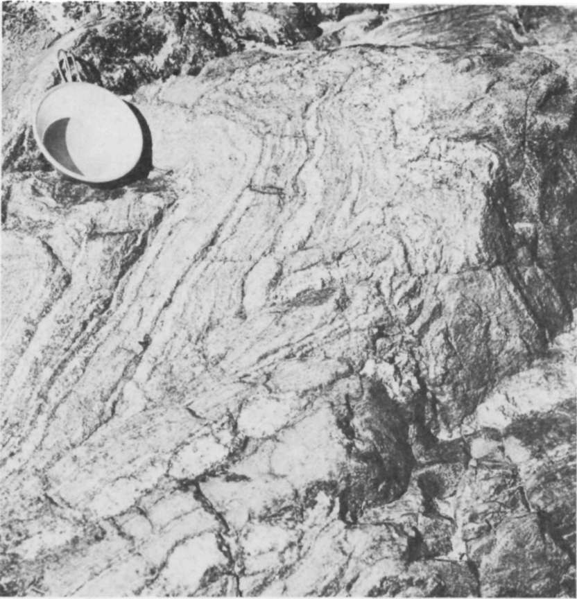
TEXT-FIGURE 19.—Exposure of gneiss in Granite Gorge at Mile 100. The crinkled and crumpled bands express the nature of deformation.
