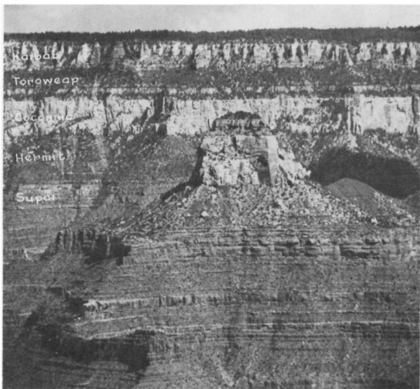
TEXT-FIGURE 6.—Buddha Temple and the North Rim as viewed from the Kaibab Trail. The resistant rock which holds up the pyramid-shaped pinnacle of Buddha Temple is the Coconino Sandstone which also forms the white second cliff below the rim of the canyon on the north rim. The small alternating cliffs and slopes in the red sandstones below are the Supai Formation.
