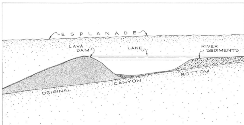
TEXT-FIGURE 55.—Diagram showing the relationships of lava dams and impounded lakes in the western Grand Canyon region.
