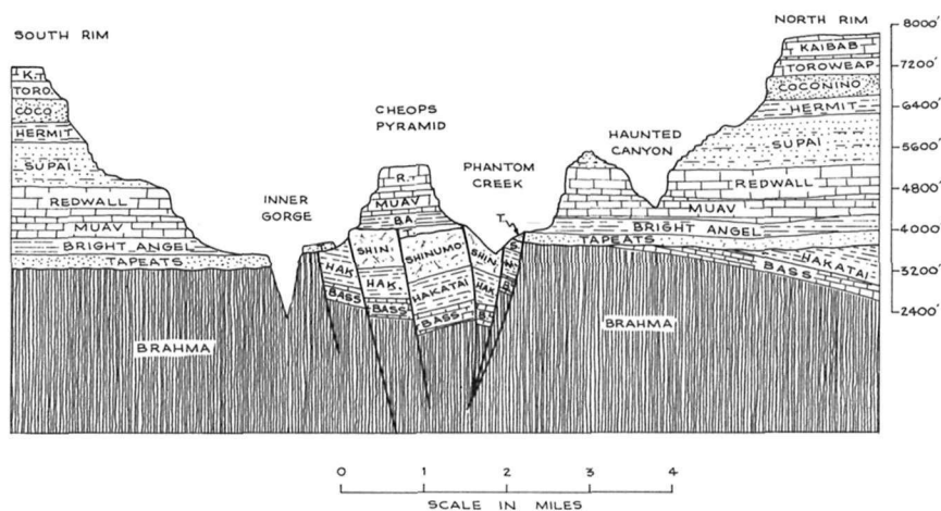
TEXT-FIGURE 3.—Cross-section from El Tovar Hotel northward through Cheops Pyramid. The three major rock divisions are clearly shown including the upper sequence of horizontal Paleozoic rocks which form the major walls of the canyon, the tilted Grand Canyon Series beneath Cheops Pyramid, and the old Precambrian metamorphic and igneous rocks in Granite Gorge.
