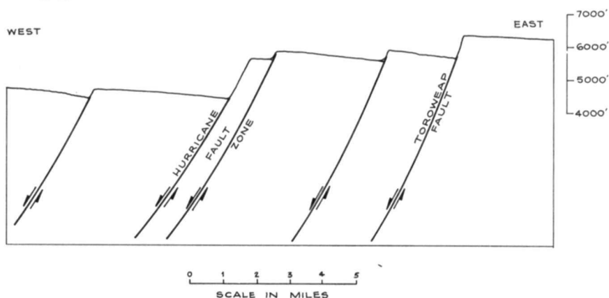
TEXT-FIGURE 68.—Cross-section showing the displacement along the Hurricane Fault zone near Mile 191.
