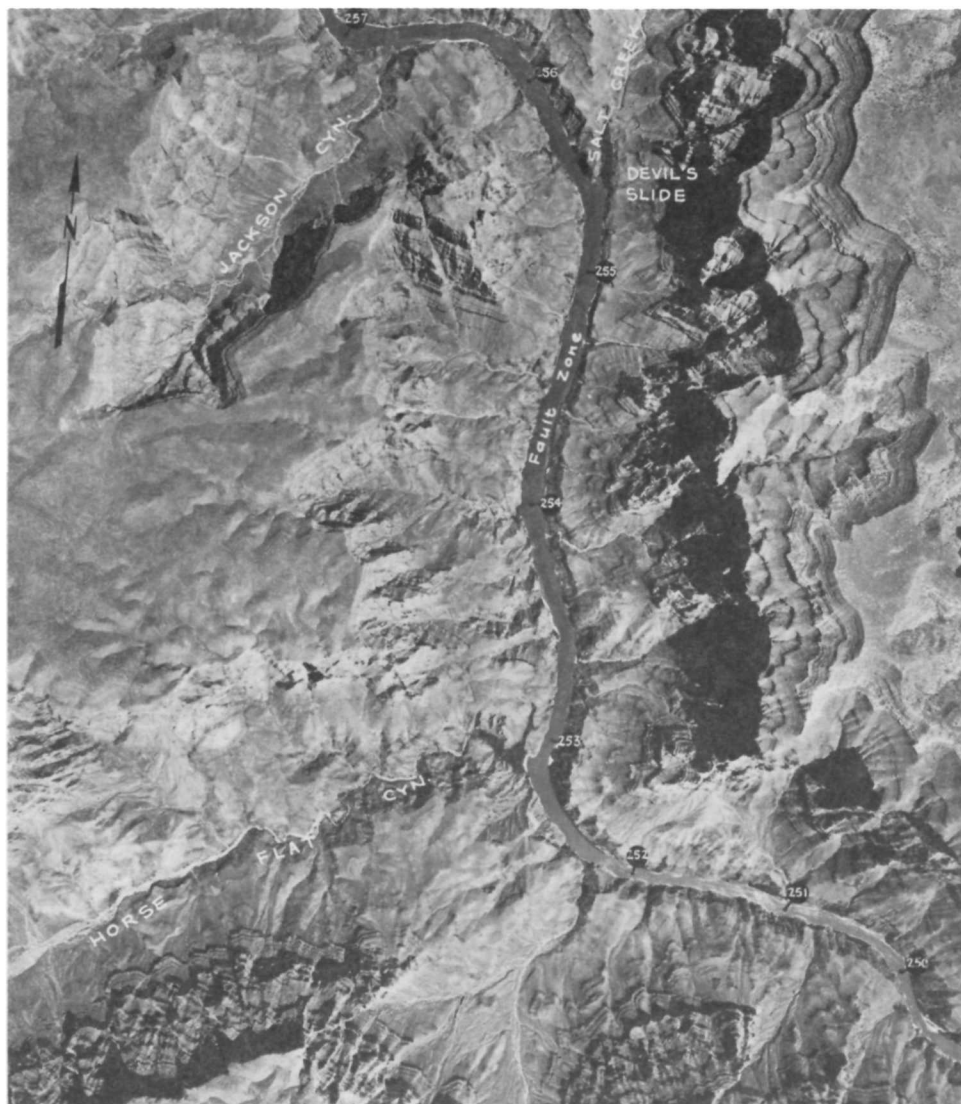
TEXT-FIGURE 87.—Vertical aerial photograph of the Colorado River from Mile 250 to Mile 257.
