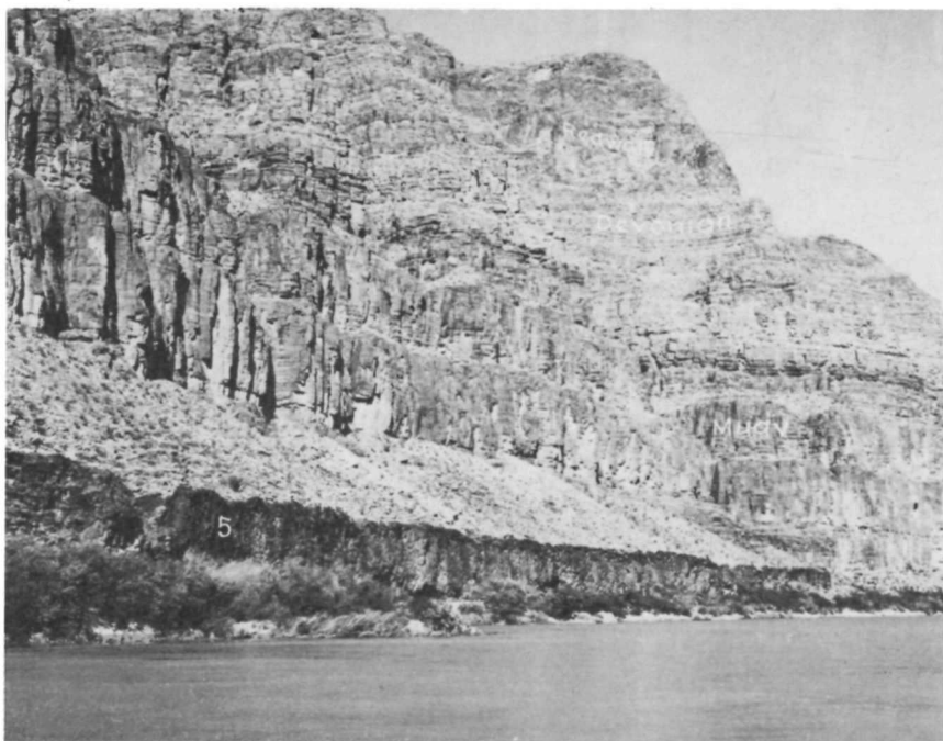
TEXT-FIGURE 70.—A remnant of a younger intracanyon Flow 5 at Mile 197 adhering to the canyon wall 50 to 60 feet above river level. The Muav Limestone forms a series of cliffs up to the Redwall Formation on the horizon. The thin uniformly bedded strata are the Devonian Limestone.
