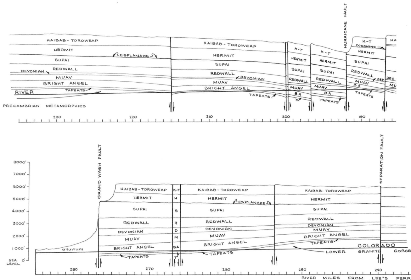
TEXT-FIGURE 11.—Cross-section showing the rock sequence along the river from Phantom Ranch to Grand Wash Cliffs. The profile is along the north or right wall of the canyon.
