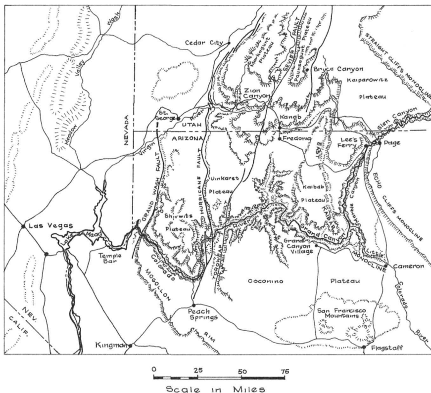
TEXT-FIGURE 1.—Map of the southwestern part of the Colorado Plateau showing the major features associated with the Grand Canyon. The Grand Canyon ends at Grand Wash Cliffs which is the boundary between the Colorado Plateau and the Basin and Range Province.
