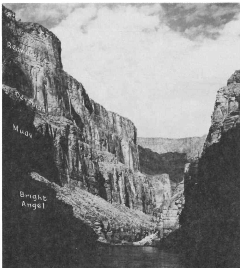
TEXT-FIGURE 41.—View looking downstream from Mile 154. The nature of the inner gorge below the Esplanade Platform and the outer rim of the canyon can be seen ahead. The Muav Limestone becomes very thick in this area and holds up a sequence of several cliffs between the slopes of the Bright Angel Shale and the prominent Redwall Cliff.
