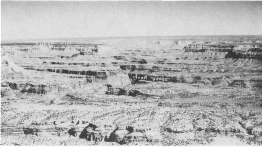
TEXT-FIGURE 48.—View of Grand Canyon from above Mile 176 looking toward the east. The broad platform of the Esplanade, the outer rim carved on the Kaibab-Toroweap, and the inner gorge below show the typical profile of the western Grand Canyon. The Colorado River is 3,000 feet below the level of the Esplanade in the narrow gorge.
