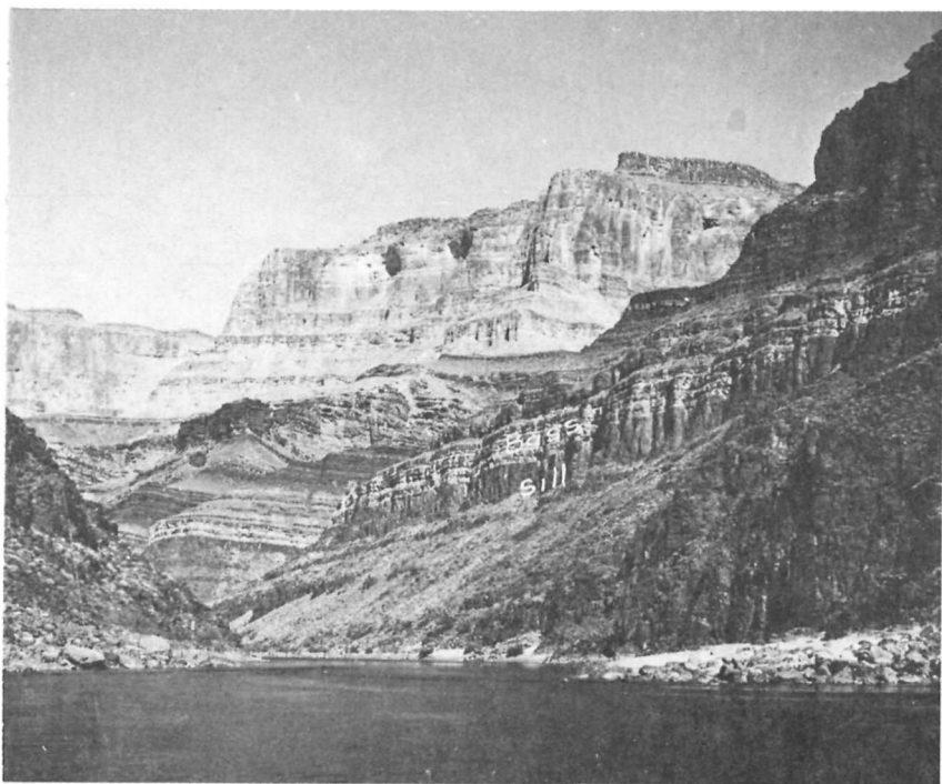
TEXT-FIGURE 32.—The Grand Canyon Series as exposed at Mile 130, downstream from Bedrock Rapids. The light-colored bedded units are bleached Bass Limestone which has been altered by injection of a large diabase sill below. Typical caverns and alcoves etched in the Redwall Limestone are visible on the skyline.
