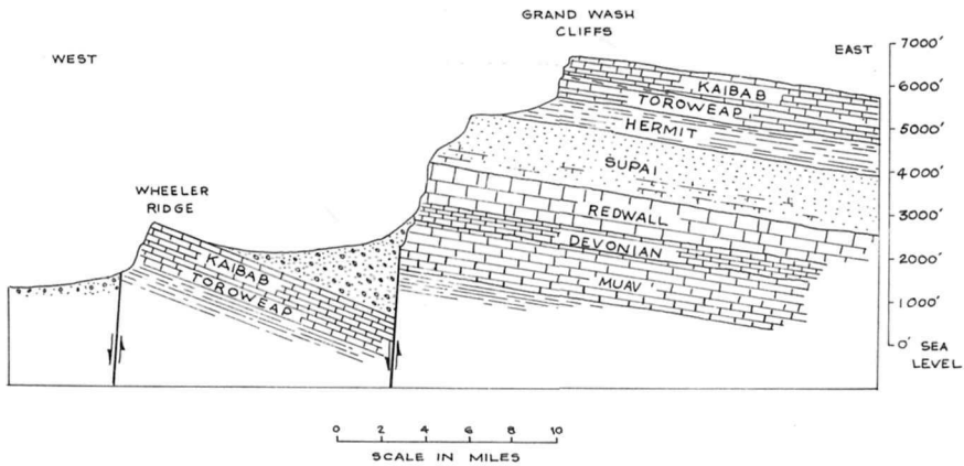
TEXT-FIGURE 96.—Cross-section across the Grand Wash Cliffs and fault zone, westward across Wheeler Ridge.
