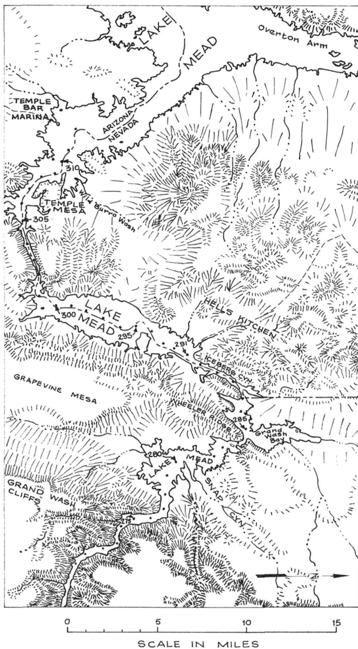
TEXT-FIGURE 98.—Map of the upper part of Lake Mead from the Grand Wash Cliffs west to near Temple Bar Landing.
