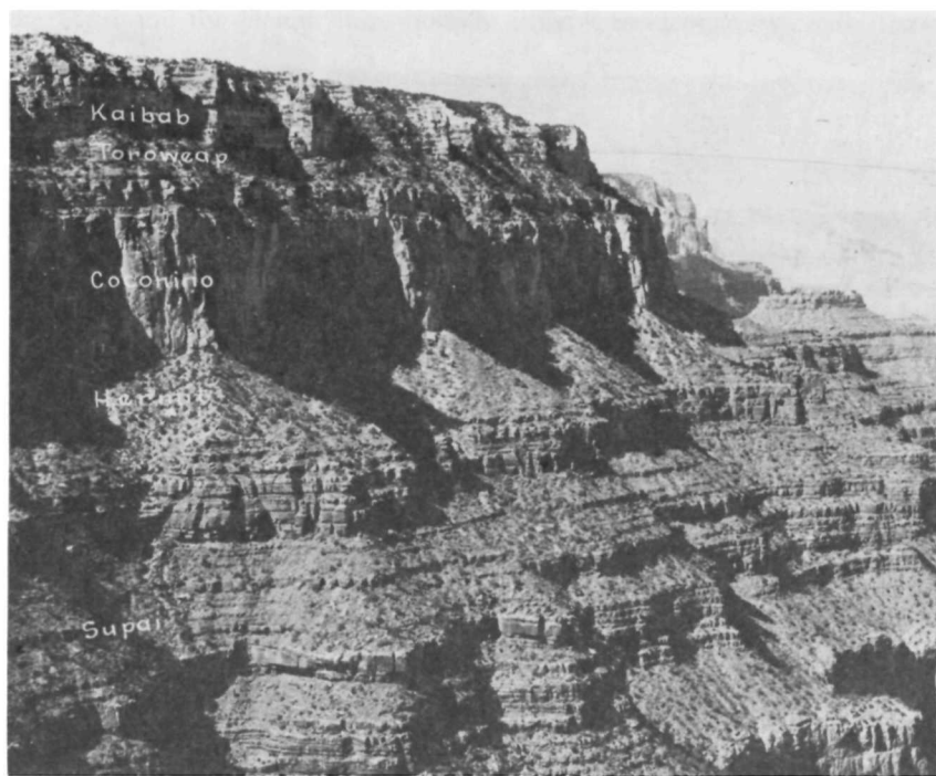
TEXT-FIGURE 5.—The Upper Paleozoic sequence exposed near the top of Kaibab Trail on the South Rim. Hermit Shale forms the slopes near the middle of the sequence of cliffs, with red Supai Formation exposed in step-like fashion below. The prominent light vertical wall above the Hermit slope is the Coconino Sandstone. Overlying broken cliffs are carved in the Kaibab and Toroweap formations.
