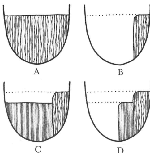
TEXT-FIGURE 52.—Diagram showing the origin of juxtaposed basalt remnants in the western Grand Canyon.
