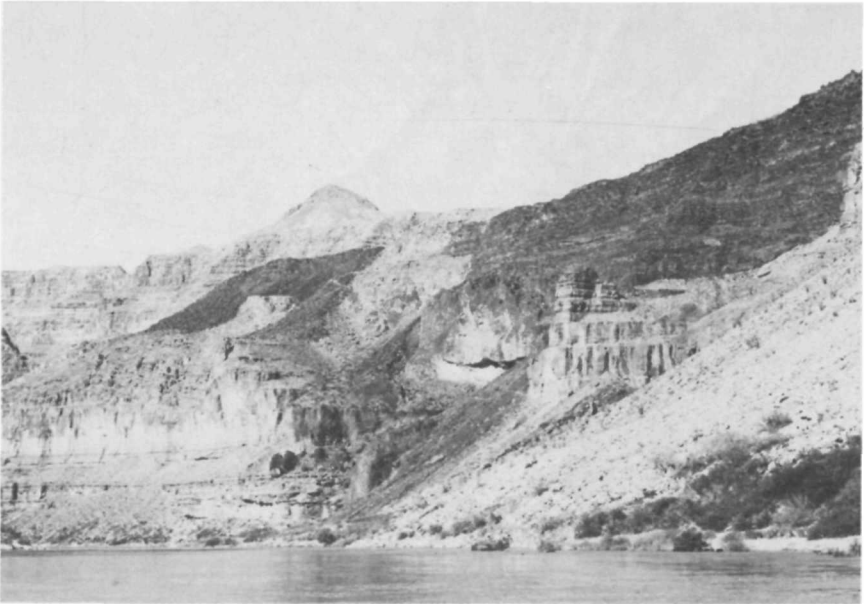
TEXT-FIGURE 63.—Whitmore Wash. The ancient tributary valley is filled with a sequence of thinly bedded lavas. It is possible to drive to the rim of the canyon at this point although the road is extremely rough and 4-wheel drive is advised. The trail leading up to the canyon rim can be seen near the center of the picture. Segments of a hose used to refuel jet boats coming up the river can be seen dangling from the rim near the lip of the basalts and on down past the "castle" to the river below.
