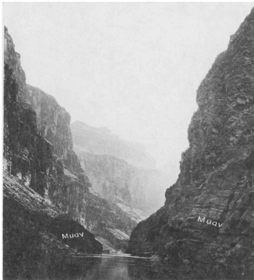
TEXT-FIGURE 39.—Small flexure in Muav Limestone developed at river level at Mile 148. This minor folding may be the result of release of confining pressure as the river removes the overlying rocks. Axes of these small folds generally are along the trend of the river channel.
