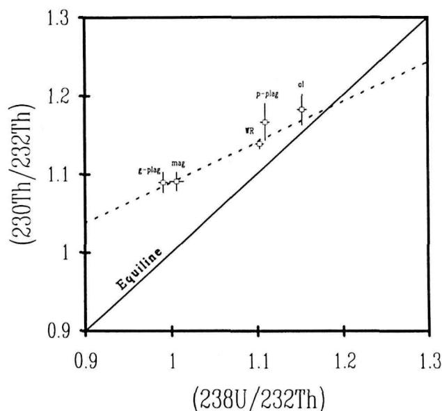
FIGURE 3— ^{230}\text{Th}/^{232}\text{Th} versus ^{238}\text{U}/^{232}\text{Th} for the Bluewater flow from the Zuni-Bandera field on the Jemez lineament in New Mexico. The isochron, shown by the dashed line, gives a 2\sigma age of 79 \text{ ka} \pm 40 \text{ ka} .
