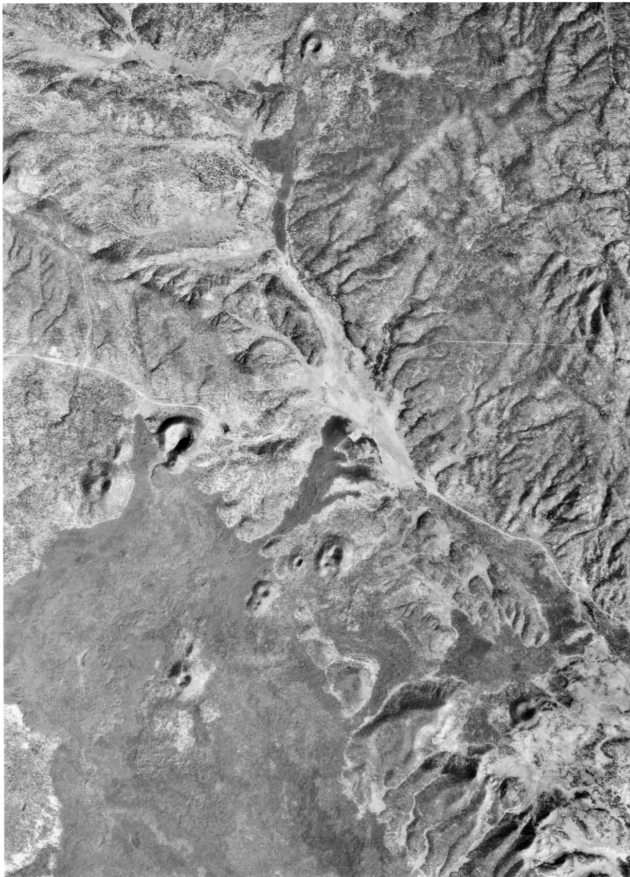
FIGURE 7a—Aerial photo showing the numerous volcanic vents near Bandera Crater.
