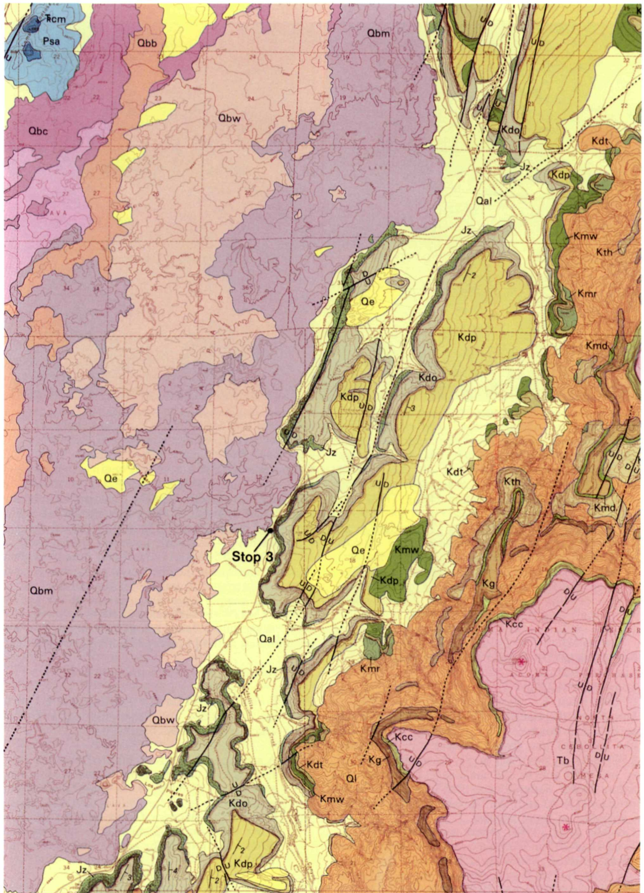
FIGURE 5b—This portion of the geologic map of Maxwell (1986) covers essentially the same area as the photograph in Fig. 5a.
