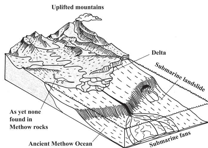
Figure 18. Sketch showing Cretaceous setting for accumulation of sediments that became rocks of Methow Ocean and younger deposits (after a drawing by David G. Howell).
