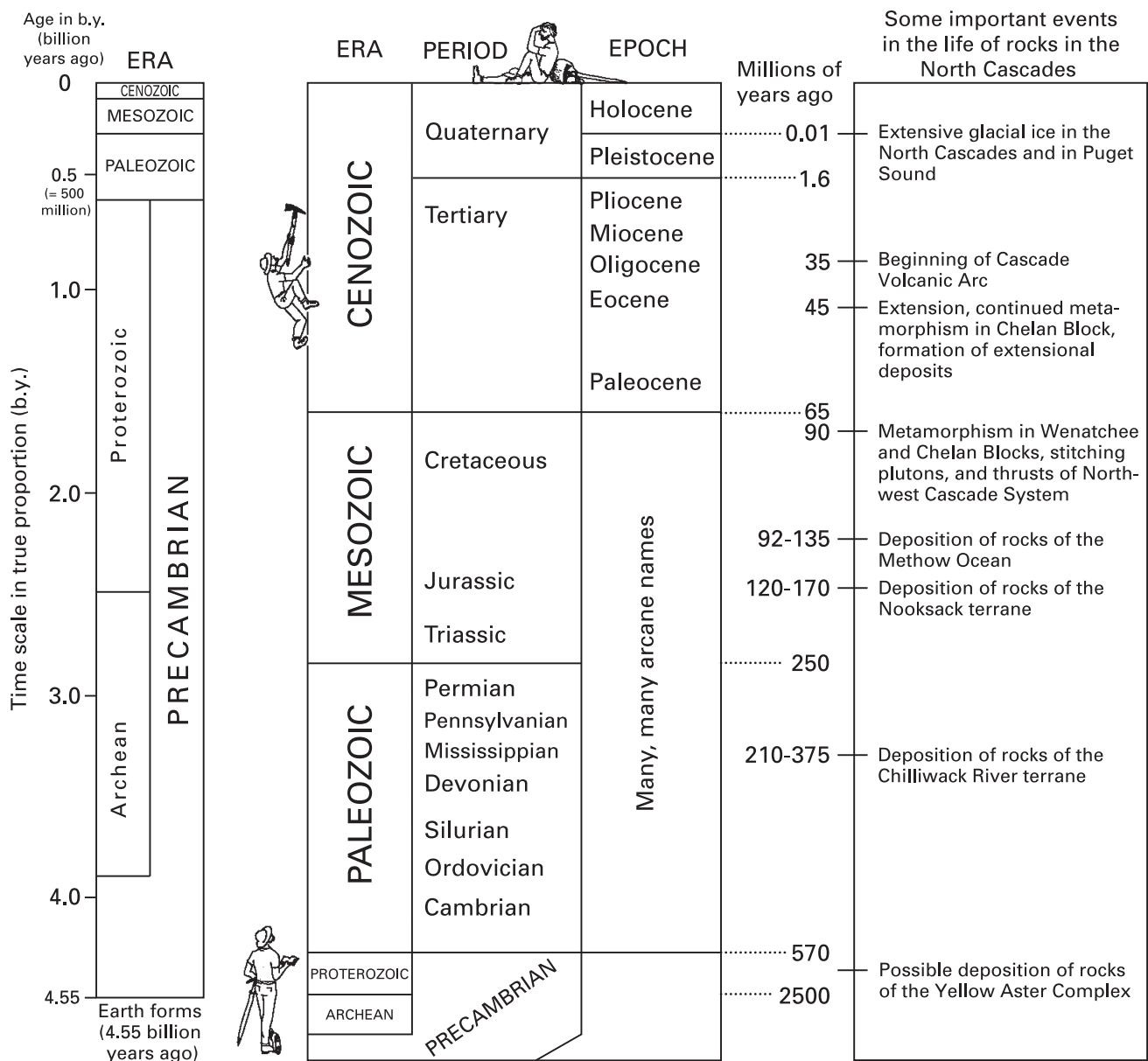
Figure 6. Geologic time scales relative to some geologic events in North Cascades, Washington.
