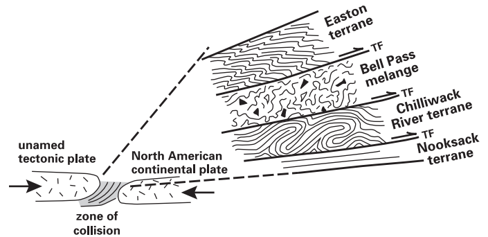
Figure 11. Sketch of cross section showing how terranes (nappes) became stacked in Northwest Cascade System along thrust faults (TF) during collision between tectonic plates. Half arrow (→) shows direction of movement along faults.
