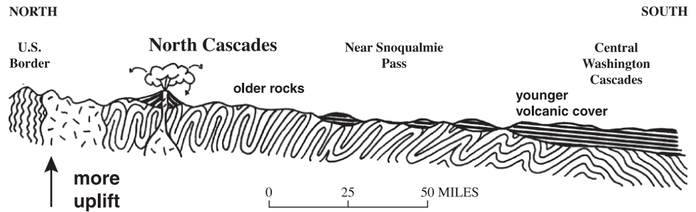
Figure 10. Sketch showing a north-south cross section of the Cascade Range in Washington. Erosion removed more of the volcanic deposits in the north than in the south, because uplift is greater in the north. Contact between volcanic deposits and underlying, folded older rocks is an angular unconformity.
