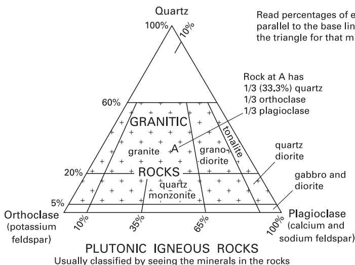
Figure 21. Ternary diagrams showing classification of igneous rocks by percent content of light-colored minerals (shown at corners of triangular diagrams). Dark minerals like biotite and hornblende are not included in percentage calculation. All rocks in patterned area of plutonic triangle can be called granitic because they resemble granite. Only some rock names are shown.
