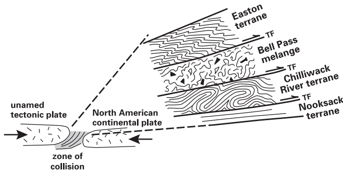
Figure 11. Sketch of cross section showing how terranes (nappes) became stacked in Northwest Cascade System along thrust faults (TF) during collision between tectonic plates. Half arrow (—>) shows direction of movement along faults.
