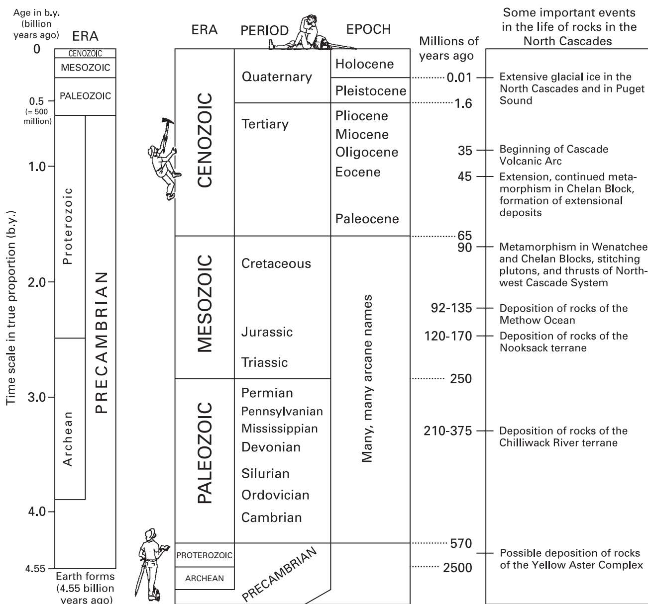
Figure 6. Geologic time scales relative to some geologic events in North Cascades, Washington.
