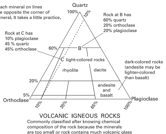
Figure 21. Ternary diagrams showing classification of igneous rocks by percent content of light-colored minerals (shown at corners of triangular diagrams). Dark minerals like biotite and hornblende are not included in percentage calculation. All rocks in patterned area of plutonic triangle can be called granitic because they resemble granite. Only some rock names are shown.
