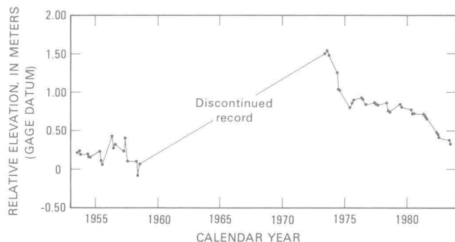
FIGURE 11.—Variation in mean elevation of the low-flow channel of Redwood Creek at the gaging station near Blue Lake (11481500). Mean streambed elevations were determined by using methods described by Hickey (1969).
