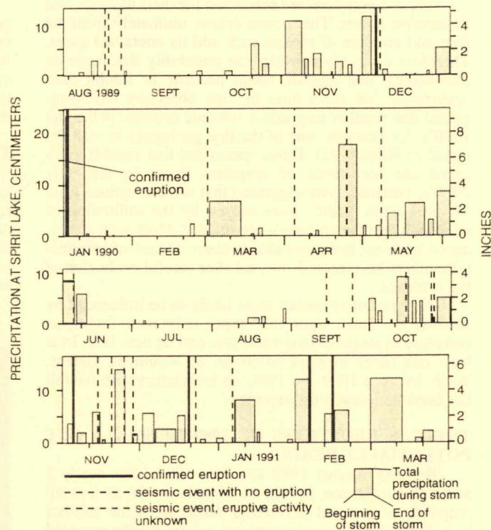
Figure 2: Timing of storms and explosion-like seismic events at Mount St. Helens, 1989-1991.
