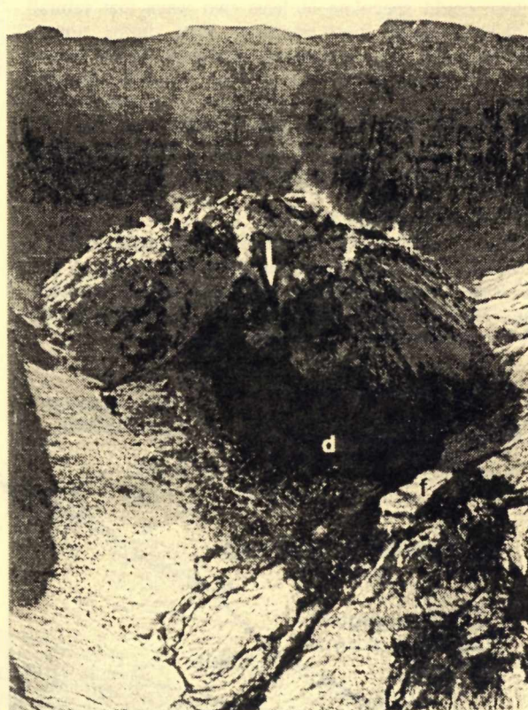
Figure 1: Mount St. Helens dome following an explosion on November 5, 1990. Eruption vent shown by white arrow. A flood channel (f) was scoured by snowmelt through the main eruption deposit (d) and was then covered by snow. Blocks that pepper the left side of the crater were ballistically ejected from the vent.
