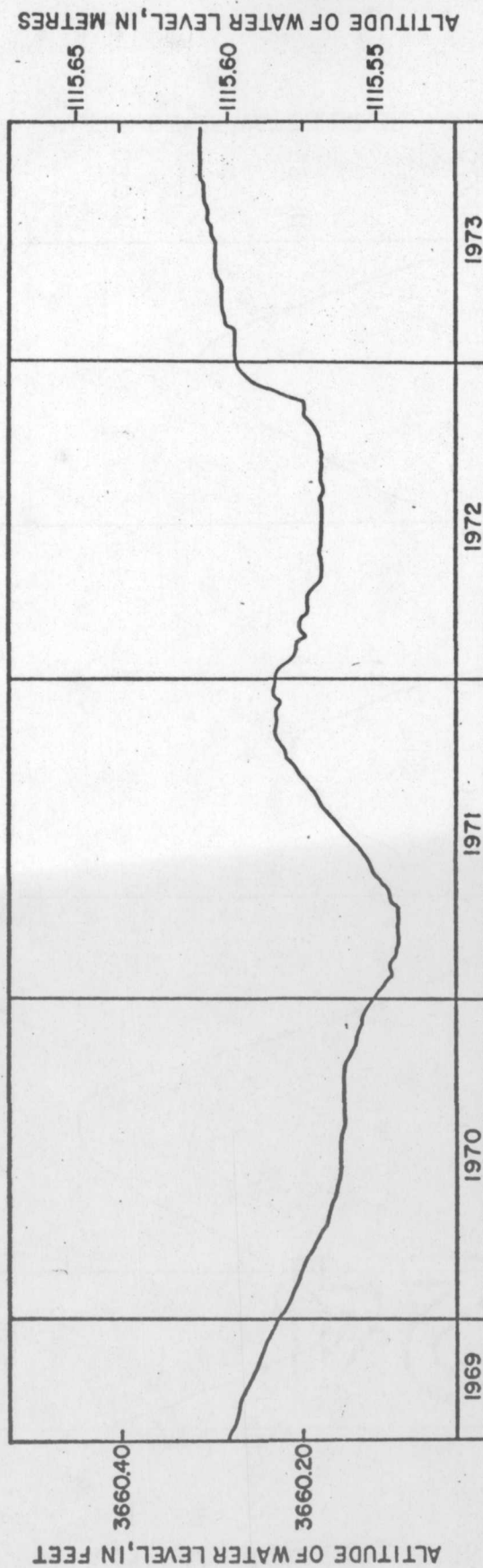
Figure 9.--Hydrograph of the Painted Grotto pool.
