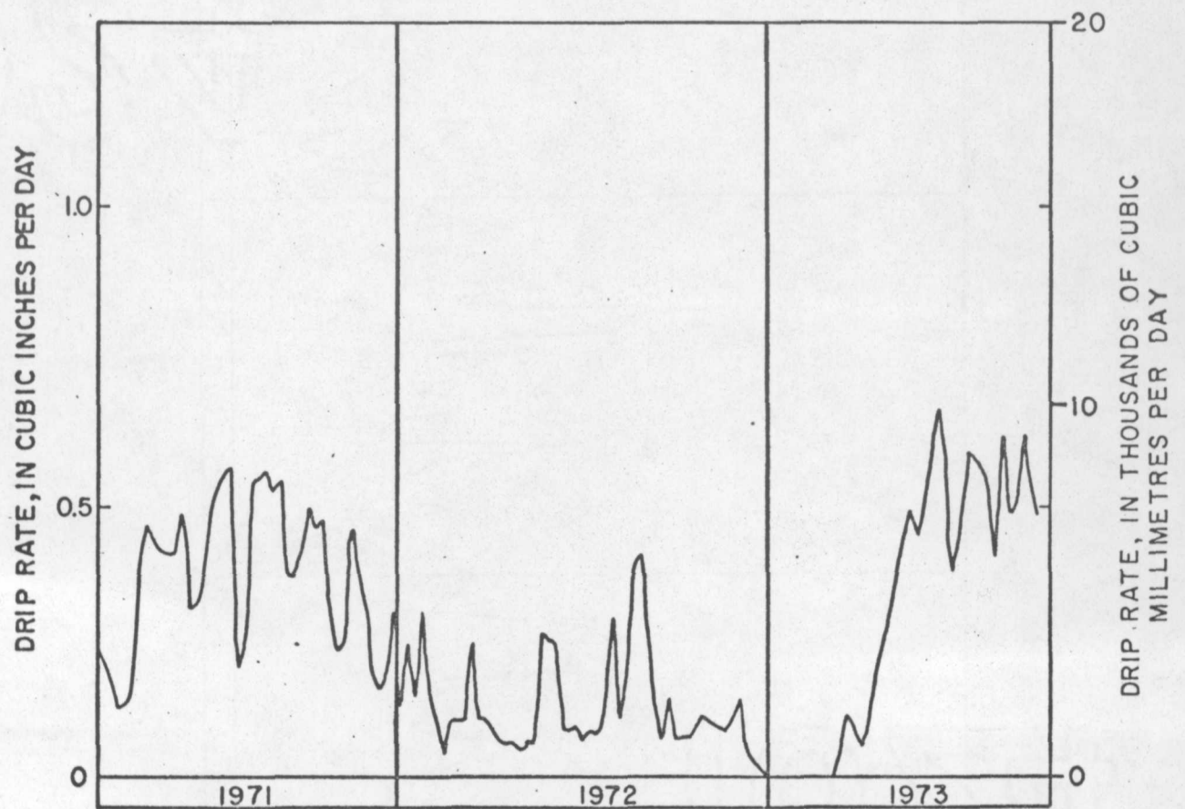
Figure 30.--Drip rate at the Baby Hippo.
