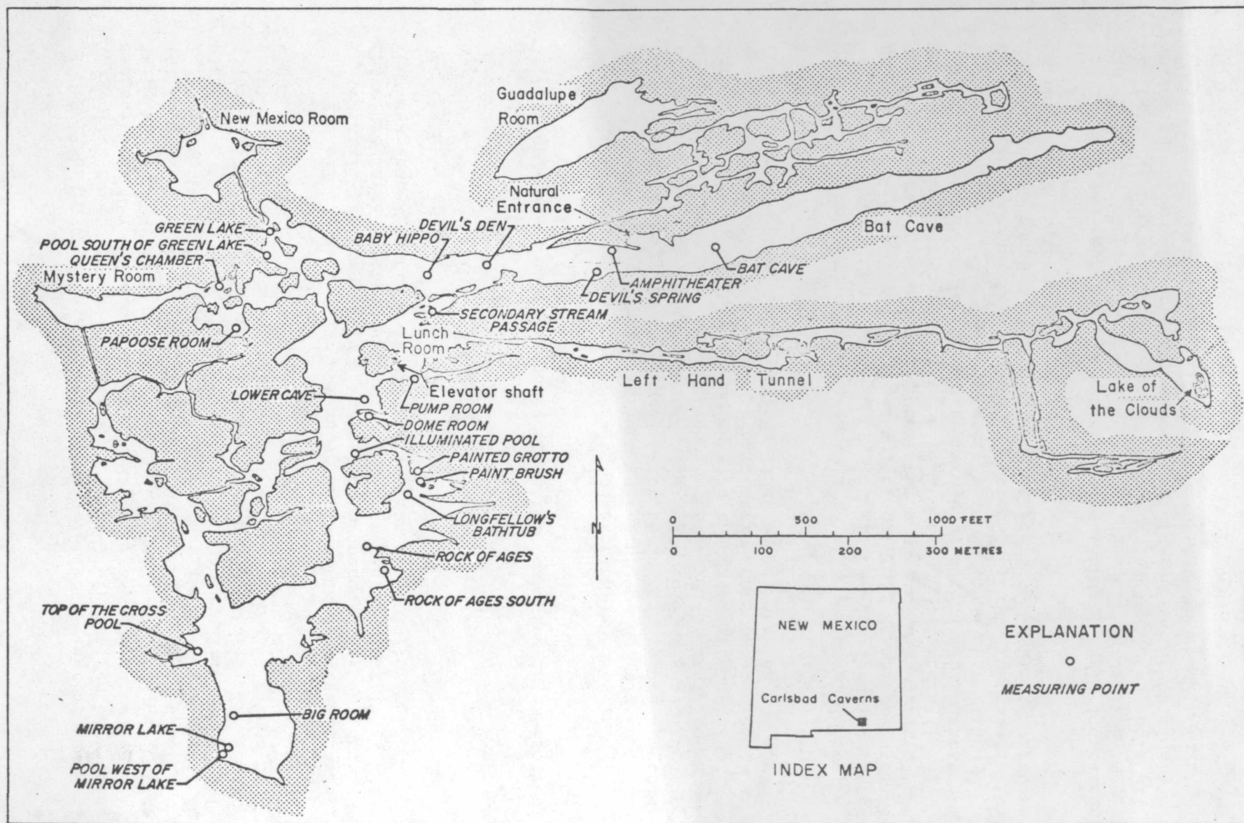
Figure 1.--Map of Carlsbad Caverns showing location of measuring points.
