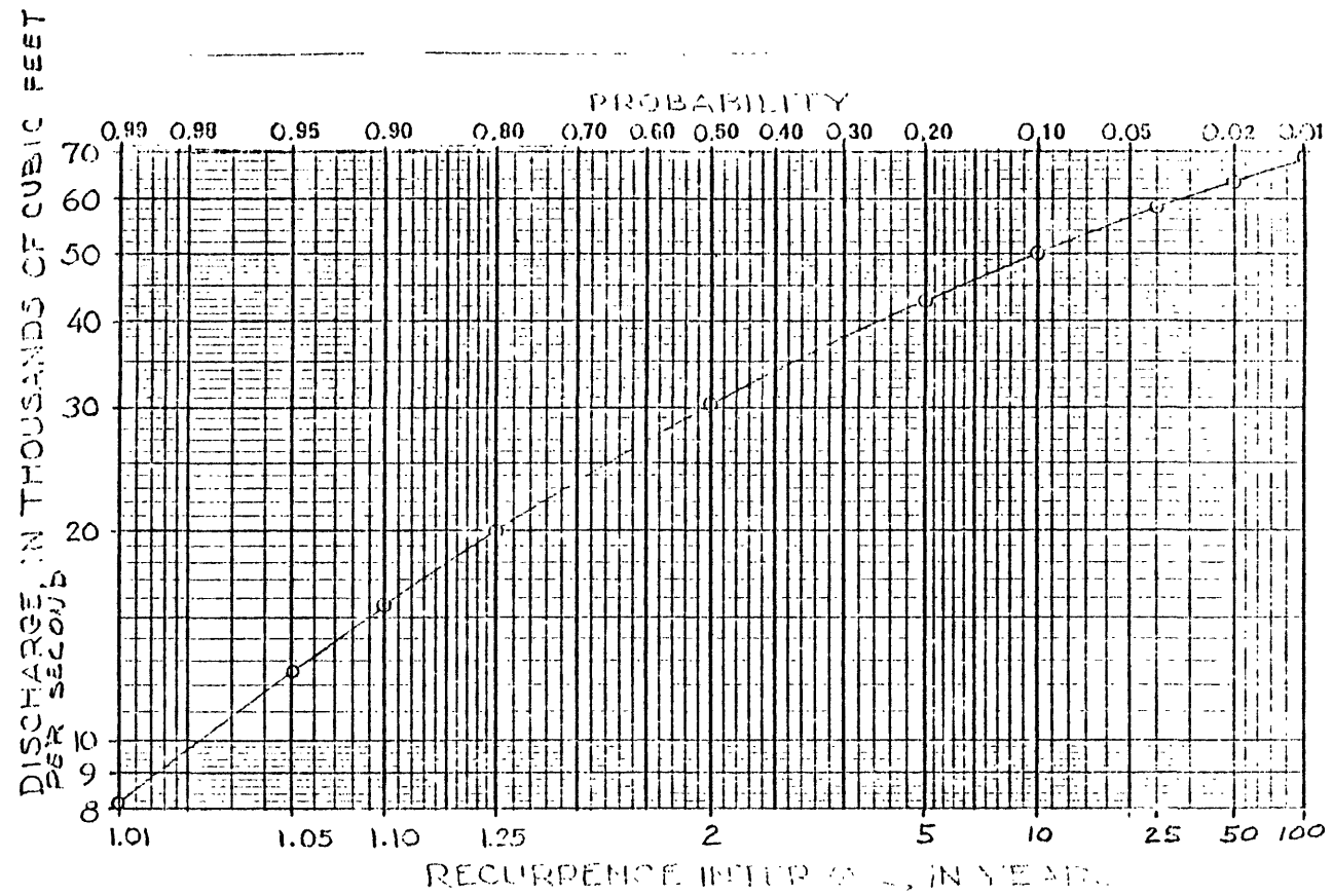
Figure 5.--Flood-frequency curve, Green River at Green River, Utah.
