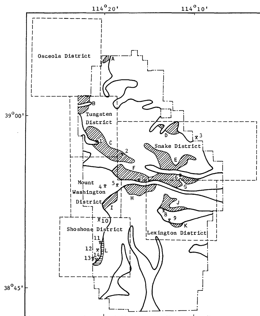
Figure 2.--Areas of mineral resource potential in the Wheeler Peak and Highland Ridge Further Planning Areas, Nevada.
