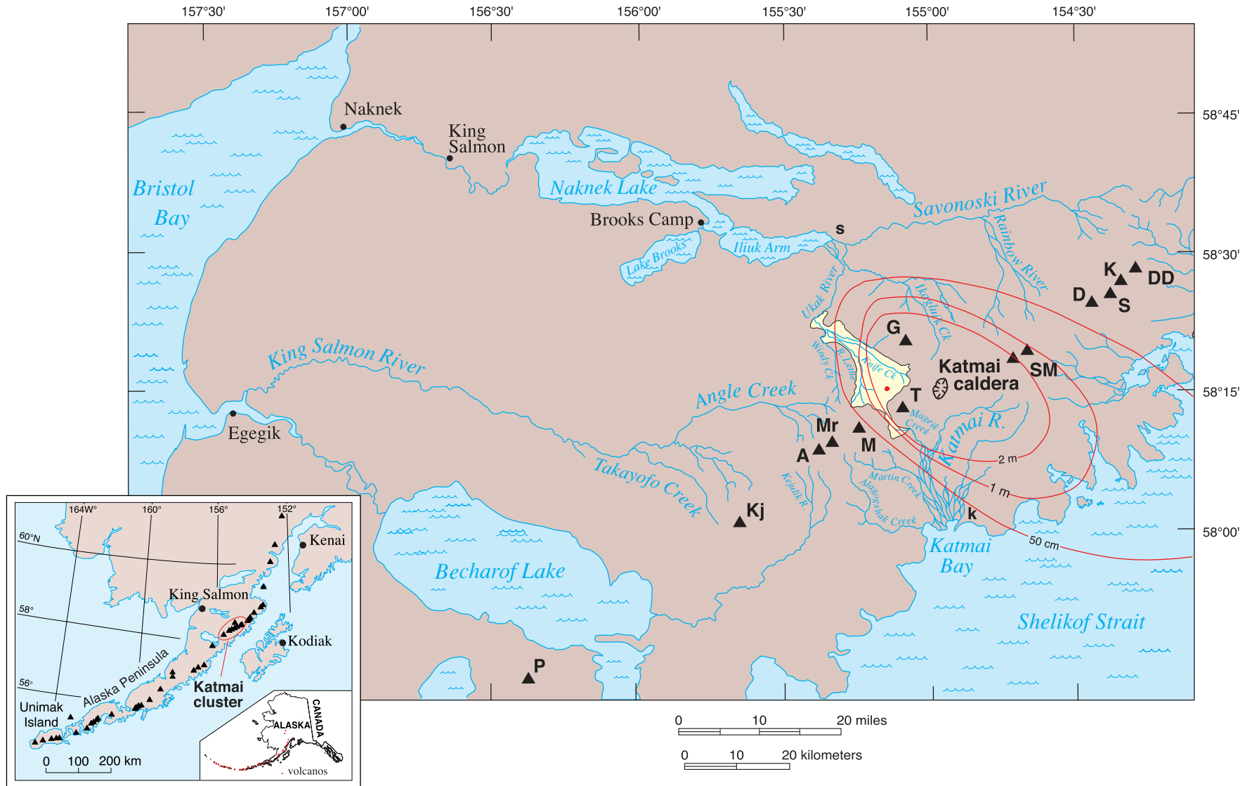
Figure 1. Regional setting of area mapped on upper Alaska Peninsula. Triangles indicate andesite-dacite stratovolcanoes, identified by letter from southwest to northeast: P =Peulik; Kj =Kejulik; A =Alagogshak; Mr =Martin; M =Mageik; T =Trident; G =Griggs; SM =Snowy Mountain (two cones); D =Denison; S =Steller; K =Kukak; DD =Devils Desk. Only Griggs volcano (formerly Knife Peak) lies significantly behind the main axial chain. Just west of Katmai caldera, yellow area is Valley of Ten Thousand Smokes ash-flow sheet, which erupted at Novarupta (red dot) in June 1912 and also poured south through Katmai Pass between Trident and Mageik volcanoes. Isopachs show thickness of cumulative 3-day plinian fallout from Novarupta. City of King Salmon and three villages indicated are the only settlements in this otherwise uninhabited wilderness. Small letters, k on Katmai Bay and s on Savonoski River, indicate sites of former villages abandoned during the 1912 eruption.
