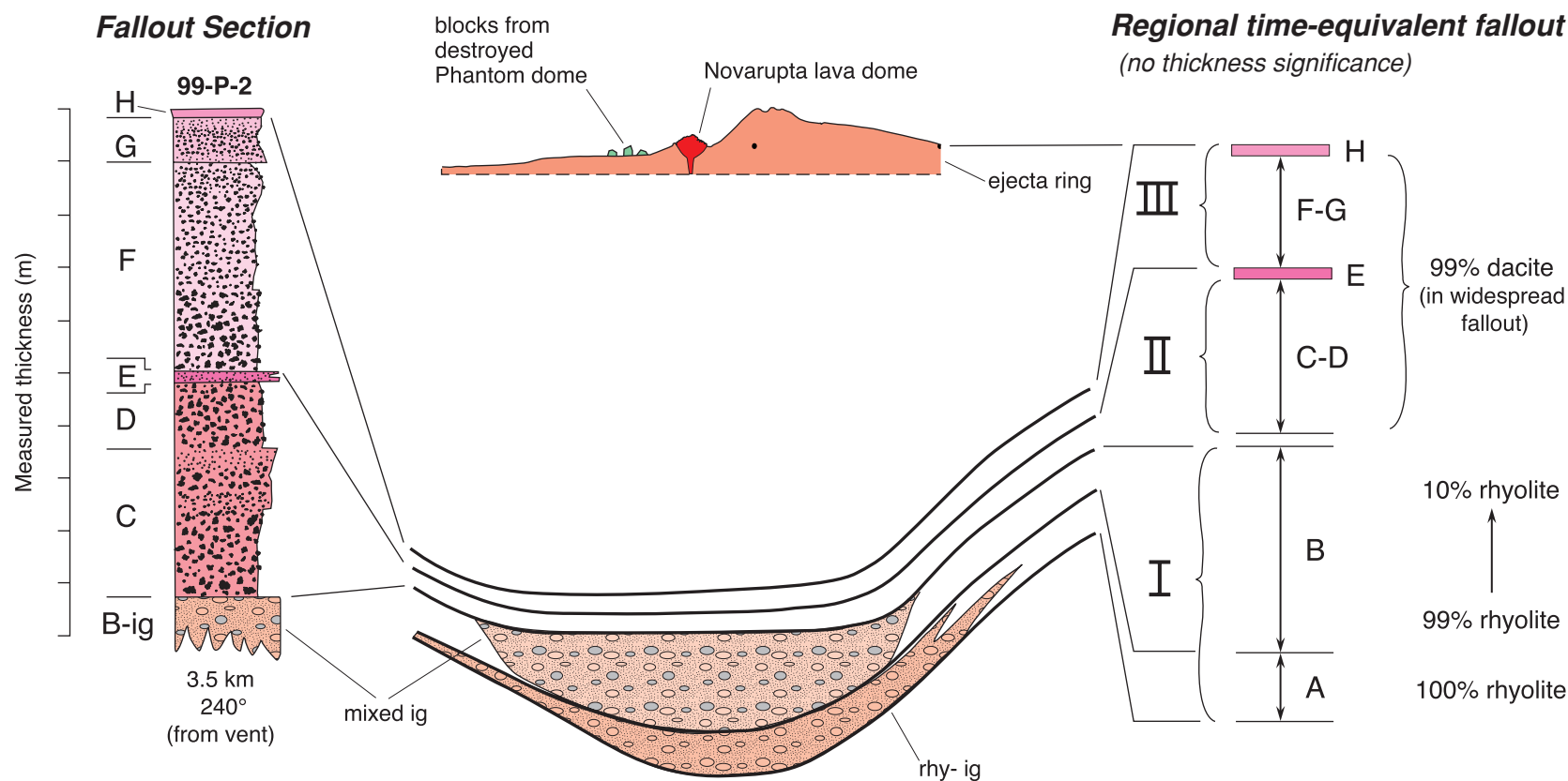
Figure 2. Eruptive sequence at Novarupta in 1912, showing schematically the concurrent emplacement during Episode I of compositionally zoned valley-filling ignimbrite (rhy ig, mixed ig) and fallout Layers A and B. These are overlain by fallout Layers C through H, emplaced during Episodes II and III on the second and third days of the eruption. Ejecta-ring material exposed close to the vent is coarser and more heterogeneous but is time-equivalent to region-wide fallout Layers G and upper F (Houghton and others, 2003). The capping dustfall, Layer H, is overlain proximally by dacitic lava blocks of transient Phantom dome, which was explosively destroyed before extrusion of rhyolitic Novarupta dome, which survived, terminating the sequence. Measured reference section 99-P-2 (Houghton and others, 2003) is at the north base of Mount Cerberus, 3.5 km southwest of the vent.
