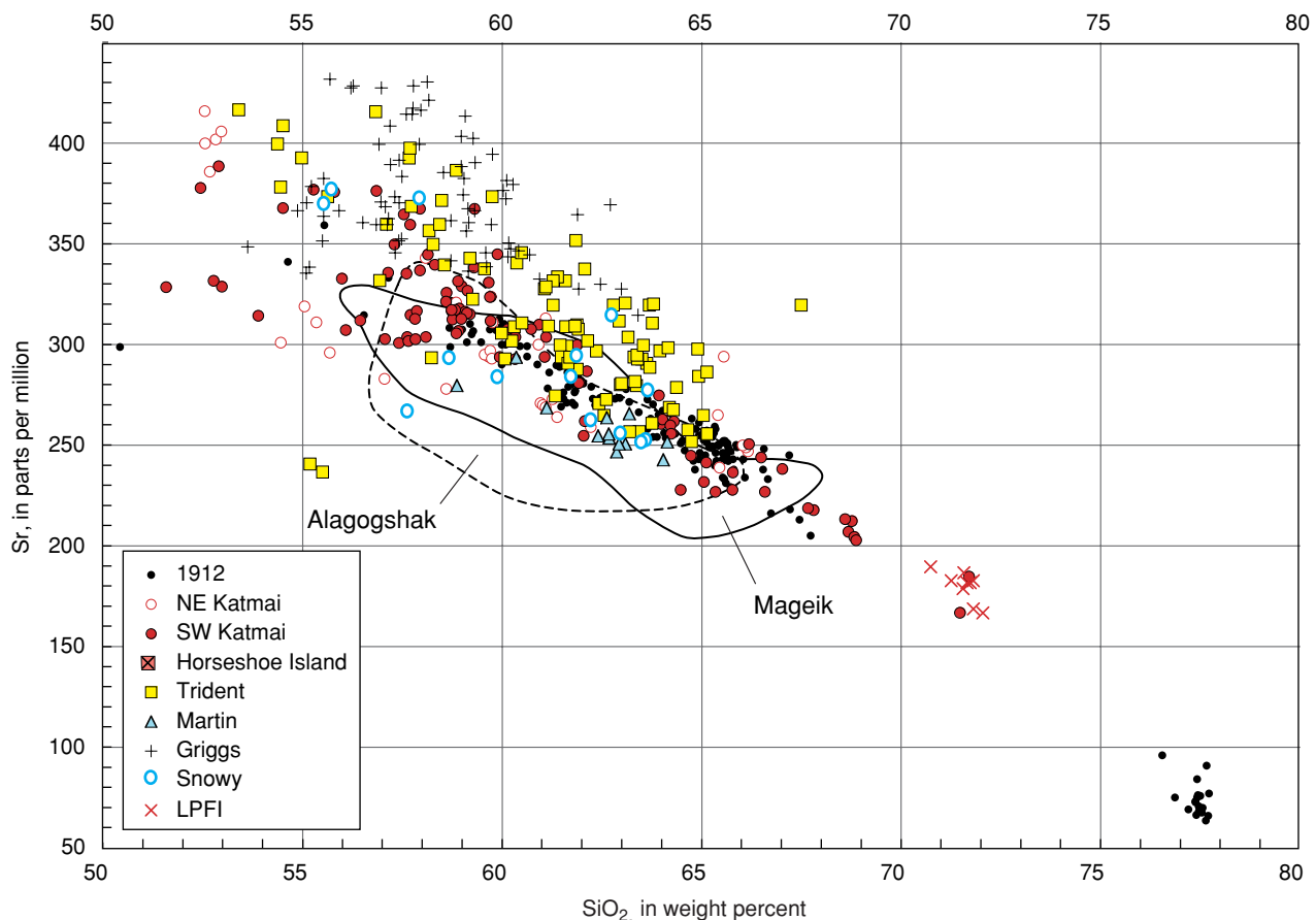
Figure 3. K 2 O, Zr, and Sr versus SiO 2 contents for products of Katmai cluster volcanoes. Symbols identified in inset. LPFI=late Pleistocene rhyodacite plinian pumice fall and ignimbrite (map unit krp) erupted at Mount Katmai. Horseshoe Island dacite dome (map unit khi) was emplaced on floor of Katmai caldera after 1912 collapse; it was sampled and analysed by Fenner (1950) for major elements but not for trace elements. For clarity, field outlines alone are plotted for Alagogshak (n=44) and Mageik (n=56) volcanoes; see Hildreth and others (1999, 2000) for plots of those data. Major elements are normalized to volatile-free totals of 99.6 wt % (leaving 0.4 wt % for trace elements and halogens). High-Zr cluster for Southwest Katmai at 64% SiO 2 represents unit kds.
