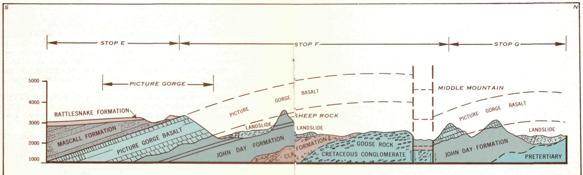
Fig. 5.—North-south section along the John Day River through Picture Gorge and Middle Mountain.
