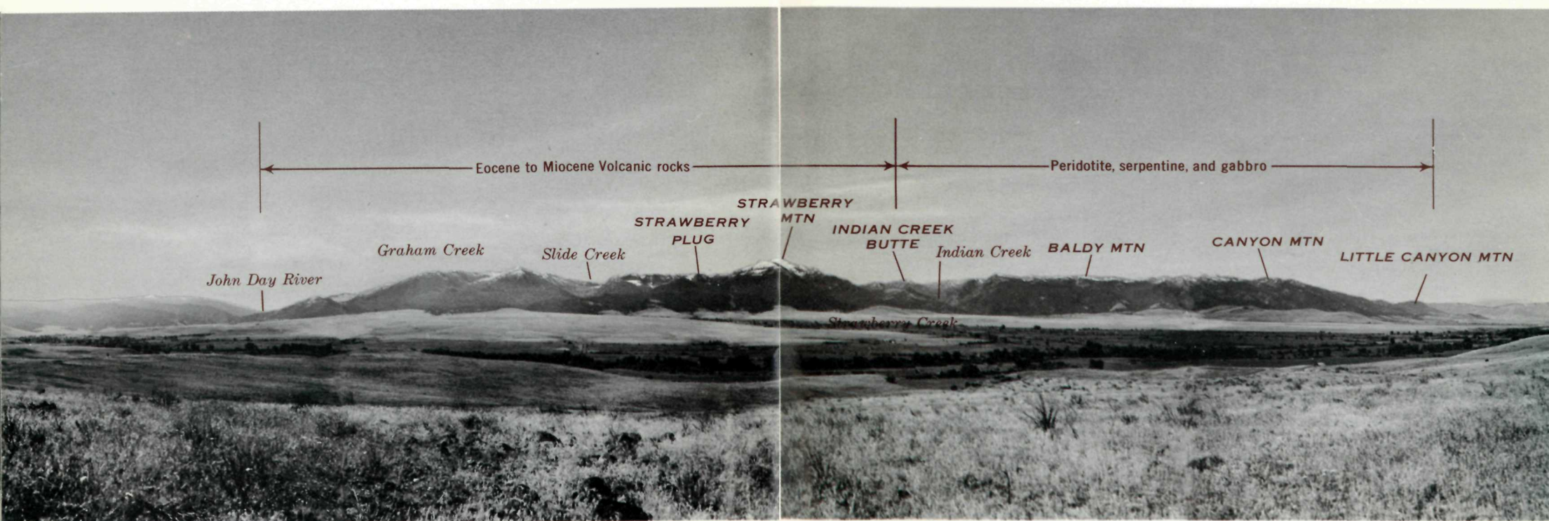
Fig. 13.—Panorama of the Strawberry Range and the John Day River valley from the north.
