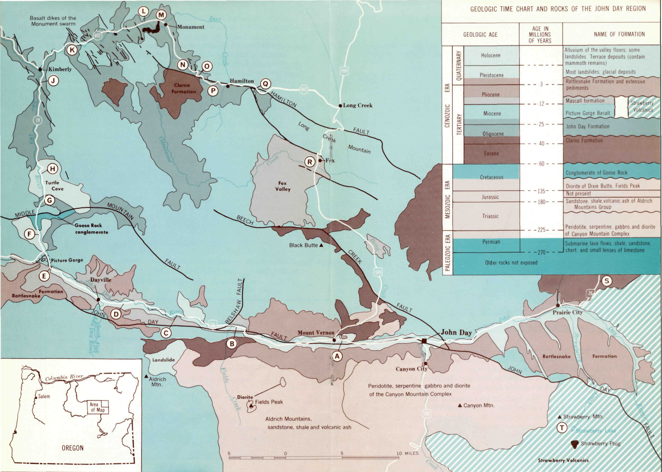
Fig. 1.—Geologic map of the John Day Country showing road log route.
