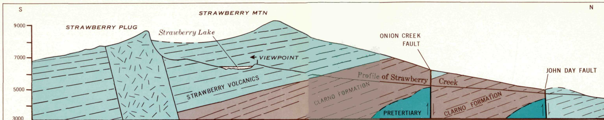
Fig. 14.—Section through the Strawberry Mountain, along Strawberry Creek.
