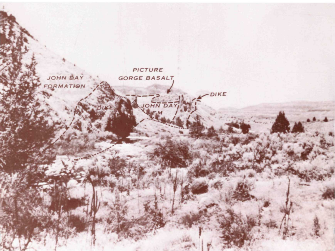
Fig. 8.—Basalt dike two miles south of Kimberly.
