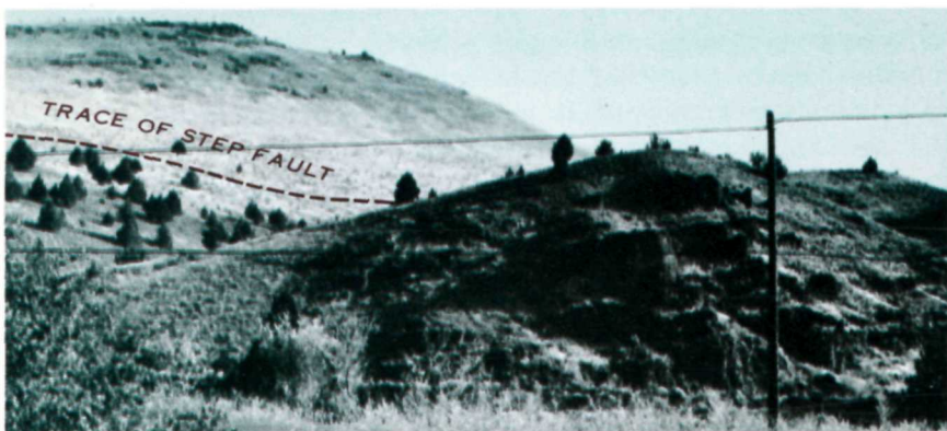
Fig. 2.—View of Mount Vernon Butte and diagram of faulting along its south slope.
