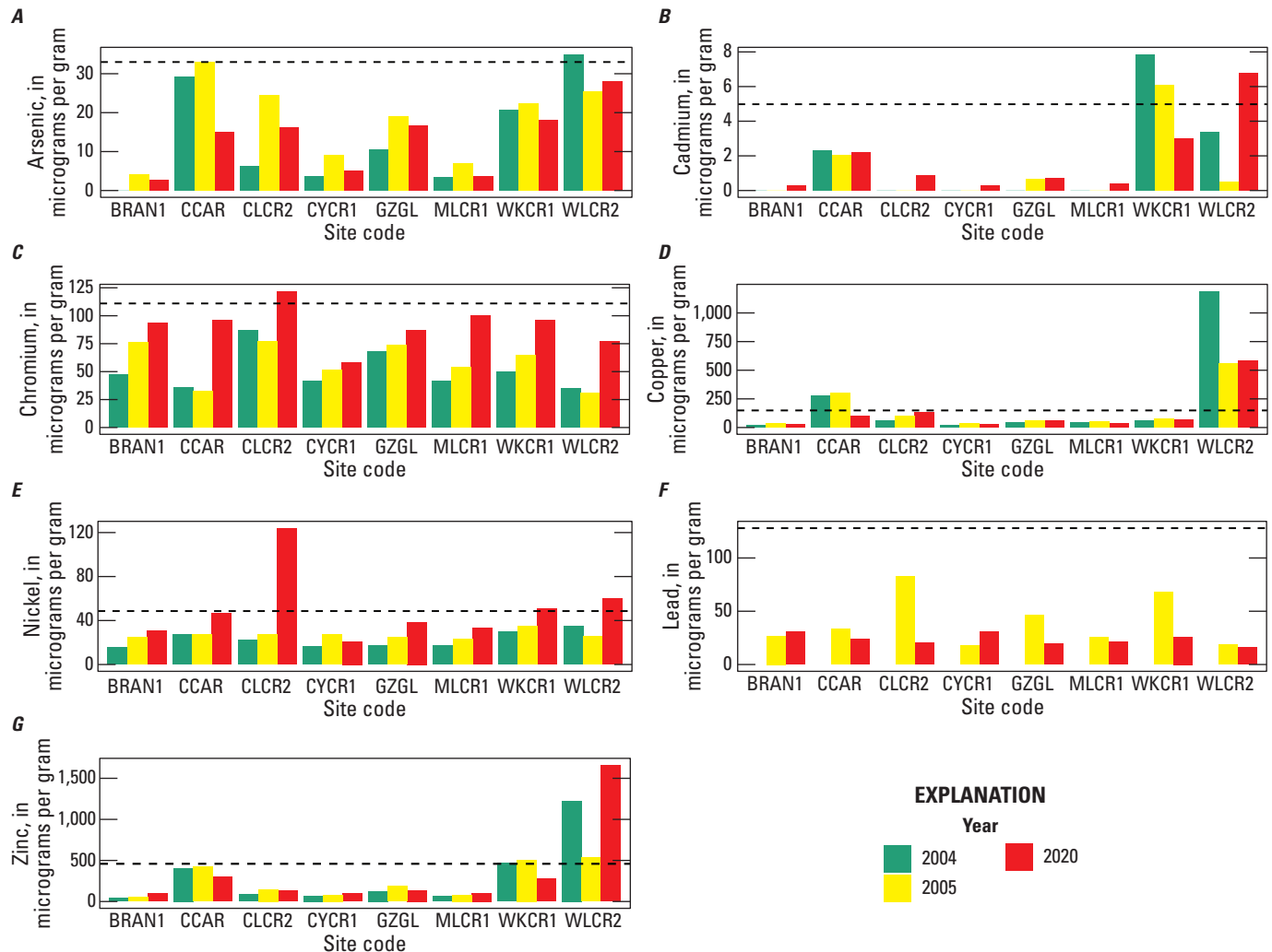
Figure 4. Average concentrations of metals of biological concern measured in bed sediment samples from sample locations in Whiskeytown National Recreation Area, Shasta County, California, 2004–20 (Wulff and others, 2023). The dashed line represents the consensus-based probable effect concentration (PEC) from sediment-quality guidelines in MacDonald and others (2000). Site code abbreviations: BRAN1, Brandy Creek near Whiskeytown; CCAR, Clear Creek above Carr Powerhouse near French Gulch; CLCR2, Clear Creek at Peltier Valley Road near Shasta; CYCR1, Crystal Creek near mouth near French Gulch; GZGL, Grizzly Gulch near Whiskeytown; MLCR1, Mill Creek near French Gulch; WKCR1, Whiskey Creek near Whiskeytown; WLCR2, Willow Creek near French Gulch.
