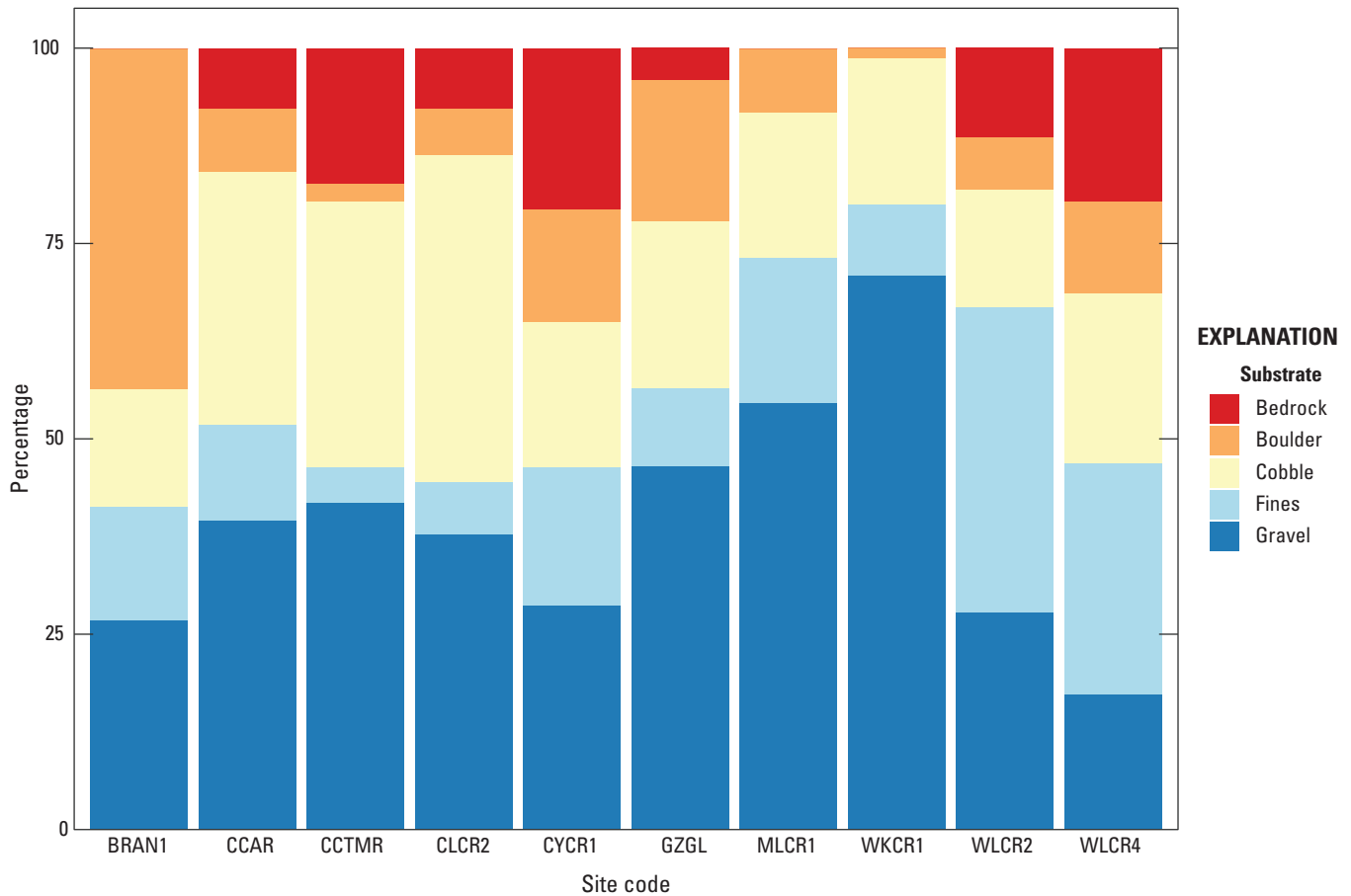
Figure 8. Percentage substrate size characterization summarized by site within Whiskeytown National Recreation Area, California, 2020 (Wulff and others, 2023). Substrate categories are as follows: smooth bedrock/concrete/hardpan; silt; sand (greater than [ > ] 0.063–2 millimeters [mm]); fine gravel, fine/medium gravel ( >2 –16 mm); coarse gravel ( >16 –32 mm); very coarse gravel ( >32 –64 mm); small cobble ( >64 –128 mm); large cobble ( >128 –256 mm); small boulder ( >256 –512 mm); large boulder ( >512 mm); percentage bedrock; percentage fines, percentage silt + percentage sand; percentage gravel, percentage fine/medium gravel + percentage coarse gravel + percentage very coarse gravel; percentage cobble, percentage small cobble + percentage large cobble; percentage boulder, percentage small boulder + percentage large boulder (Fitzpatrick and others, 1998). Site code abbreviations: BRAN1, Brandy Creek near Whiskeytown; CCAR, Clear Creek above Carr Powerhouse near French Gulch; CCTMR, Clear Creek near French Gulch; CLCR2, Clear Creek at Peltier Valley Road near Shasta; CYCR1, Crystal Creek near mouth near French Gulch; GZGL, Grizzly Gulch near Whiskeytown; MLCR1, Mill Creek near French Gulch; WKCR1, Whiskey Creek near Whiskeytown; WLCR2, Willow Creek near French Gulch; WLCR4, Willow Creek at Trinity Mountain Road near French Gulch.
