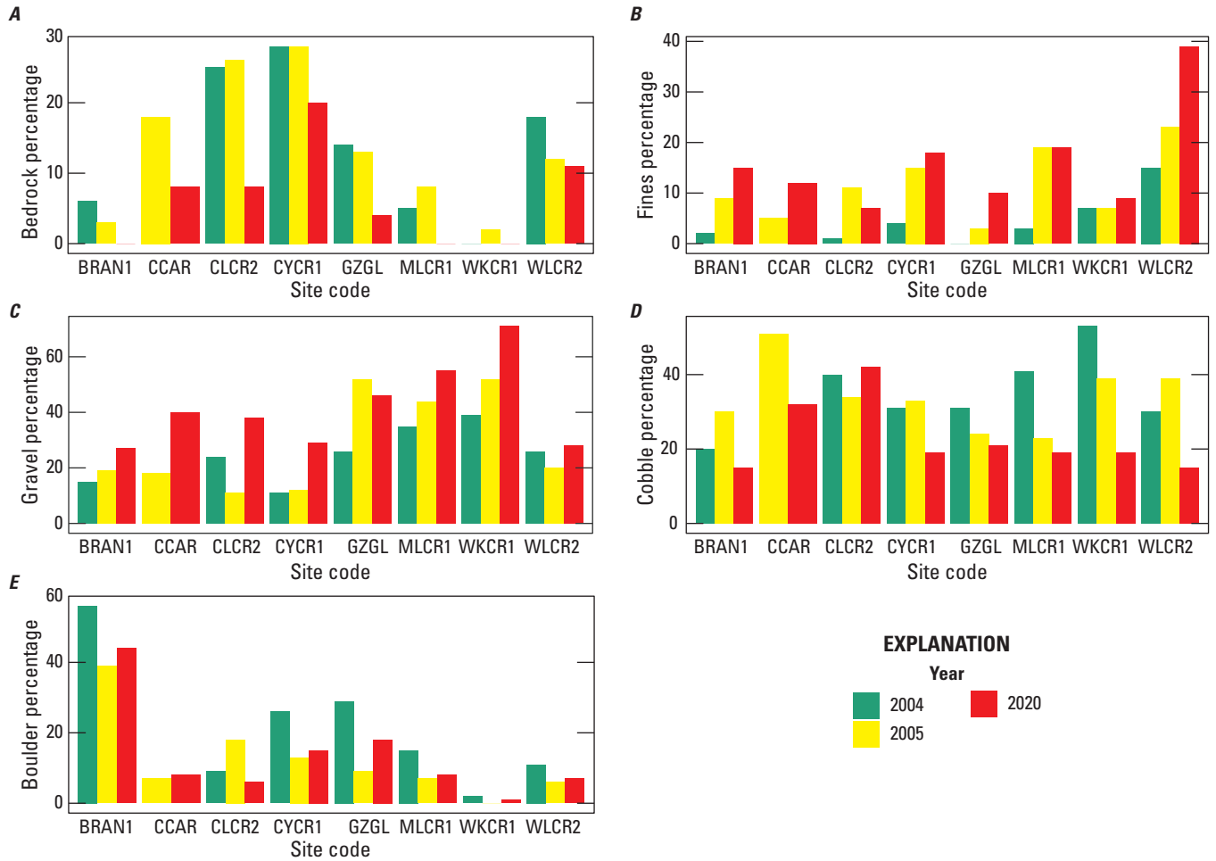
Figure 10. Substrate size characterization summarized by site within Whiskeytown National Recreation Area, California, 2004–20 (Wulff and others, 2023). There were 220 total particles (n) measured at each site. Site code abbreviations: BRAN1, Brandy Creek near Whiskeytown; CCAR, Clear Creek above Carr Powerhouse near French Gulch; CLCR2, Clear Creek at Peltier Valley Road near Shasta; CYCR1, Crystal Creek near mouth near French Gulch; GZGL, Grizzly Gulch near Whiskeytown; MLCR1, Mill Creek near French Gulch; WKCR1, Whiskey Creek near Whiskeytown; WLCR2, Willow Creek near French Gulch.
