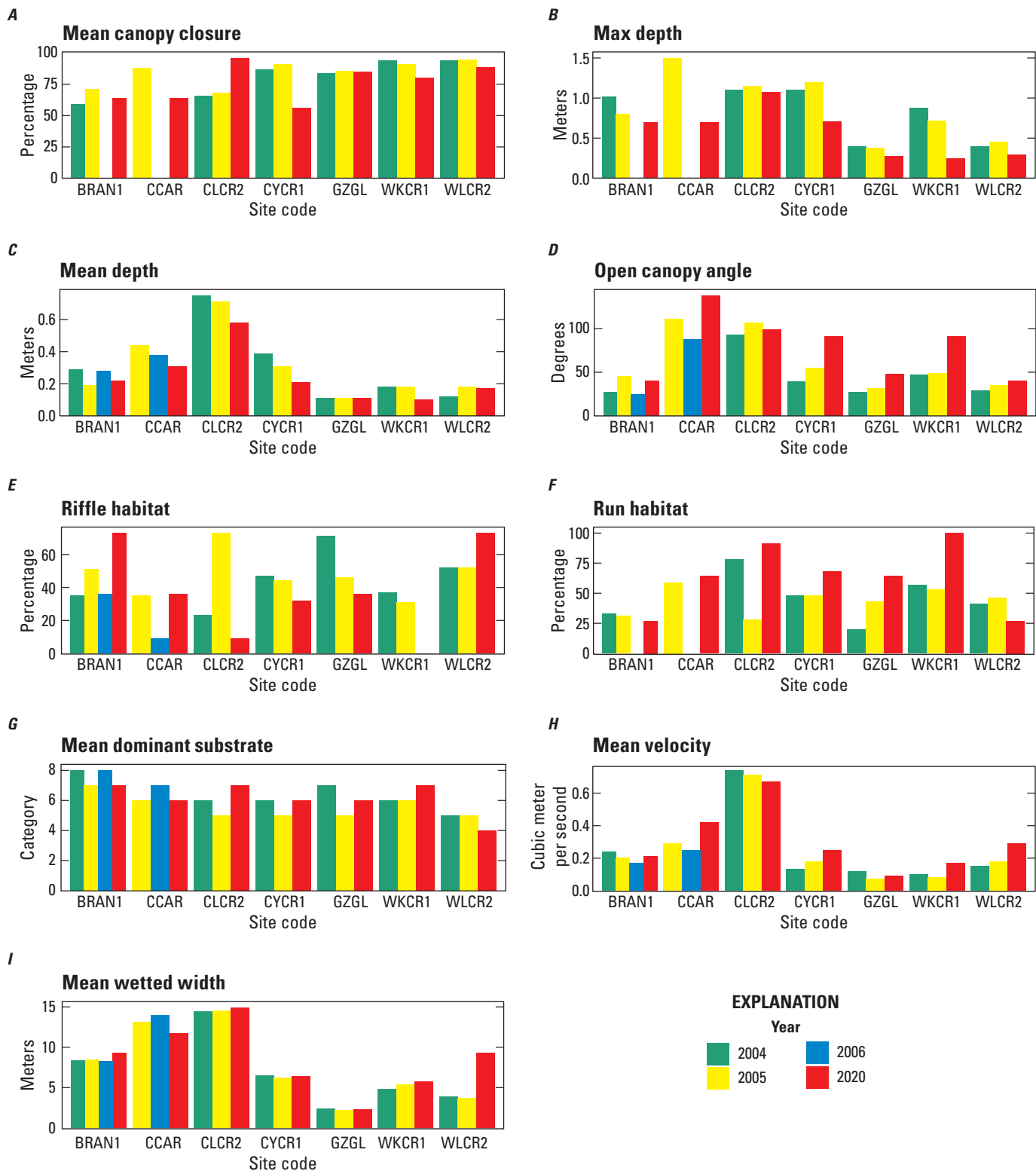
Figure 9. Selected stream-habitat characteristics of sites in Whiskeytown Recreation Area, Shasta County, California, 2004–20 (Wulff and others, 2023). Site code abbreviations: BRAN1, Brandy Creek near Whiskeytown; CCAR, Clear Creek above Carr Powerhouse near French Gulch; CLCR2, Clear Creek at Peltier Valley Road near Shasta; CYCR1, Crystal Creek near mouth near French Gulch; GZGL, Grizzly Gulch near Whiskeytown; WKCR1, Whiskey Creek near Whiskeytown; WLCR2, Willow Creek near French Gulch.
