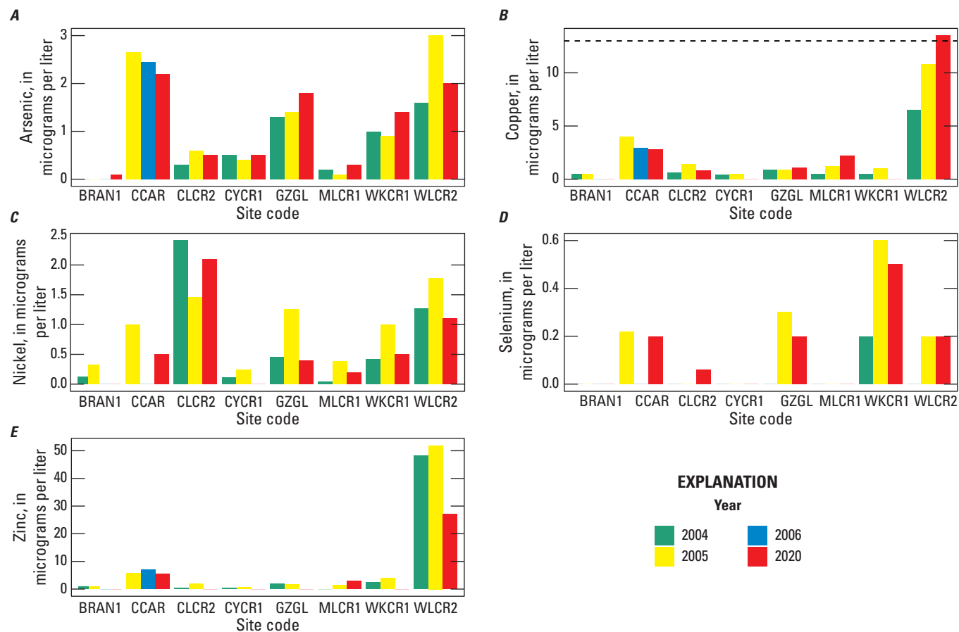
Figure 3. Concentrations of metals of biological concern measured in filtered water from sample locations within Whiskeytown National Recreation Area, Shasta County, California, 2004–20 (Wulff and others, 2023). The dashed line represents chronic toxicity for sculpin ( Cottus ) calculated for a water hardness of 100 milligrams per liter (mg/L; Besser and others, 2007), which is similar to the water hardness of 102 mg/L measured in Willow Creek near French Gulch (WLCR2; Wulff and others, 2023). Site code abbreviations: BRAN1, Brandy Creek near Whiskeytown; CCAR, Clear Creek above Carr Powerhouse near French Gulch; CLCR2, Clear Creek at Peltier Valley Road near Shasta; CYCR1, Crystal Creek near mouth near French Gulch; GZGL, Grizzly Gulch near Whiskeytown; MLCR1, Mill Creek near French Gulch; WKCR1, Whiskey Creek near Whiskeytown; WLCR2, Willow Creek near French Gulch.
