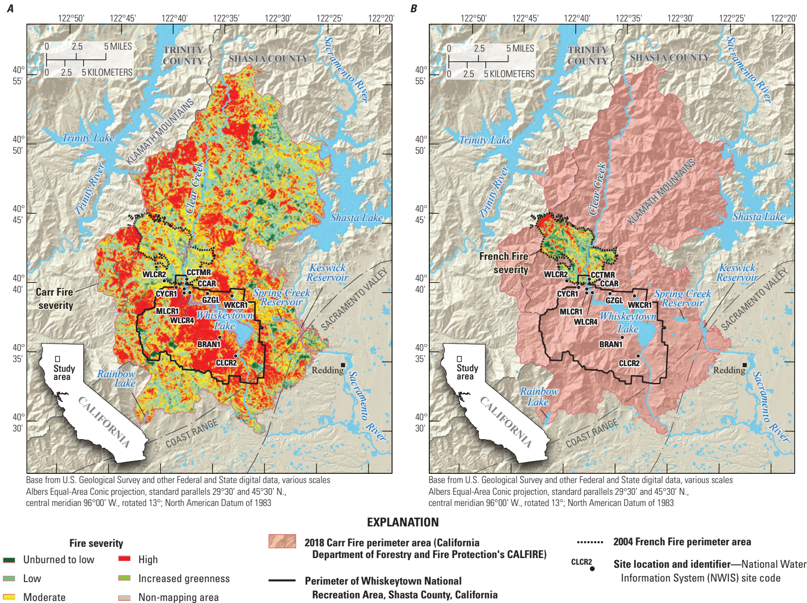
Figure 1. A , Burn severity of the Carr Fire and B , burn severity of the 2004 French Fire, in relation to the 2020 sample site locations within Whiskeytown National Recreation Area, Shasta County, California (U.S. Geological Survey, 2016; U.S. Geological Survey Burn Severity Portal, 2022). Site code abbreviations: BRAN1, Brandy Creek near Whiskeytown; CCAR, Clear Creek above Carr Powerhouse near French Gulch; CLCR2, Clear Creek at Peltier Valley Road near Shasta; CCTMR, Clear Creek near French Gulch; CYCR1, Crystal Creek near mouth near French Gulch; GZGL, Grizzly Gulch near Whiskeytown; MLCR1, Mill Creek near French Gulch; WLCR1, Whiskey Creek near Whiskeytown; WLCR2, Willow Creek near French Gulch; WLCR4, Willow Creek at Trinity Mountain Road near French Gulch.
