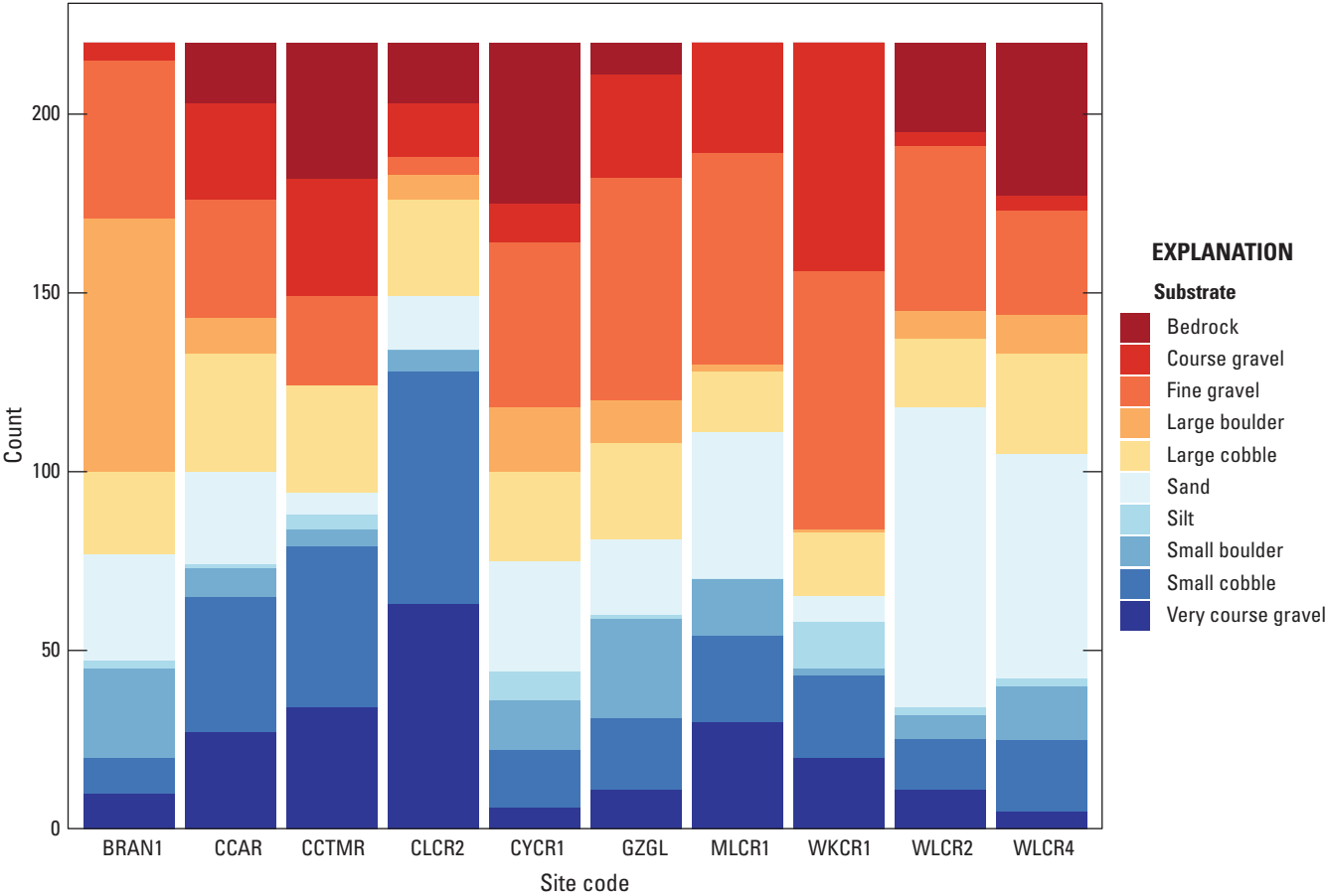
Figure 7. Substrate size characterization summarized by site within Whiskeytown National Recreation Area, California, 2020 (Wulff and others, 2023). There were 220 total particles (n) measured at each site. Substrate categories are as follows: smooth bedrock/concrete/hardpan; silt; sand (greater than [ > ] 0.063–2 millimeters [mm]); fine gravel, fine/medium gravel ( > 2–16 mm); coarse gravel ( > 16–32 mm); very coarse gravel ( > 32–64 mm); small cobble ( > 64–128 mm); large cobble ( > 128–256 mm); small boulder ( > 256–512 mm); large boulder ( > 512 mm; Fitzpatrick and others, 1998). Site code abbreviations: BRAN1, Brandy Creek near Whiskeytown; CCAR, Clear Creek above Carr Powerhouse near French Gulch; CCTMR, Clear Creek near French Gulch; CLCR2, Clear Creek at Peltier Valley Road near Shasta; CYCR1, Crystal Creek near mouth near French Gulch; GZGL, Grizzly Gulch near Whiskeytown; MLCR1, Mill Creek near French Gulch; WKCR1, Whiskey Creek near Whiskeytown; WLCR2, Willow Creek near French Gulch; WLCR4, Willow Creek at Trinity Mountain Road near French Gulch.
