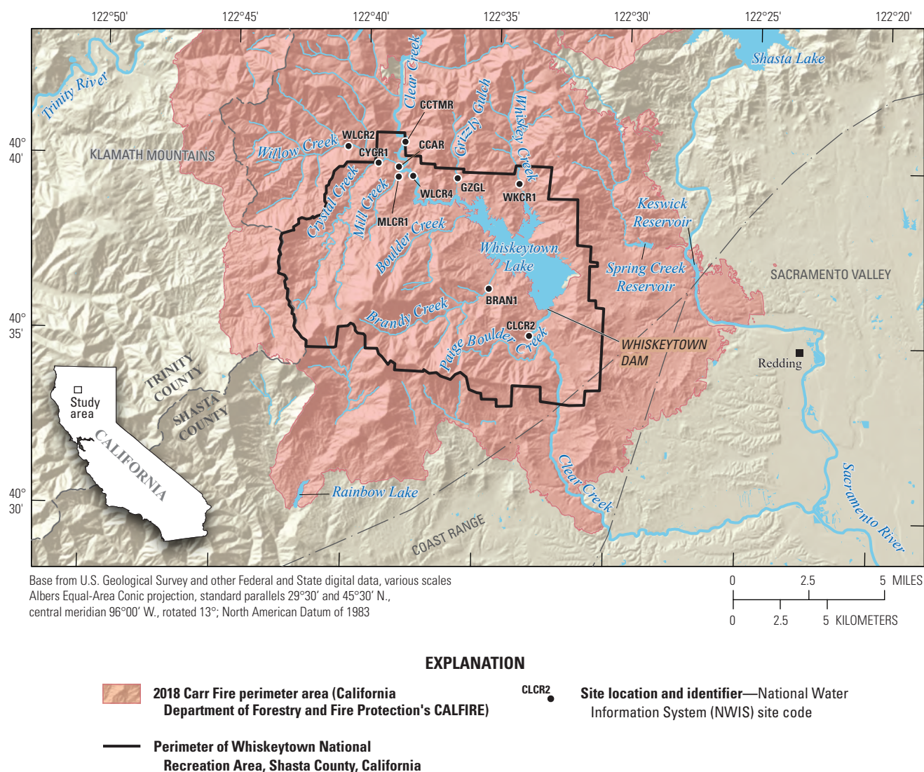
Figure 2. Location of survey sites within Whiskeytown National Recreation Area, Shasta County, California (U.S. Geological Survey, 2016). Site code abbreviations: BRAN1, Brandy Creek near Whiskeytown; CCAR, Clear Creek above Carr Powerhouse near French Gulch; CLCR2, Clear Creek at Peltier Valley Road near Shasta; CCTMR, Clear Creek near French Gulch; CYCR1, Crystal Creek near mouth near French Gulch; GZGL, Grizzly Gulch near Whiskeytown; MLCR1, Mill Creek near French Gulch; WLCR1, Whiskey Creek near Whiskeytown; WLCR2, Willow Creek near French Gulch; WLCR4, Willow Creek at Trinity Mountain Road near French Gulch.
