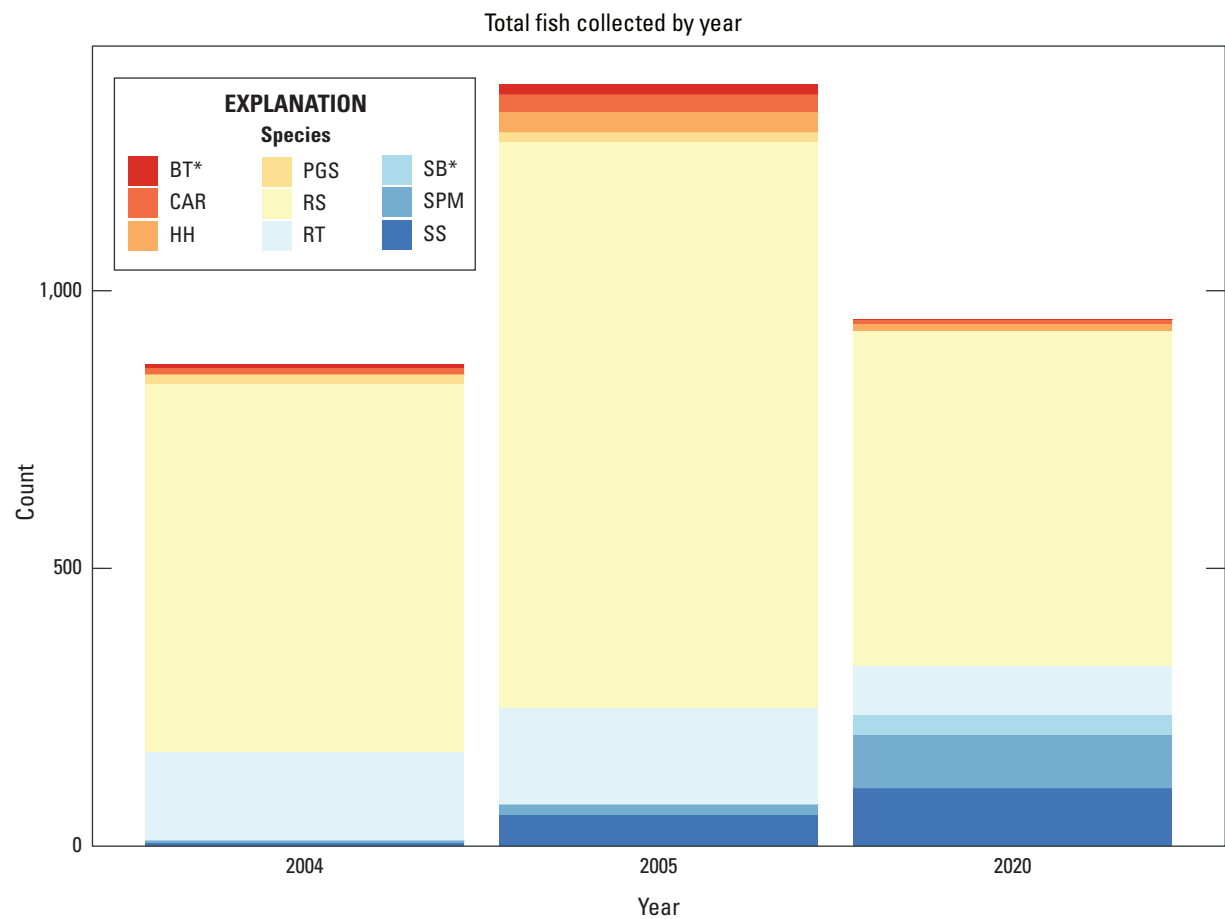
Figure 11. Count summary by year for fish and amphibians collected by backpack electroshock sampling in Whiskeytown Recreation Area, Shasta County, California, 2004–20 (Wulff and others, 2023). Abbreviations: BT, brook trout* ( Salvelinus fontinalis ); CAR, California Roach ( Hesperoleucus symmetricus ); HH, Hardhead ( Mylopharodon conocephalus ); PGS, Pacific Giant Salamander ( Dicamptodon tenebrosus ); RS, riffle sculpin ( Cottus gulosus ); RT, Rainbow Trout ( Oncorhynchus mykiss ); SB, Spotted Bass* ( Micropterus punctulatus ); SPM, Sacramento Pikeminnow ( Ptychocheilus grandis ); SS, Sacramento Sucker ( Catostomus occidentalis ); *, non-native.
