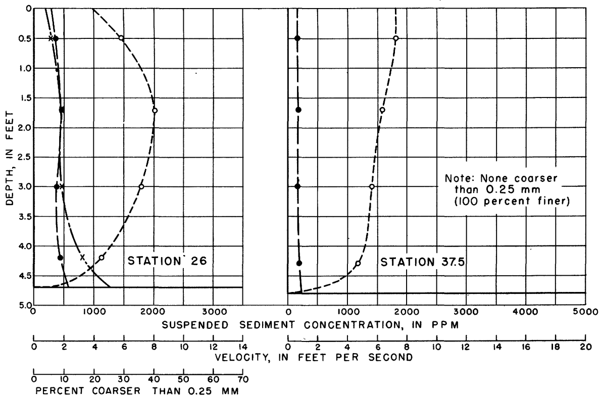
Figure 31.--Vertical distributions at section B, June 28, 1951.
