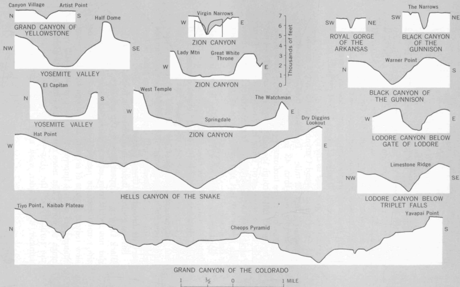
FIGURE 1.—Comparative profiles of several well-known American canyons.
