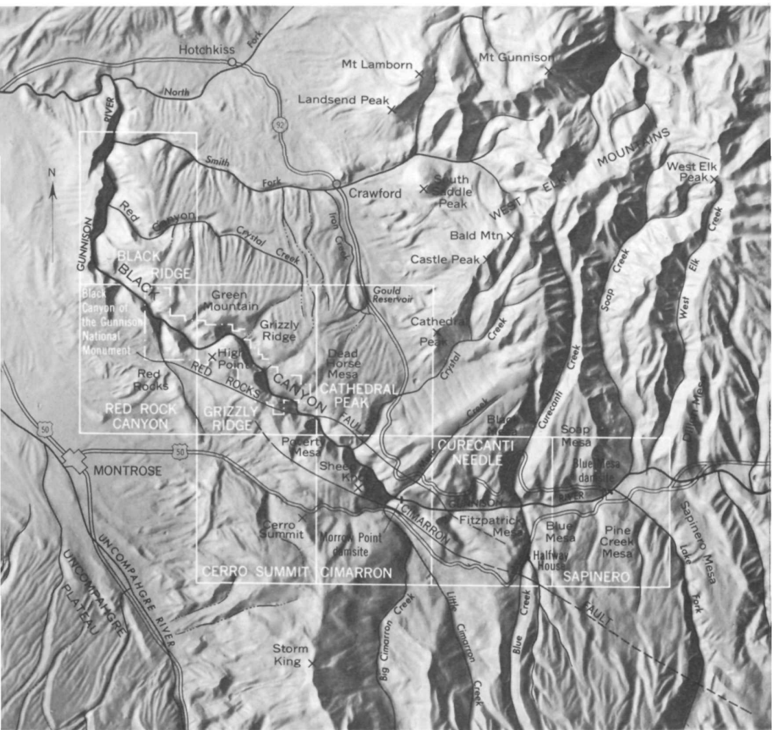
FIGURE 2.—The Black Canyon area.
