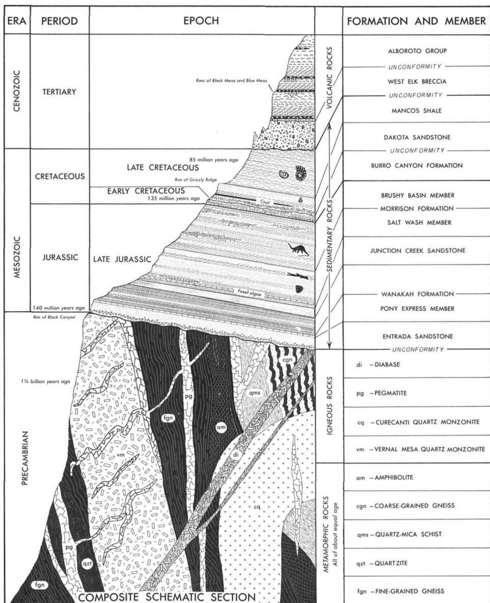
FIGURE 8.—Rock formations of the Black Canyon area.
