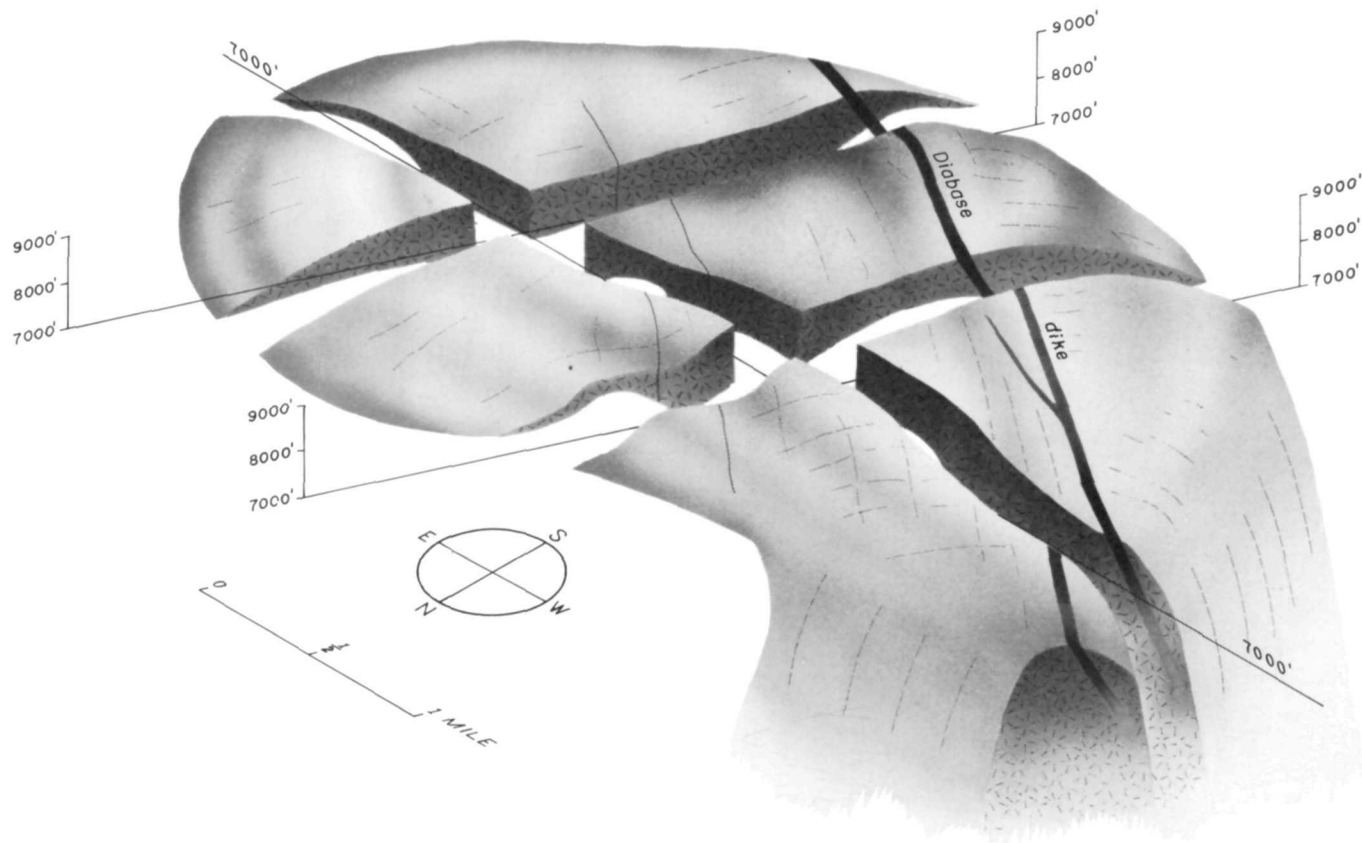
FIGURE 12.—Stereogram of the Curecanti pluton showing generalized restored form of the uneroded body.
