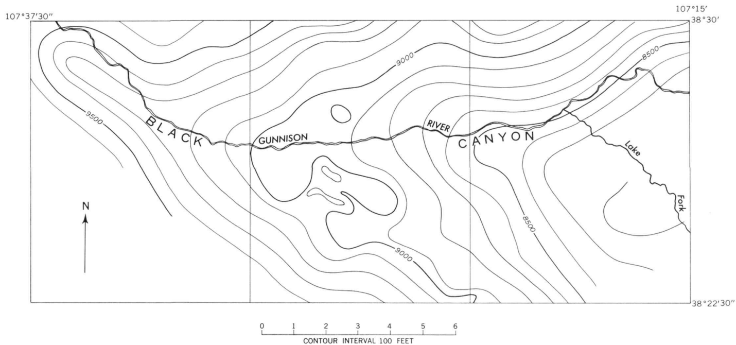
FIGURE 23.—Structure contour map, drawn at the base of the ash-flow tuff volcanic sequence, showing trend of the Gunnison River along syncline axis.
