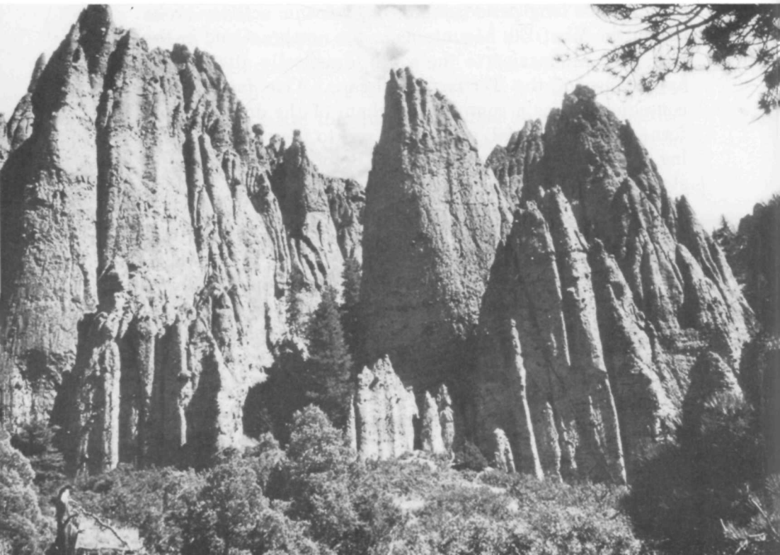
FIGURE 18.—Craggy outcrops of West Elk Breccia near head of Black Canyon at mouth of West Elk Creek. Note embedded fragments and crude bedding. Craggs are about 600 feet high.
