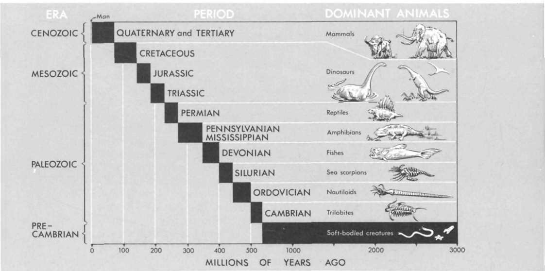
FIGURE 6.—Major divisions of geologic time.
