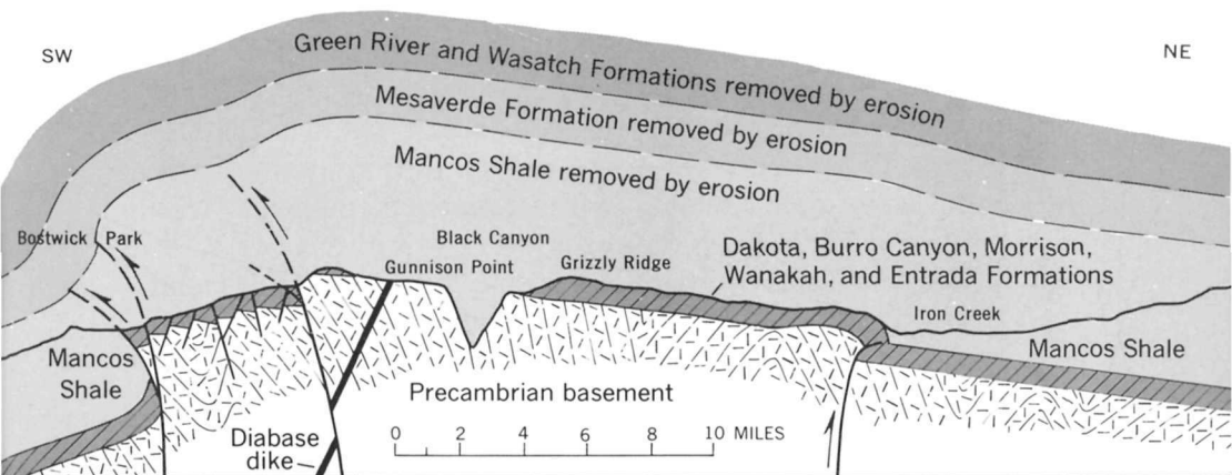
FIGURE 19.—Generalized section across Gunnison uplift showing restored form. Vertical scale is exaggerated about 2\frac{1}{2} times.
