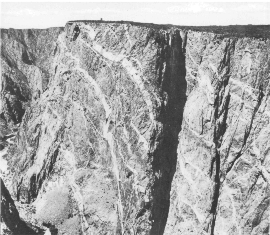
Painted Wall, Black Canyon of the Gunnison National Monument.
