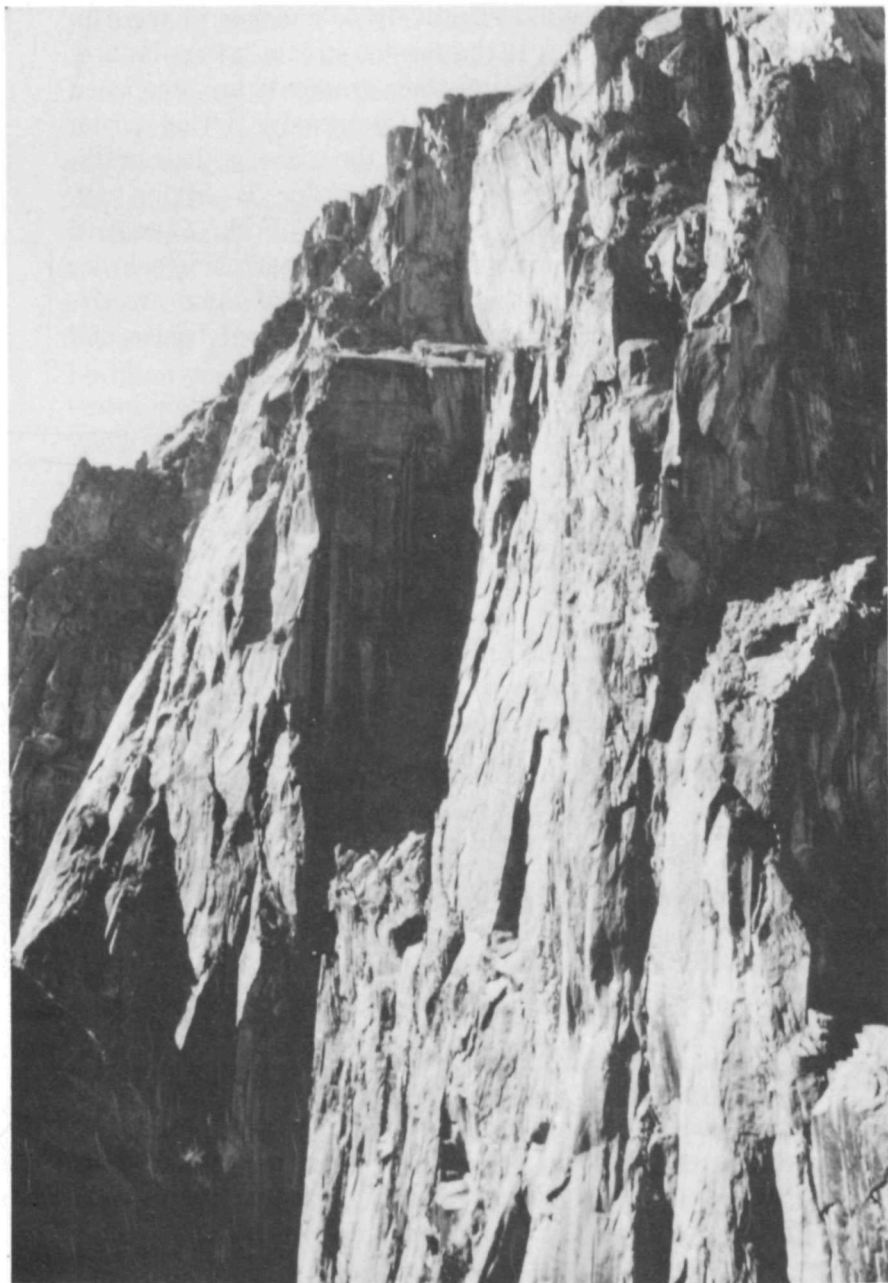
FIGURE 5.—Chasm Wall, at north end of Vernal Mesa, has a nearly vertical drop of 1,800 feet. Only the upper half of the cliff is shown in this view. Rock is Vernal Mesa Quartz Monzonite. Exfoliation along vertical joints contributes to sheerness.
