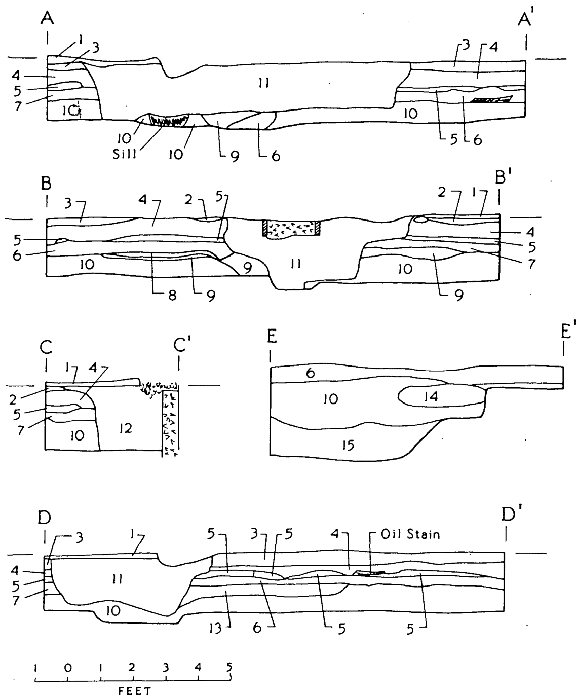
Soil Sections From Excavation of NW Bastion
