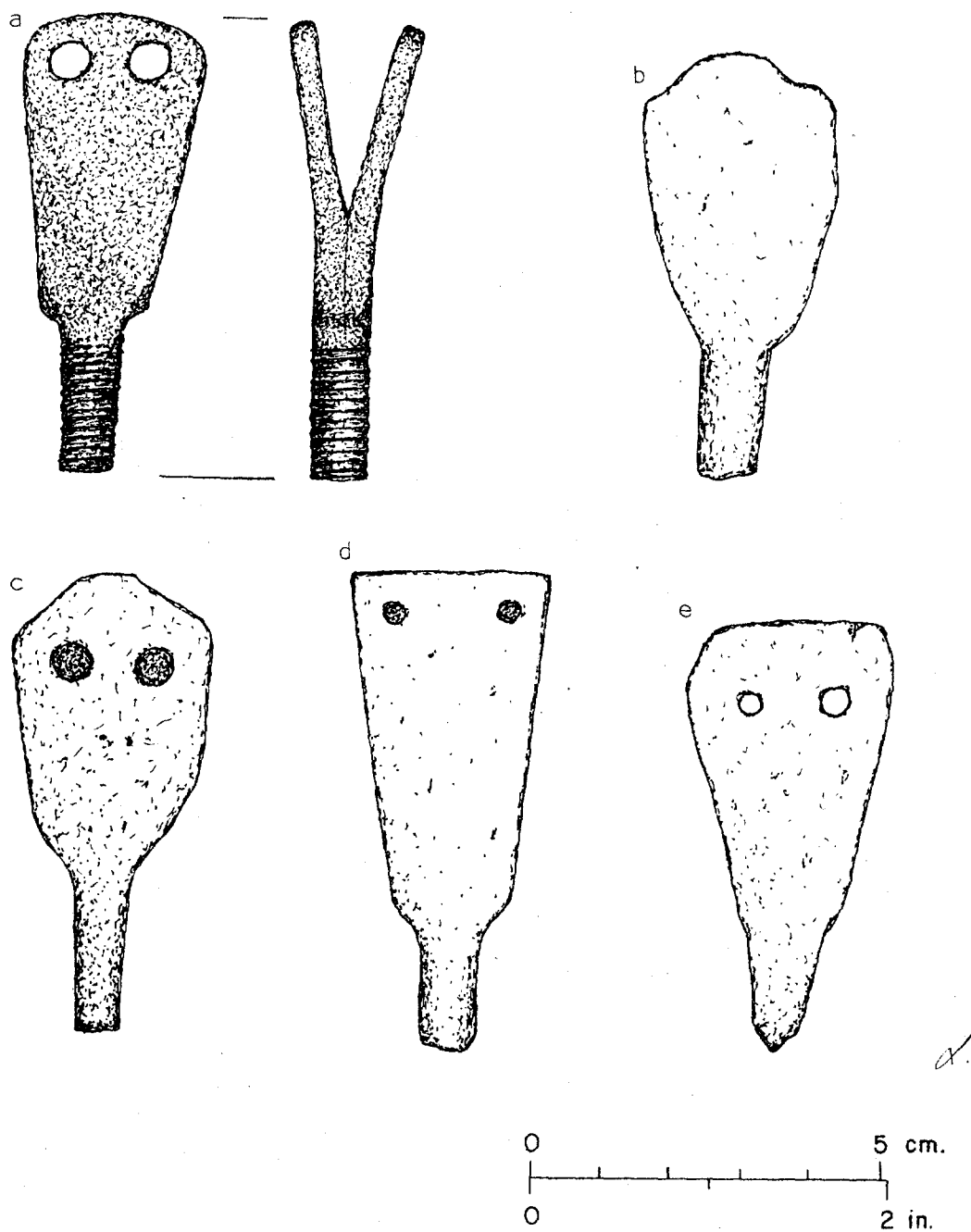
Fig. 67 -- Trap jaw posts and preforms from the Blacksmith Shop area: a). trap jaw post (FOVA 36077); b). jaw post preform (FOVA 36078); c). jaw post preform (FOVA 35024); d). jaw post preform (FOVA 36078) and e). jaw post preform (FOVA 36029).
