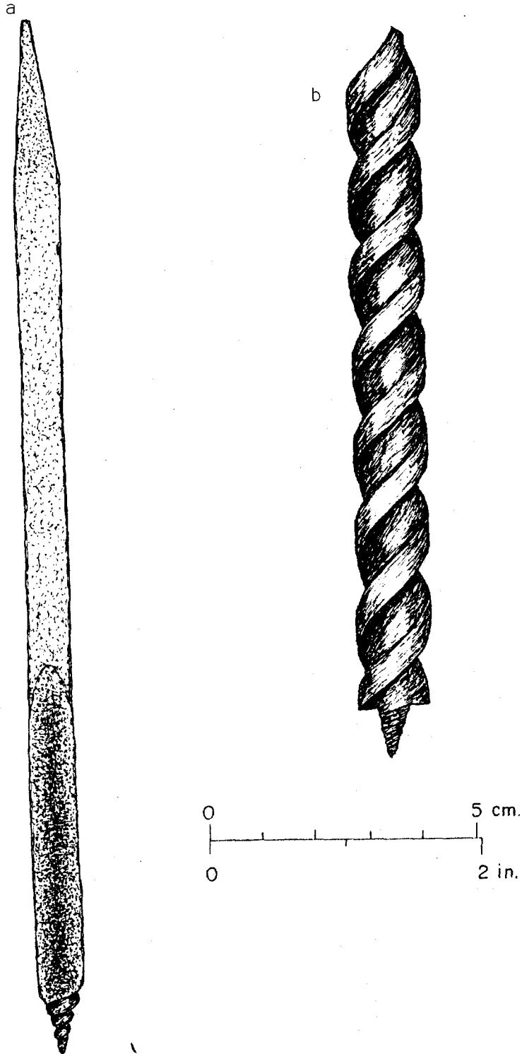
Fig. 51 -- Wood drill bits from the Blacksmith Shop area: a). drill bit (FOVA 34446) and b). auger bit (FOVA 34375).
