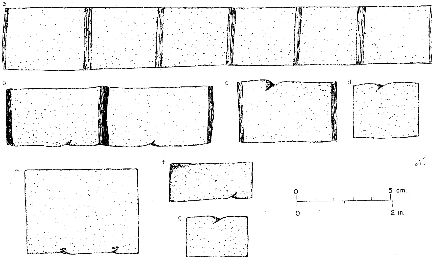
Fig. 85 -- Miscellaneous barbed wedges and preforms from the Blacksmith Shop area: a). barbed wedge preform template (FOVA 35759); b). barbed wedge preform (FOVA 33529); c). barbed wedge (FOVA 32813); d). barbed wedge (FOVA 32813); e). barbed wedge (FOVA 34917); f). barbed wedge (FOVA 34297); g). barbed wedge (FOVA 34562).
