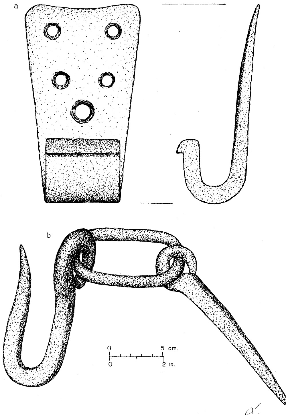
Fig. 151 -- Hooks from F523: a). hook (FOVA 27751) and b). hook, chain link and closed-eye nail (FOVA 27170).
