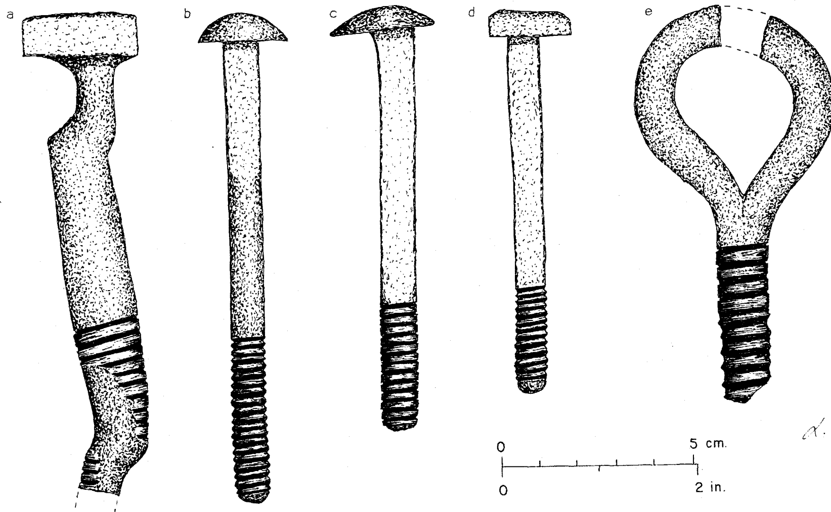
Fig. 116 -- Bolts and an eye bolt from F523: a). bolt (FOVA 28341); b). bolt (FOVA 27330); c). bolt (FOVA 27903); d). bolt (FOVA 28350) and e). closed eye bolt (FOVA 27168).
