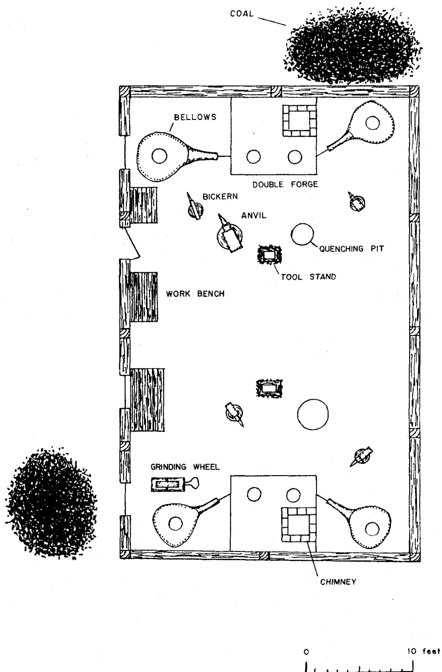
Fig. 243 -- Hypothetical reconstructed floor plan for the Blacksmith Shop (based upon currently available historical accounts together with in situ archaeological remains).
