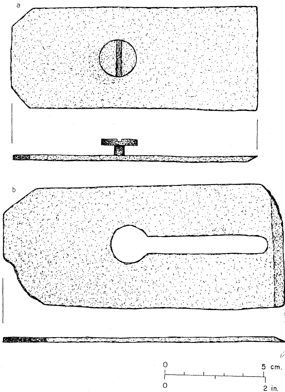
Fig. 53 -- Plane bits from the Blacksmith Shop area: a). plane bit (FOVA 34903) and b). plane bit (FOVA 34903).
