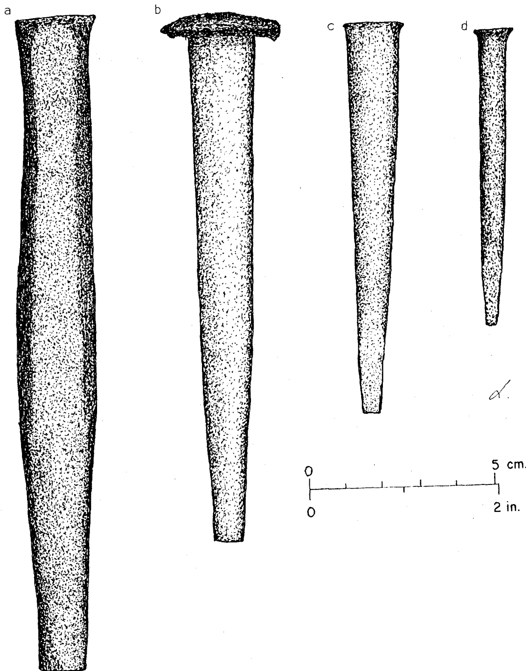
Fig. 61 -- Punches from the Blacksmith Shop area: a). punch (FOVA 35367); b). punch (FOVA 35891); c). punch (FOVA 35955) and d). punch (FOVA 34902).
