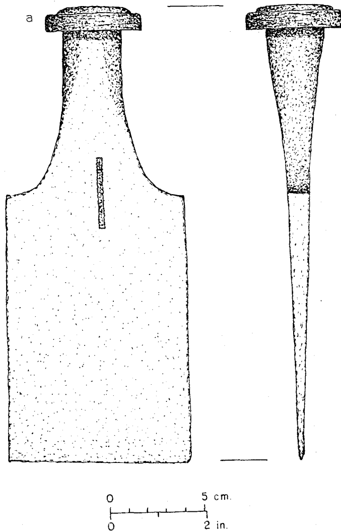
Fig. 126 -- Tools from F523: a). caulking tool (?) (FOVA 27615) and b). saw handle (FOVA 27390).
