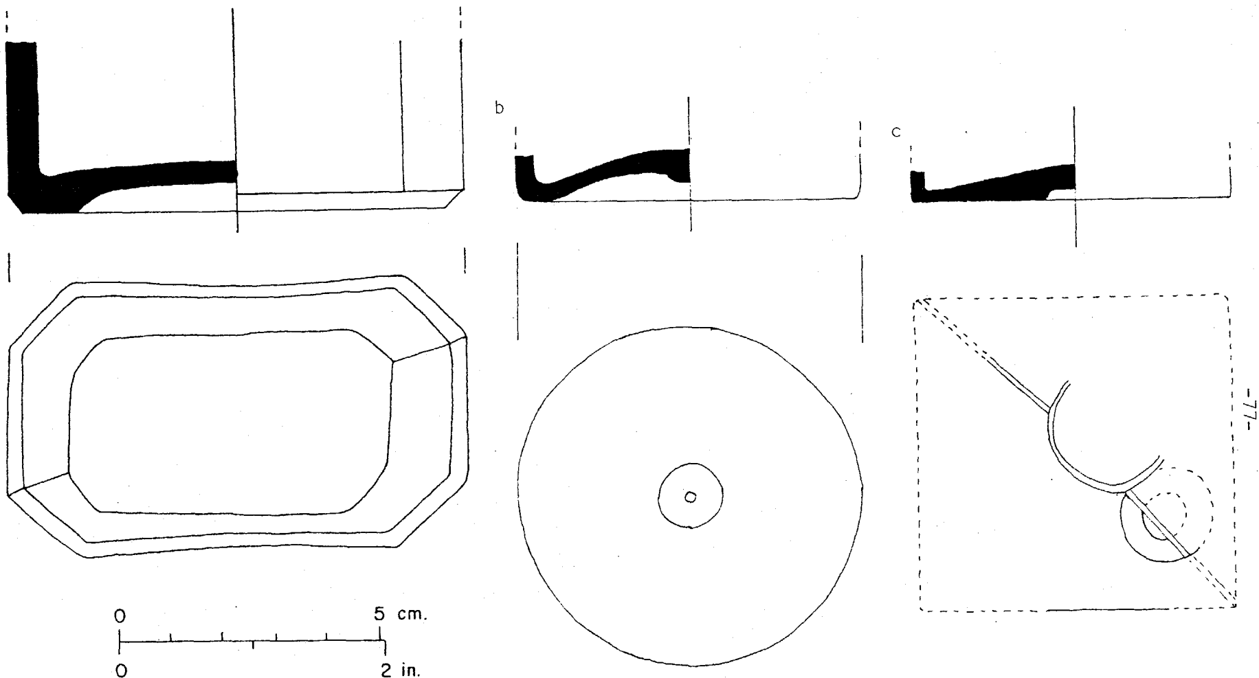
Fig. 24 -- Bottle base types found in the Blacksmith Shop area: a). base Type 65 (FOVA 34422); b). base Type 68 (FOVA 35336) and c). base Type 69 (FOVA 34243).
