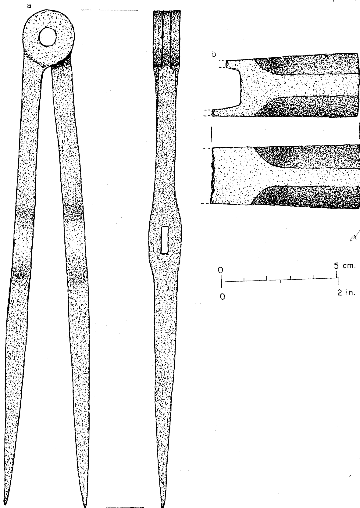
Fig. 50 -- Dividers and hammers from the Blacksmith Shop area: a). dividers (FOVA 35591) and b). hammer (FOVA 35831).
