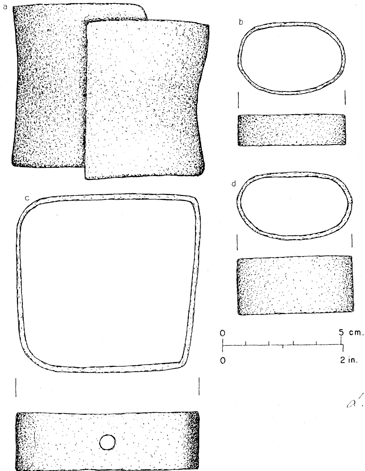
Fig. 158 -- Iron bands from F523: a). circular band securing tanged implement in wooden handle? (FOVA 28569); b). oval band (FOVA 27954); c). square band (FOVA 27326) and d). oval band (FOVA 27619).
