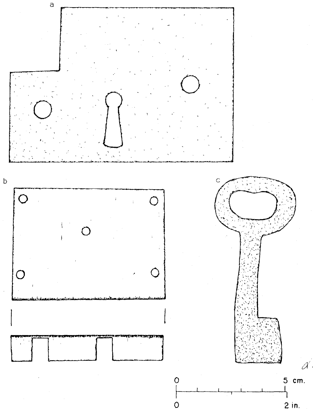
Fig. 31 -- A lock plate, furniture lock and a key preform from the Blacksmith Shop area: a). lock plate (FOVA 34074); b). furniture lock (FOVA 32805) and c). key preform (FOVA 33086).
