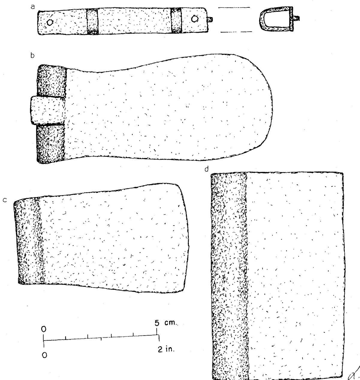
Fig. 28 -- A sliding bolt keeper and hinge preforms from the Blacksmith Shop area: a). sliding bolt keeper (FOVA 35634); b). hinge preform (FOVA 34187); c). hinge preform (FOVA 36073) and d). hinge preform (FOVA 34366).
