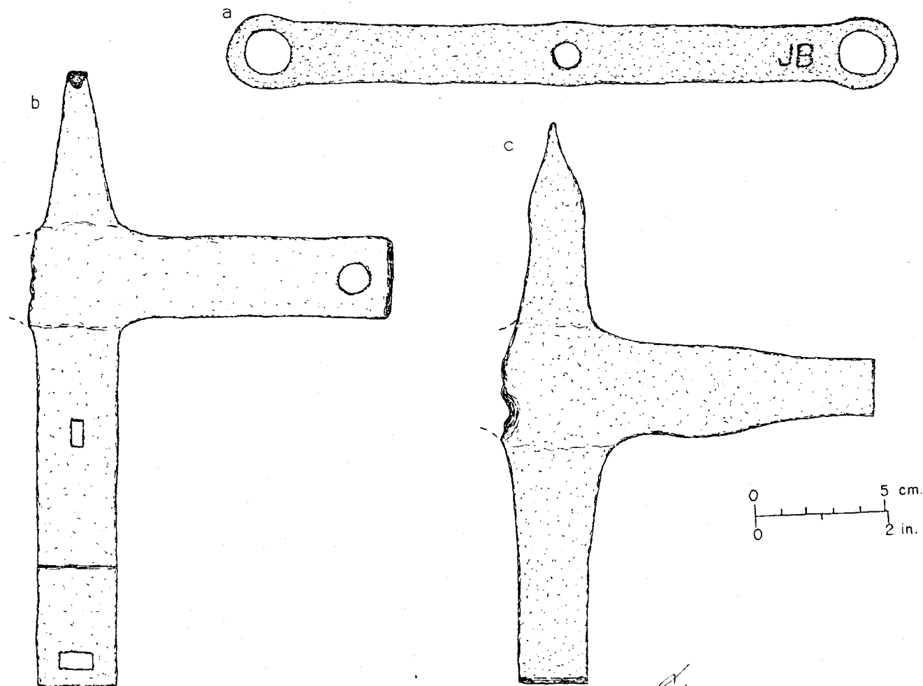
Fig. 138 -- Trap cross and base preforms from F523: a). trap cross (FOVA 28568); b). trap base preform (FOVA 27969) and c). trap base preform (FOVA 27967).
