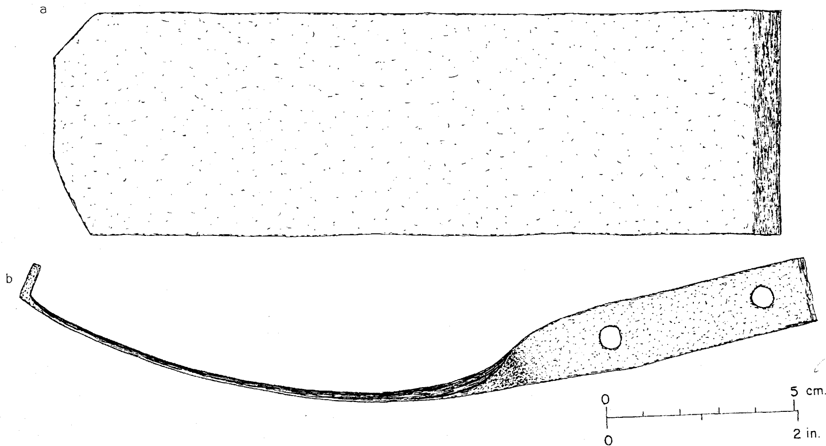
Fig. 127 -- Woodworking tools from F523: a). wood plane bit (FOVA 27973) and b). drawknife (FOVA 27973).
