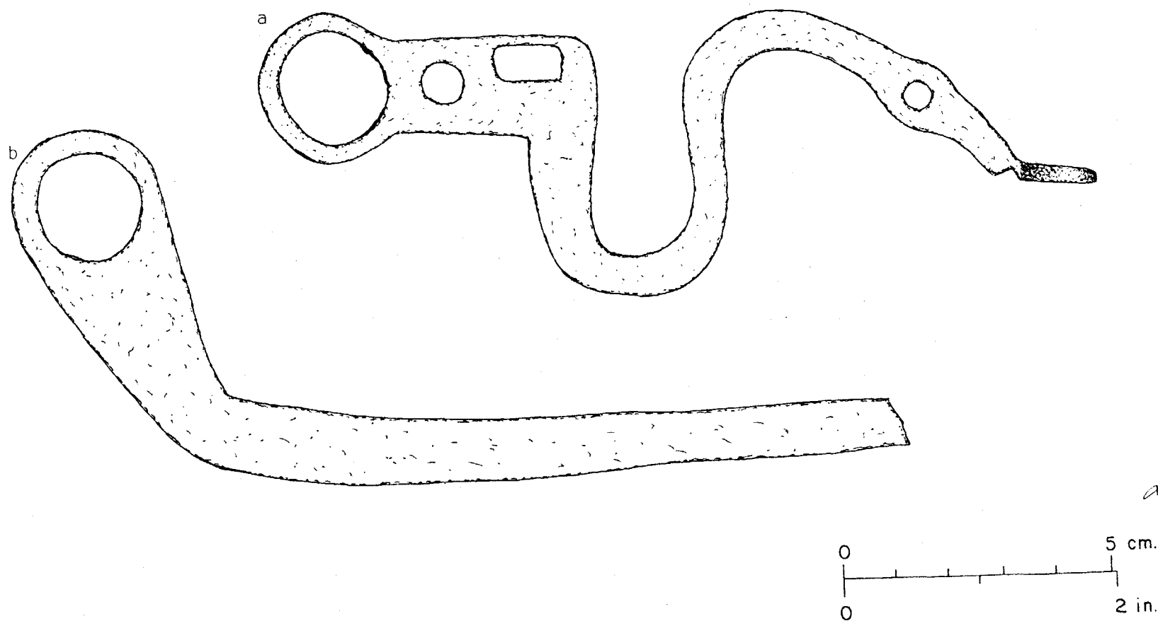
Fig. 79 -- Horse bit cheek strap and preform from the Blacksmith Shop area: a). horse bit cheek strap (FOVA 34554) and b). horse bit cheek strap preform (FOVA 35476).
