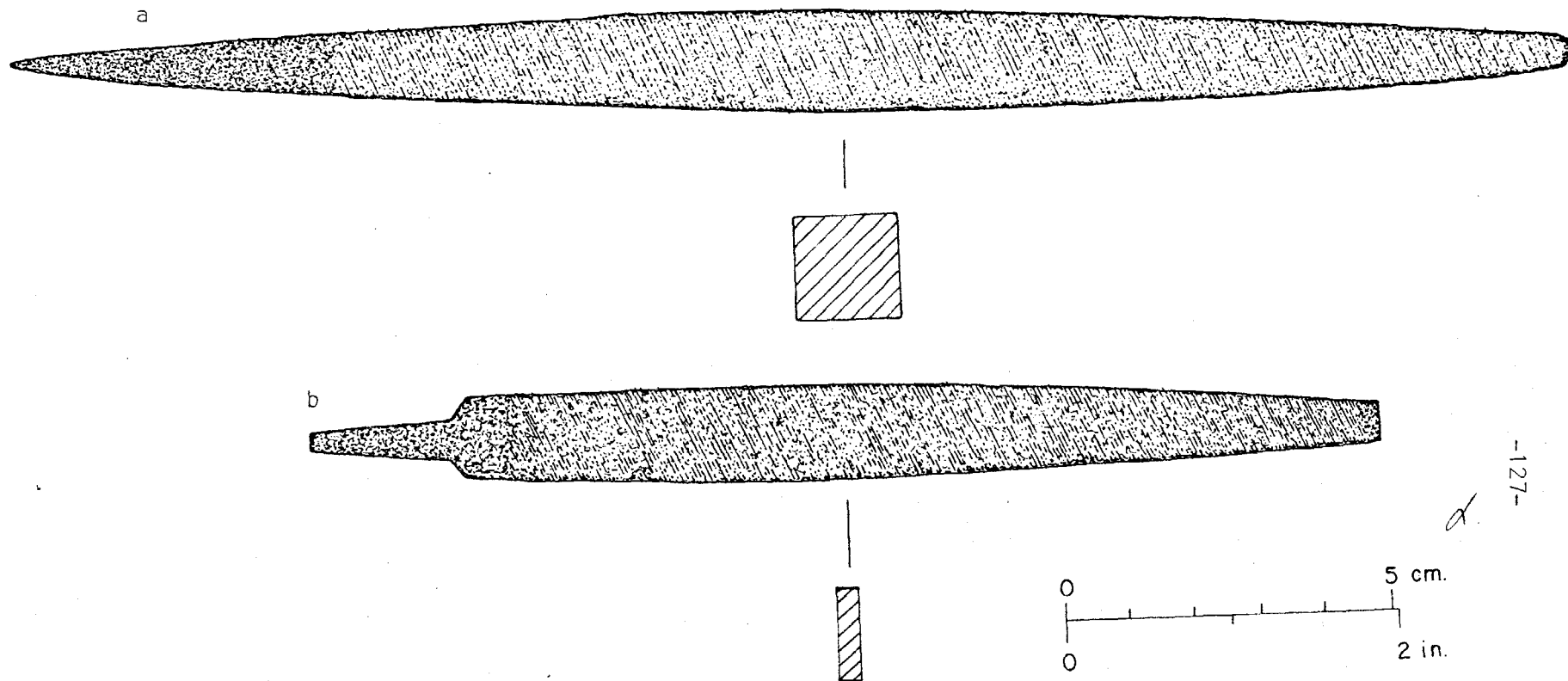
Fig. 58 -- Files from the Blacksmith Shop area: a). file (FOVA 32811) and b). file (FOVA 35369).
