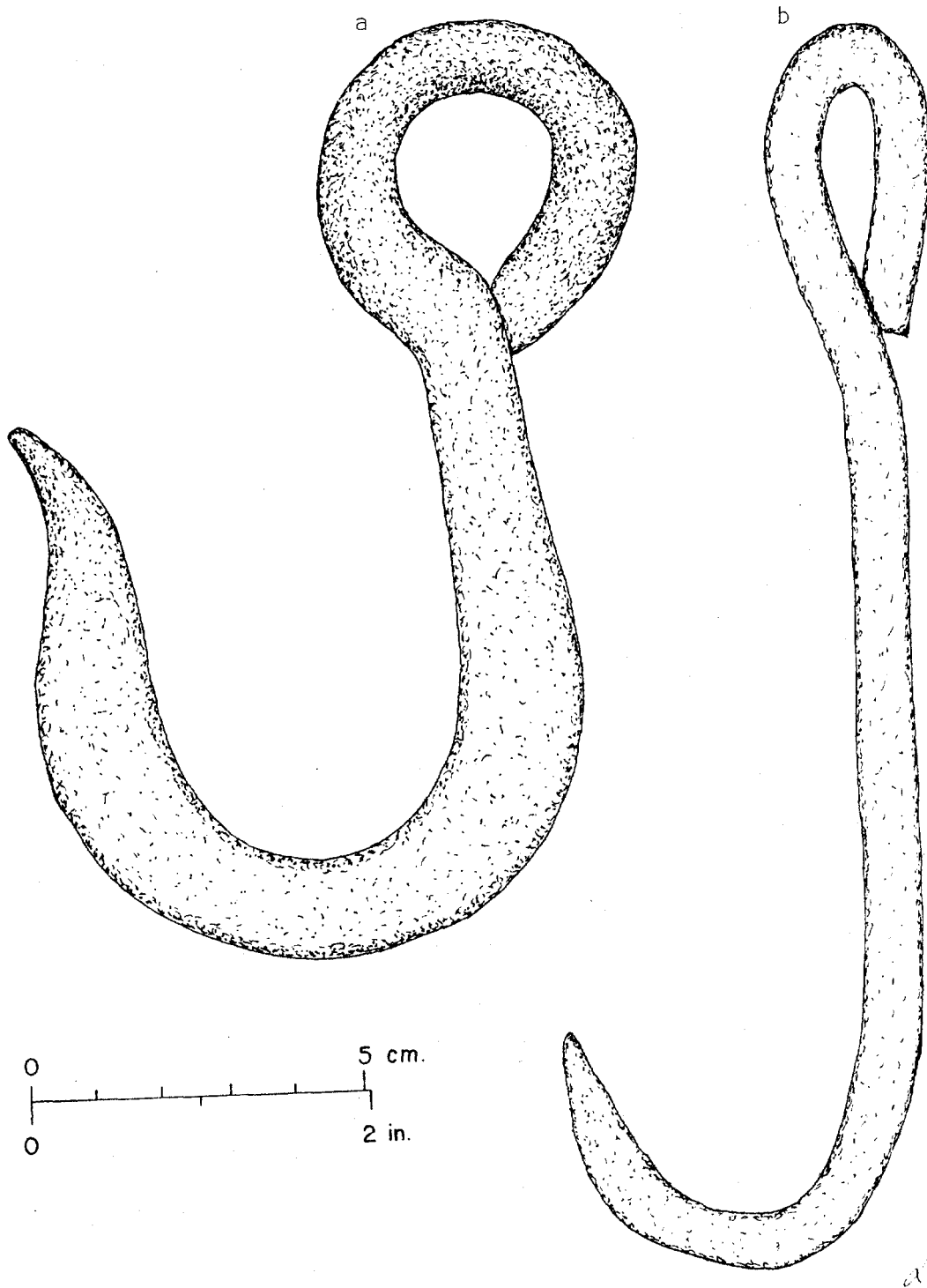
Fig. 83 -- Hooks from the Blacksmith Shop area: a). reconstructed hook (FOVA 34445) and b) hook (FOVA 34198).
