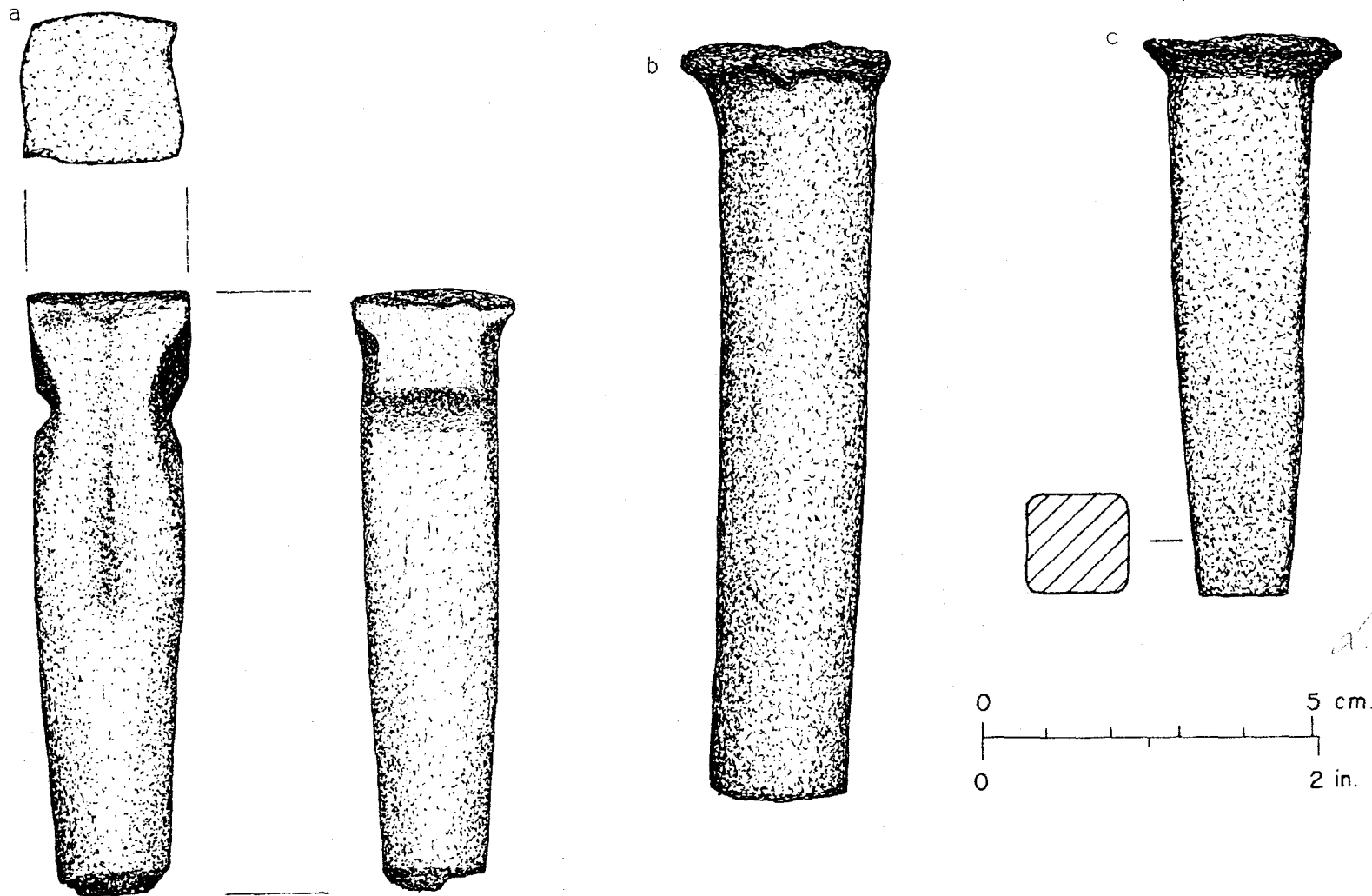
Fig. 62 -- Punches from the Blacksmith Shop area: a). punch (FOVA 34376); b). punch (FOVA 34902) and c). punch (FOVA 33240).
