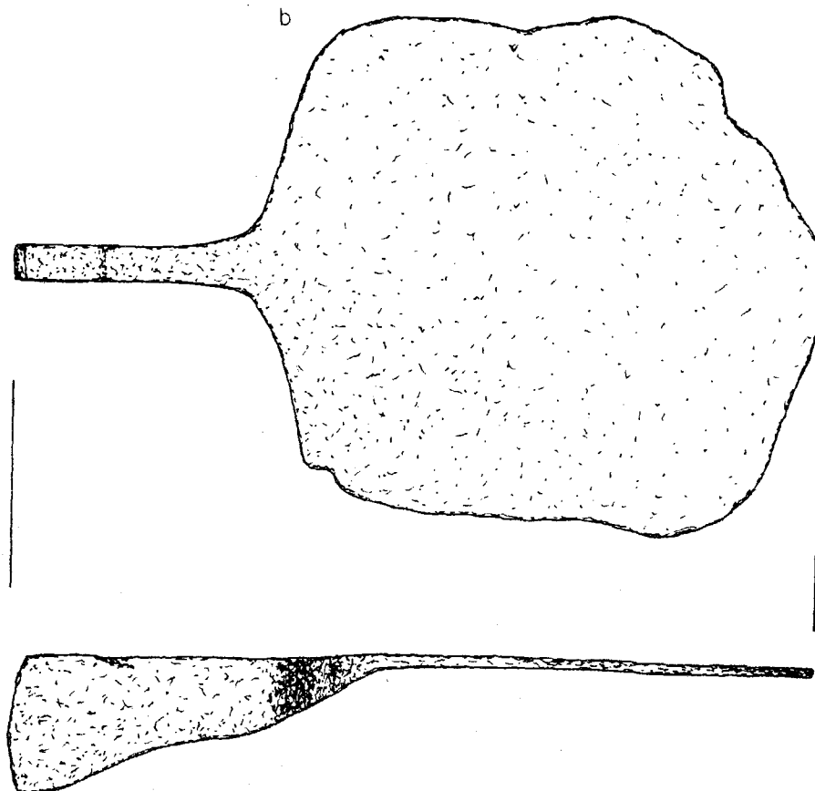
Fig. 71 -- Pan and preform from the Blacksmith Shop area: a). pan (FOVA 35363) and b). pan preform (FOVA 32301).
