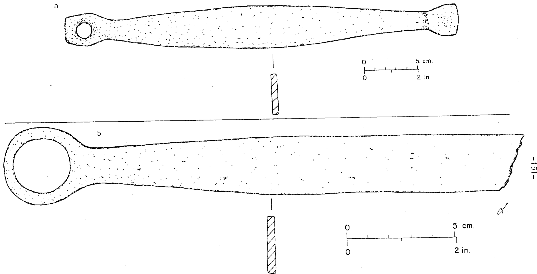
Fig. 76 -- Spring preforms from the Blacksmith Shop area: a). spring preform (FOVA 35470) and b). spring preform (FOVA 32655).
