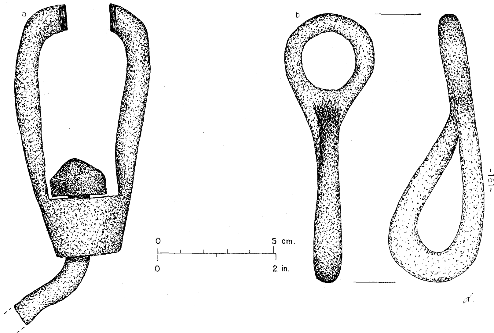
Fig. 82 -- Swivel chain link and reconstructed hook from the Blacksmith Shop area: a). swivel chain link (FOVA 34299) and b). reconstructed hook (FOVA 32812).
