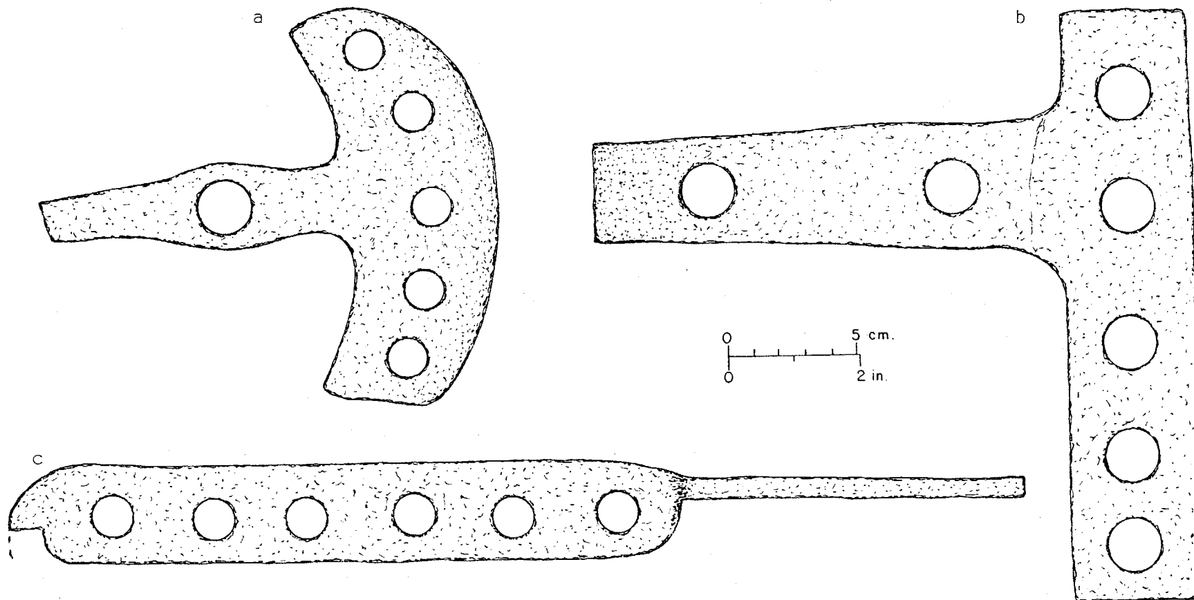
Fig. 147 -- Adjustable clevises and preform from F523: a). adjustable clevis (FOVA 27993); b). adjustable clevis (FOVA 28545); and c). adjustable clevis preform (FOVA 28195).
