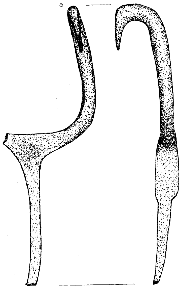
Fig. 63 -- Unid. implement and swage from the Blacksmith Shop area: a). Unidentified implement (FOVA 34557) and b). swage (FOVA 34186).
