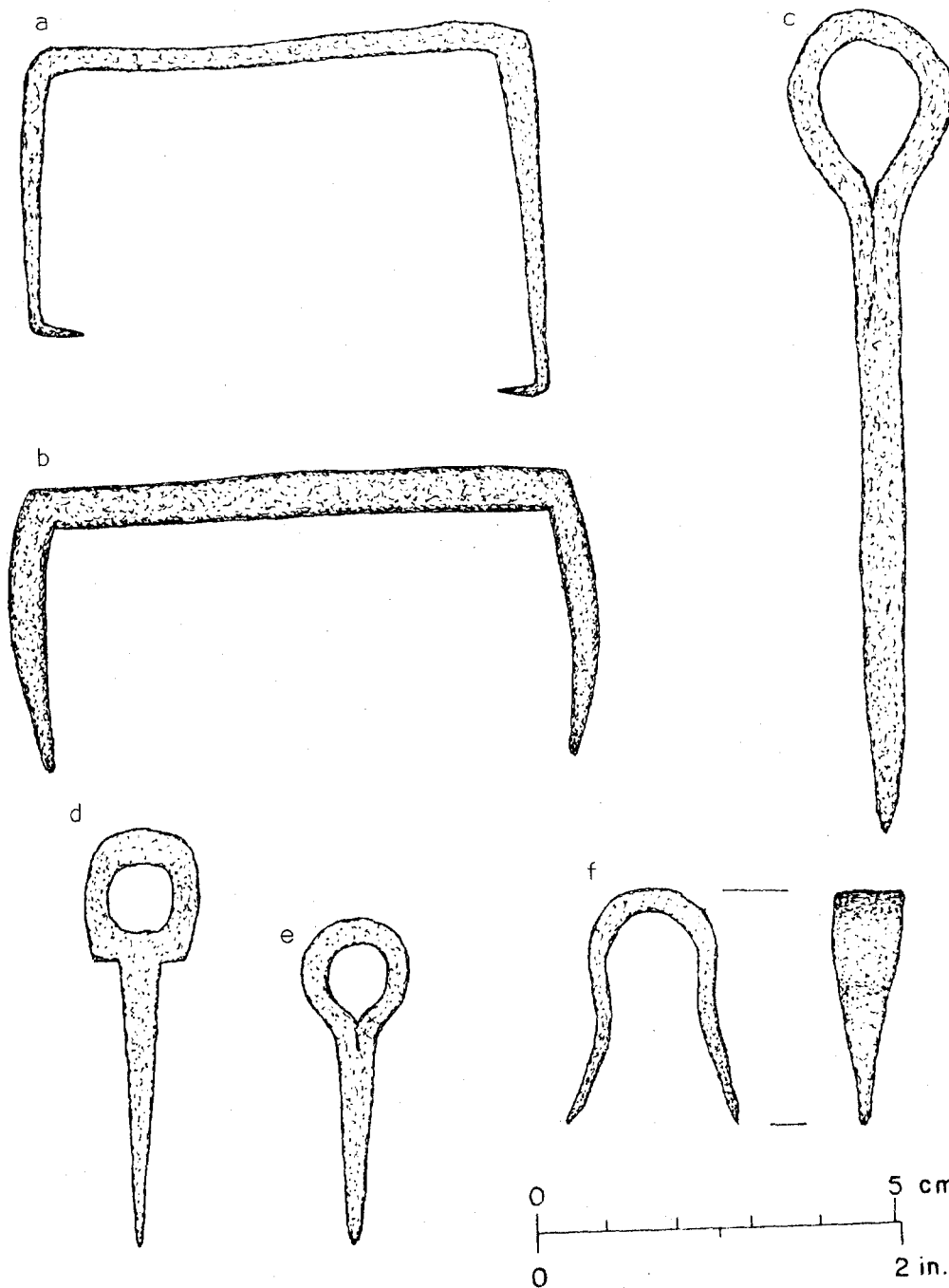
Fig. 40 -- Staples and closed eye nails from the Blacksmith Shop area: a). staple (FOVA 34873); b). staple (FOVA 35532); c). closed eye nail (FOVA 33261); d). closed eye nail (FOVA 34115); e). closed eye nail (FOVA 34115) and f). staple (FOVA 35259).
