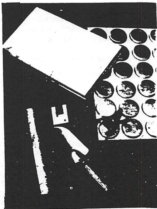
Figure 1.—A carrying case for sample cans should hold the samples securely. A covered notebook, clippers, trowel, ruler, and fuel gage are standard sampling equipment.
