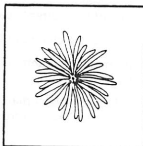
Figure 17.—If new growth is not completely separated from the 1-year-old stem and needles, the center of the new stem will be obvious. Carefully remove the new growth.
