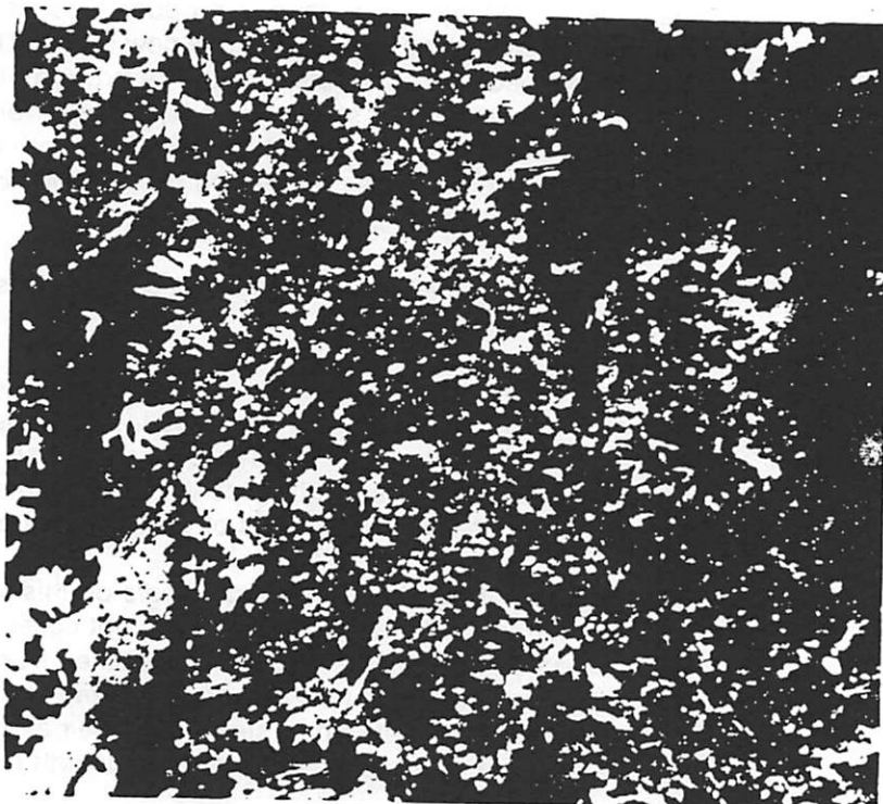
Figure 11.—Because sphagnum moss has a very dense growth form that allows it to retain free water, it rarely dries enough to burn and therefore should not be included in the feathermoss and lichen sample.
