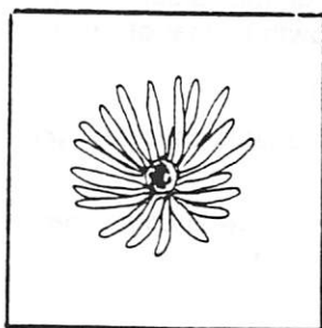
Figure 16.—If all new needle and stem growth is removed from the end of the branch, a brown concave scar, marking the end of the previous year's growth, should be evident.
