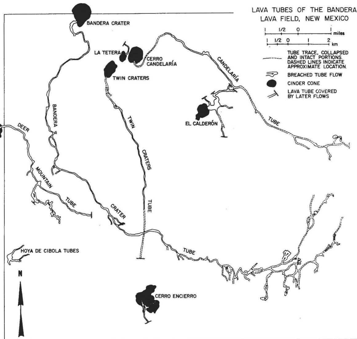
Figure 4-3: Lava tube systems of the Bandera lava field. (Ariz.fig.11)
