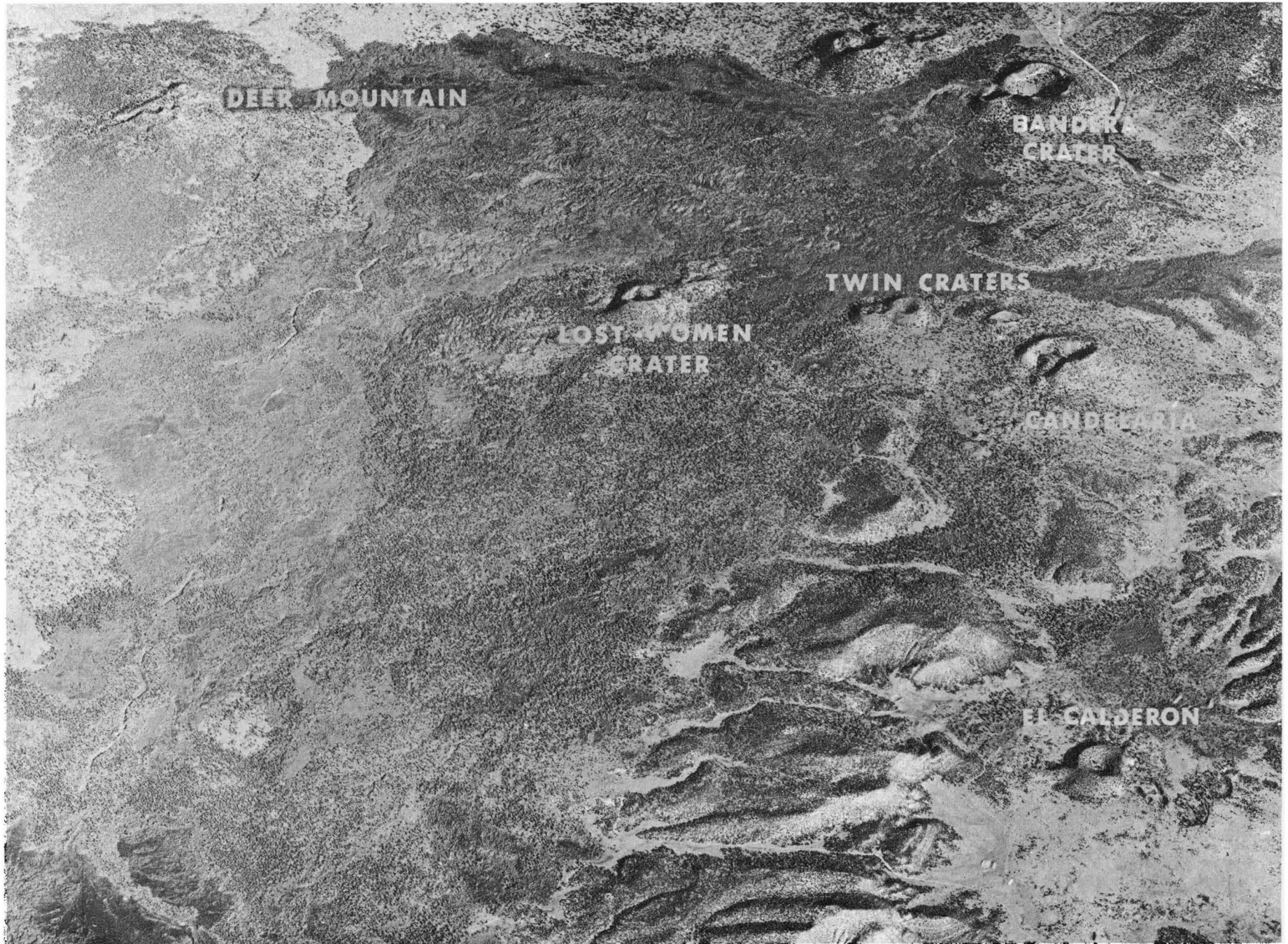
Low oblique aerial photograph of the Bandera lava field showing principal craters and collapsed lava tubes. The view is to the NW with foreground about 8 km across. (U.S. Govt. Photo, 1965).
