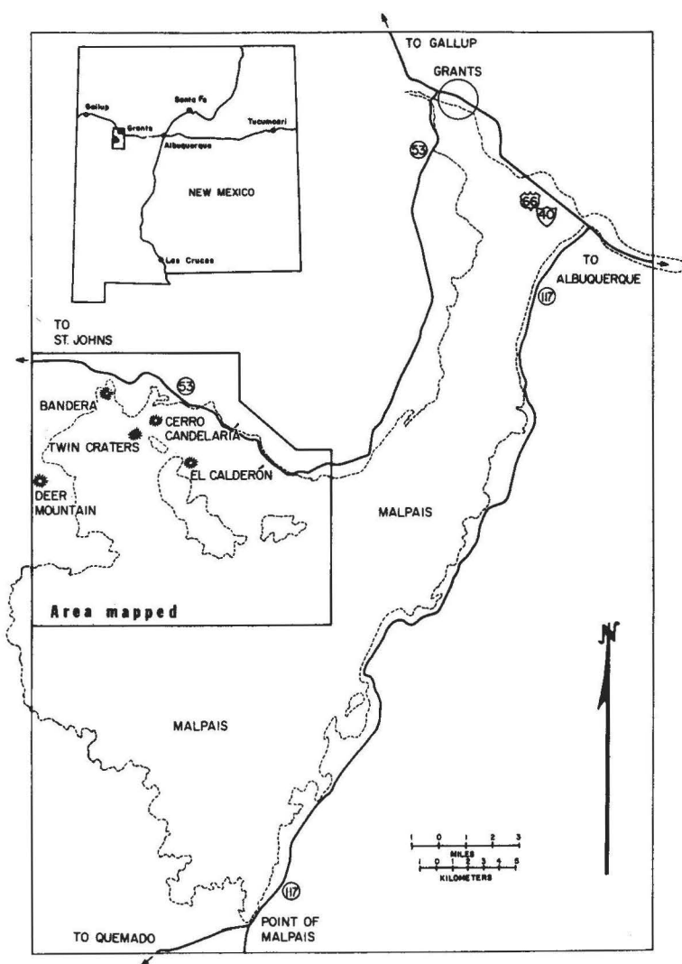
Figure 4-1: Index map to the Bandera lava field. Basalts of Pleistocene and Holocene age are outlined by the dashed line; they overlie in part older volcanics. (Ariz.fig.2)
