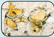
Carbonate globules in Martian meteorite ALH84001 that are the site of suggested biological signatures.
