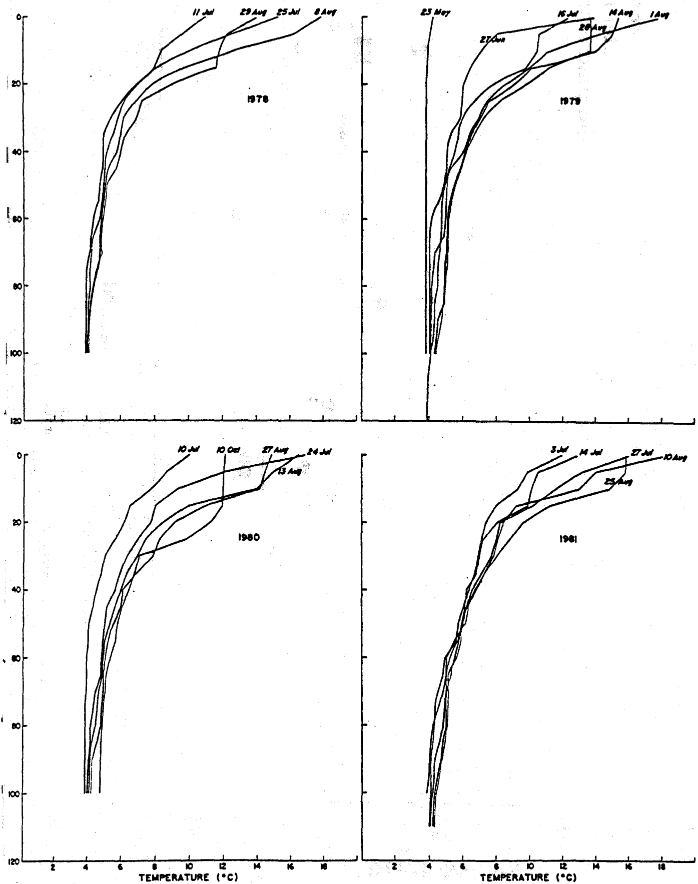
Figure 3. Thermal profiles for Crater Lake, 1978-1981.
