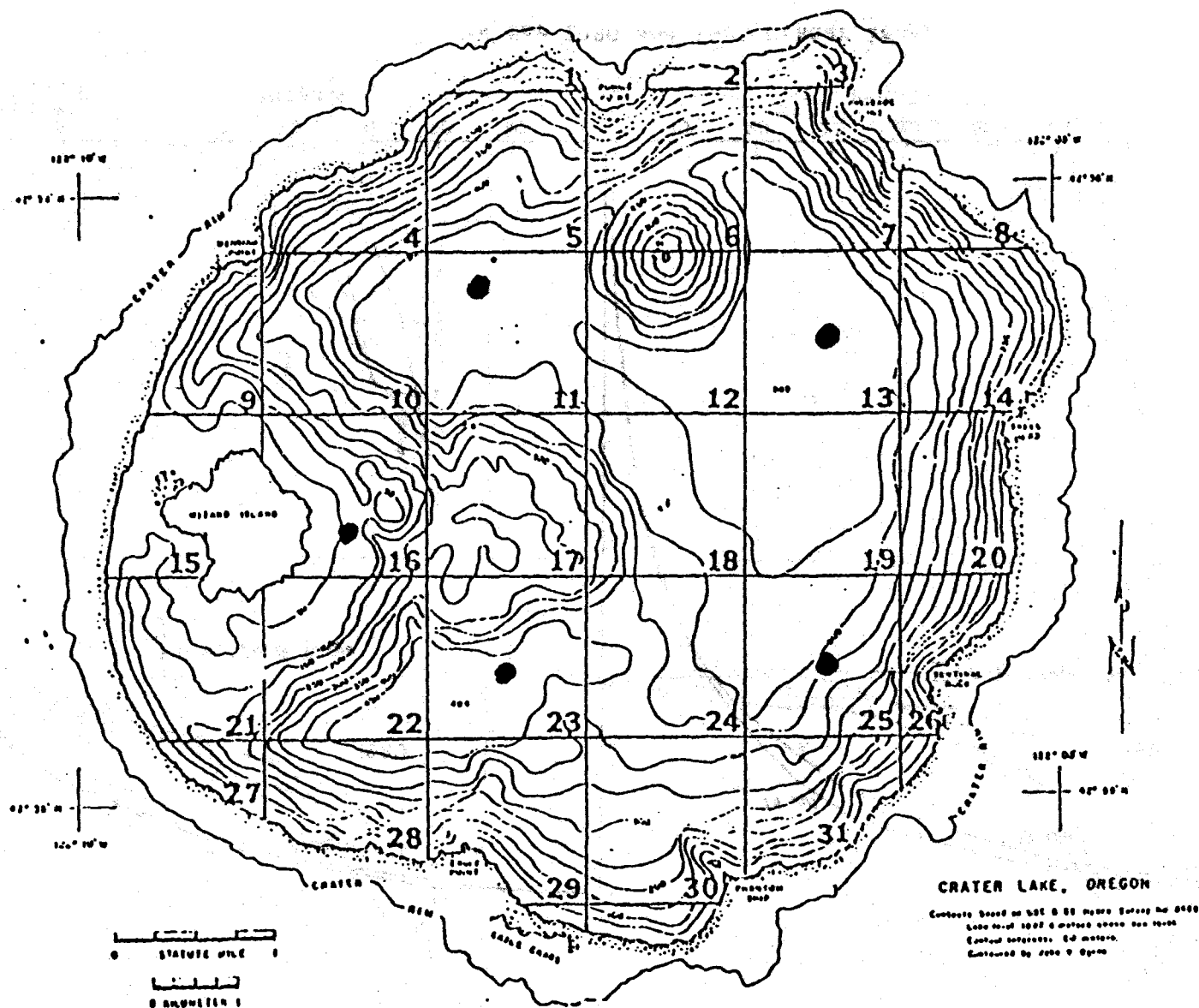
Figure 1. Lakewater sampling locations at stations 11, 13, 16, 23, and 25.
