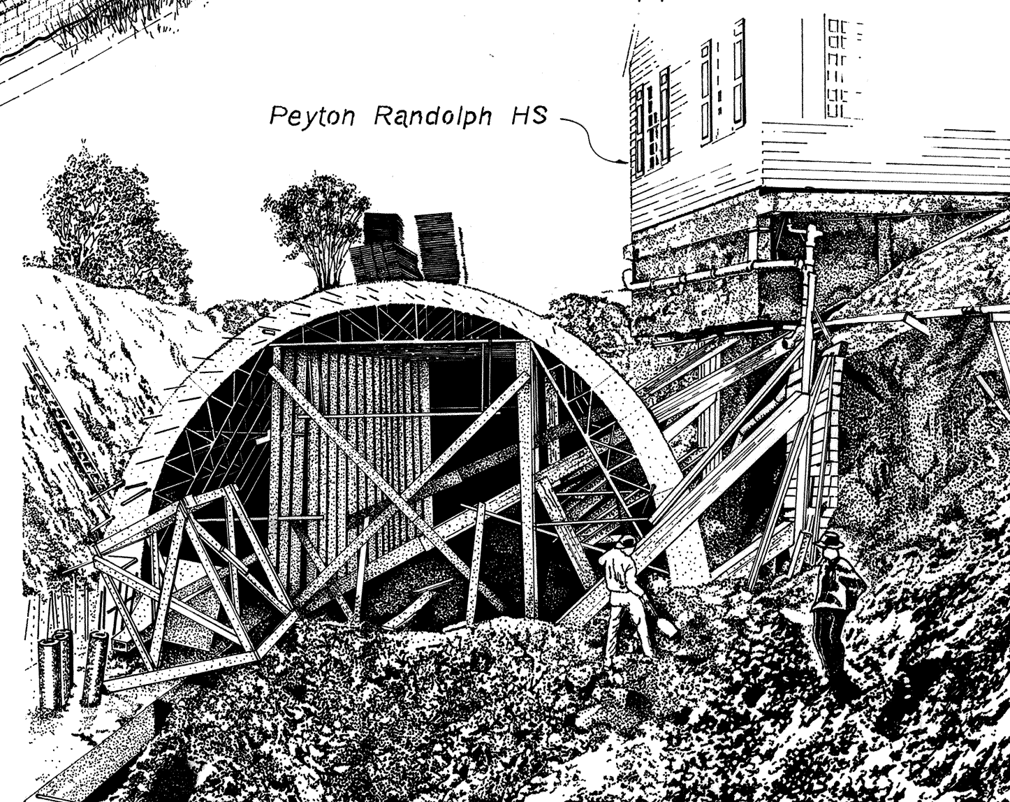
CONSTRUCTION OF TUNNEL ADJACENT TO HISTORIC STRUCTURE
