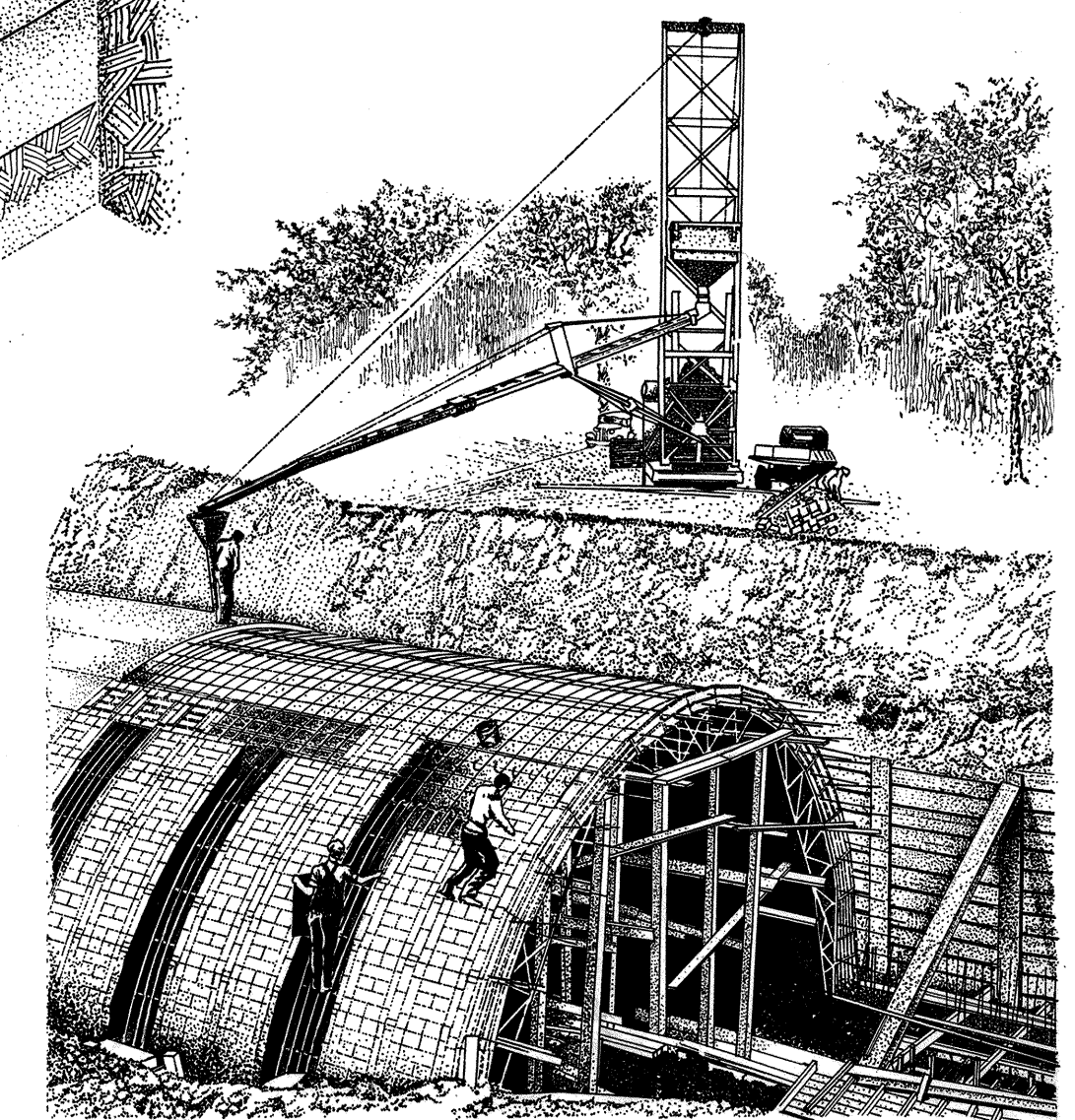
PLACEMENT OF CONCRETE
