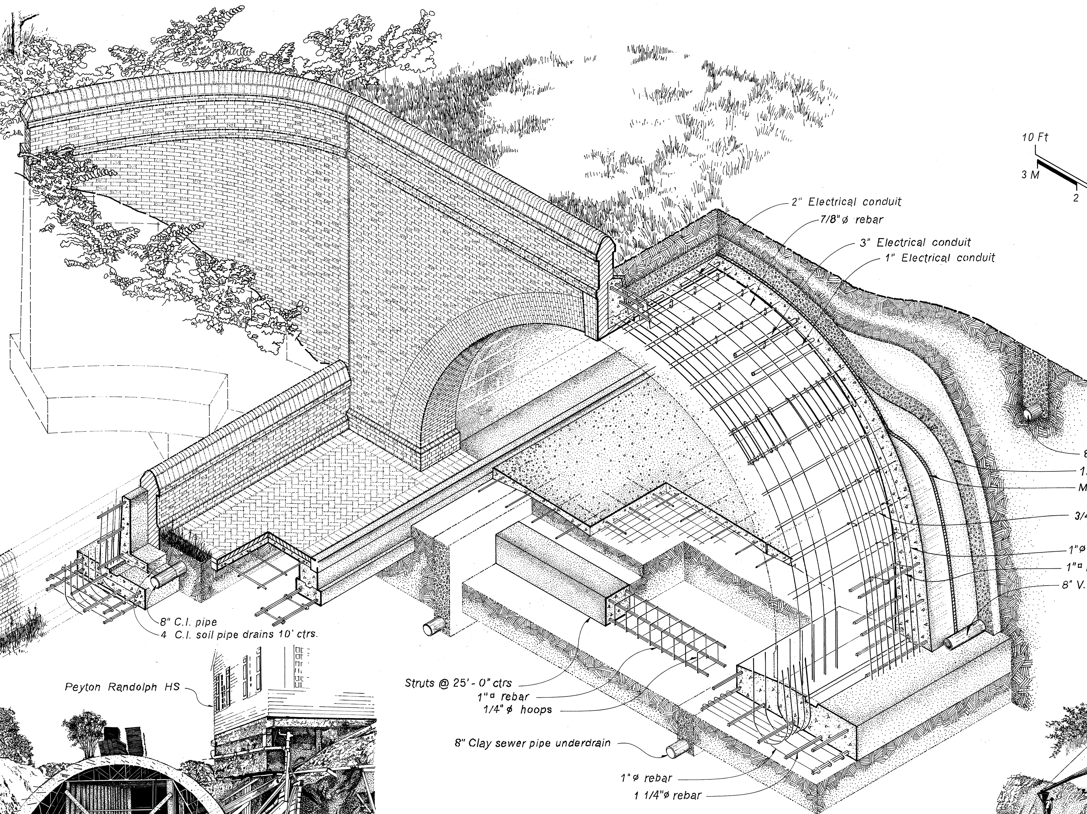
SHORING OF TUNNEL EXCAVATION
