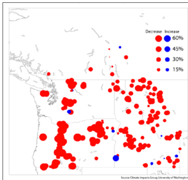
Figure 30. Trends in April 1 SWE, 1950–2000. Increases (decreases) are indicated with blue (red) dots, and the size of the dot corresponds to the magnitude of the change. Pluses and minuses indicate increases or decreases, respectively, that are less than the given scale. Source: Climate Impacts Group, University of Washington.
