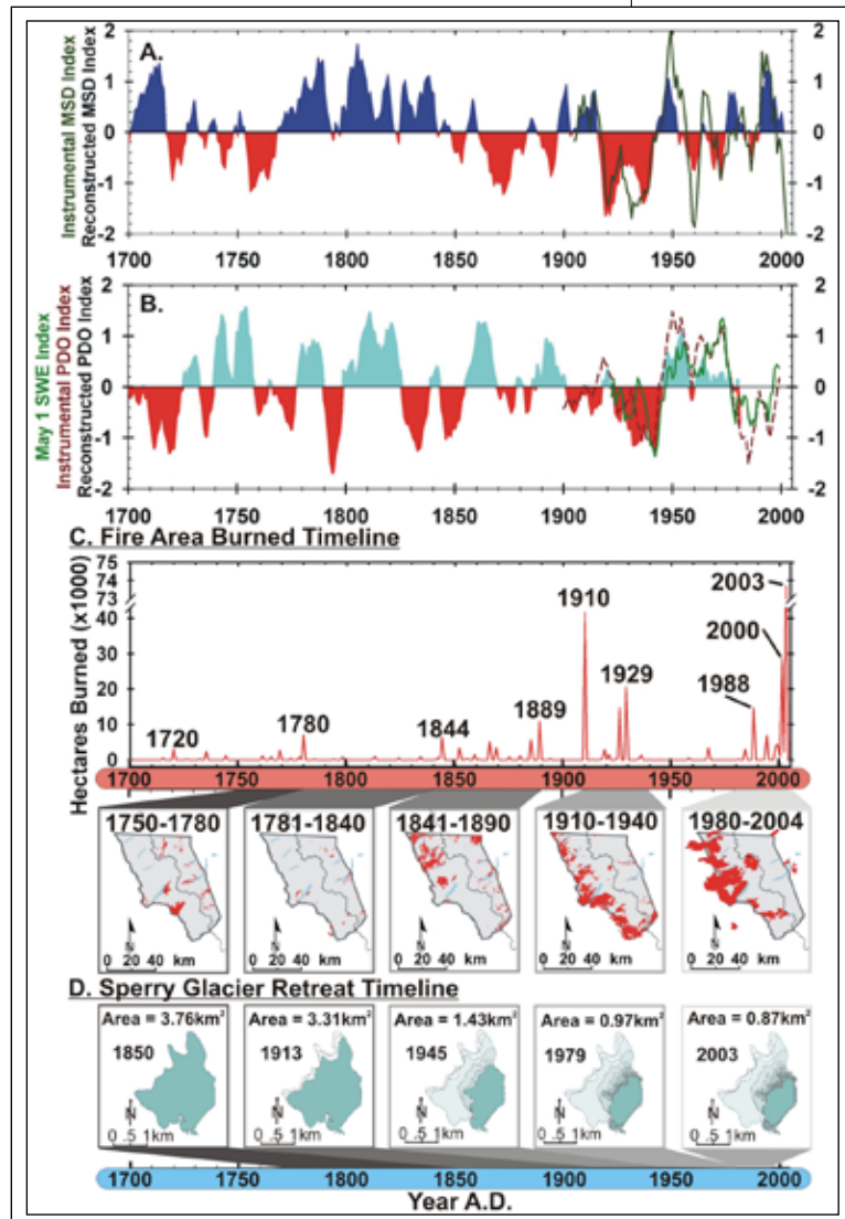
Figure 14. Relationship between Glacier National Park summer drought, inferred winter snowpack, fire area burned, and glacial recession 1700 to present. (a) Instrumental and reconstructed summer drought (MSD) normalized by converting to units of standard deviation and smoothed using a 5-year running mean. (b) Measured spring snowpack (May 1 SWE) anomalies (1922–present) and average annual instrumental and reconstructed PDO anomalies. Each time series was normalized and smoothed using a 5-year running mean. For ease of comparison, the instrumental and reconstructed PDO index was inverted due to the strong negative relationship between PDO anomalies and May 1 snowpack. (c) Fire area burned timeline for the GNP region. Timeline is presented with maps of fire activity during periods of interesting winter and summer precipitation regimes. (d) Maps showing the decrease in area of the Sperry Glacier at critical points from 1850 to 2003. The retreat patterns of the Sperry Glacier are representative of regional patterns of recession for glaciers sensitive to regional climate variability. Source: Pederson et al. 2006, American Meteorological Society; reprinted with permission.
