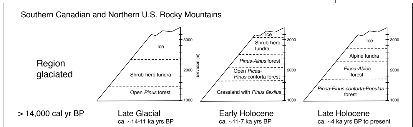
Figure 5. Ecological response to changing climatic conditions following glacial retreat in the southern Canadian and northern U.S. Rockies. Derived from MacDonald 1989 and Reasoner and Hickman 1989 (Whitlock unpublished).
