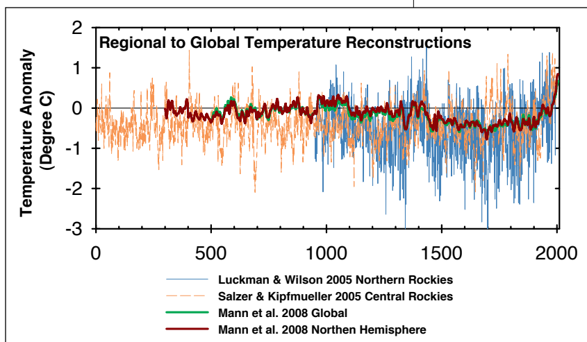
Figure 12. Comparison of regional and global temperature reconstructions. Derived from Luckman and Wilson 2005, Salzer and Kipfmüller 2005 (both based on tree-ring records), and Mann et al. 2008 (based on a multi-proxy reconstruction).
