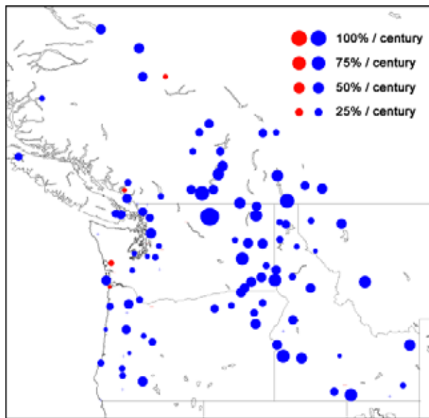
Figure 29. Trends in average annual precipitation, 1920–2000. Increases (decreases) are indicated with blue (red) dots, and the size of the dot corresponds to the magnitude of change. Source: Climate Impacts Group, University of Washington.
