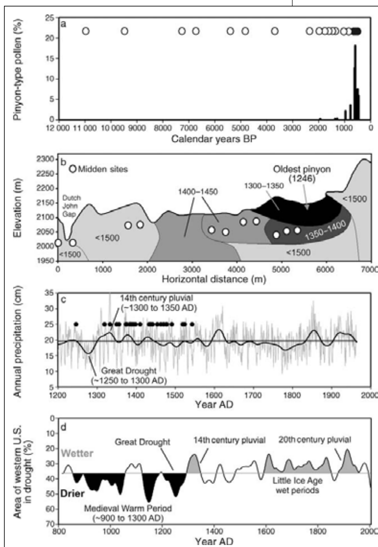
Figure 17. Establishment and presence/absence of pinyon pine in relation to climate variability and elevation during the Holocene. (a) Percentages of pinyon-type pollen (black vertical bars) and presence (solid circles) or absence (open circles) of pinyon pine macrofossils from 12,000 years of woodrat midden records collected in the DJM. (b) Map of the study area showing locations of midden sites (open circles) and sampling units used in the tree-ring age studies (shaded polygons). Each midden site is a cave or rock overhang where one or more of the 60 middens were collected. The estimated establishment dates are based on the average age of the four oldest pinyons found in each sampling unit. (c) Ages for the oldest pinyon on DJM and the four oldest pinyons in each of the eight sampling units (black dots) plotted against reconstructed annual (gray line) and 30-year smoothed (black line) precipitation values for the Uinta Basin Region. (d) Percentage of the western United States experiencing drought conditions during the last 1200 years as reconstructed from a large tree-ring network (Cook et al. 2004). Data are plotted as a 50-year moving average. The horizontal line at 37% (dark gray) shows the average or background level of drought through time. Significant multidecadal dry and wet periods identified by Cook et al. (2004) are shaded black and gray, respectively. Source: Gray et al. 2006; reprinted with permission.
