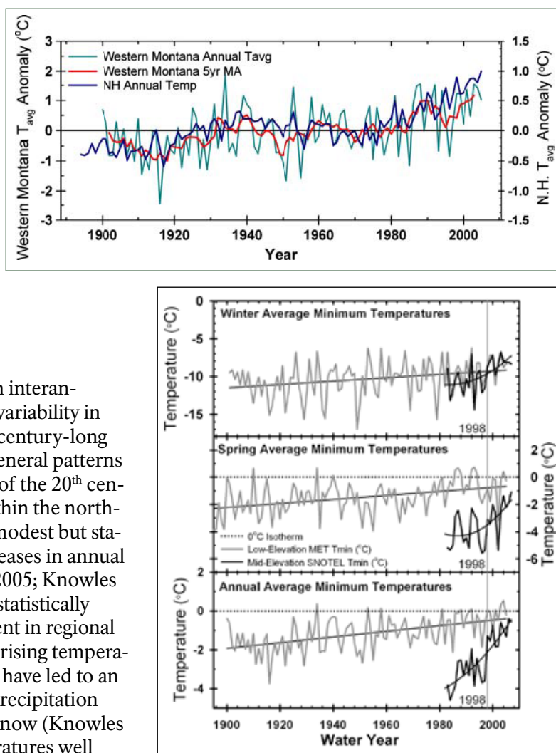
Figure 23. Comparison of variability and trends in western Montana (blue-green line) and Northern Hemisphere (dark blue line) annual average temperatures. A 5-year moving average (red line) highlights the similarity in trends and decadal variability between records. Source: Pederson et al. 2010; reprinted with permission.
