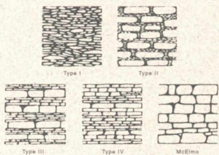
Wall facings
