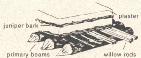
Roof construction
