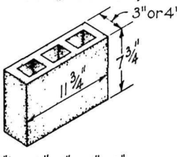
8" x 3" or 4" x 12"
