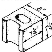
Half block
