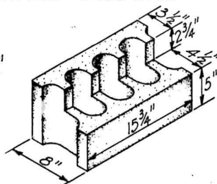
Header block
