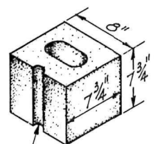
Pier or double corner block
