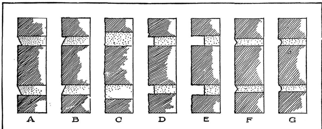
Common types of joints. (a) struck joint, (b) weathered joint, (c) flush or plain cut joint (d) raked joint, (e) stripped joint, (f) "V" joint, (g) concave joint.
