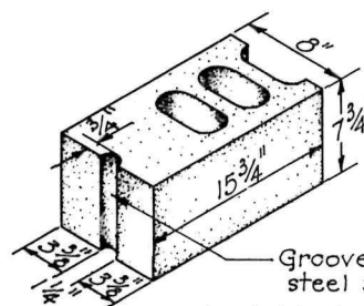
Jamb block for steel sash
