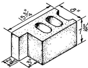
Jamb block for wood sash also used as joist block
