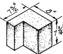
Jamb block for wood sash also used as joist block
