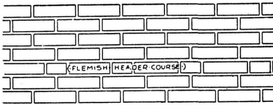
COMMON BOND
