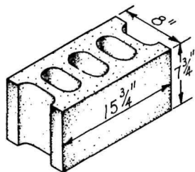
Three Core 8" x 8" x 16"
