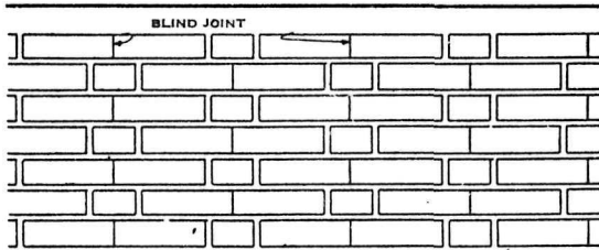
DOUBLE STRETCHER FLEMISH BOND
