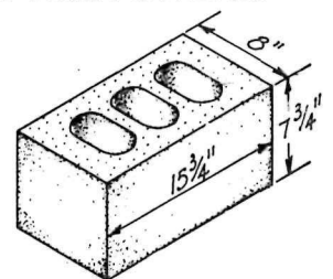
Pier or double corner block
