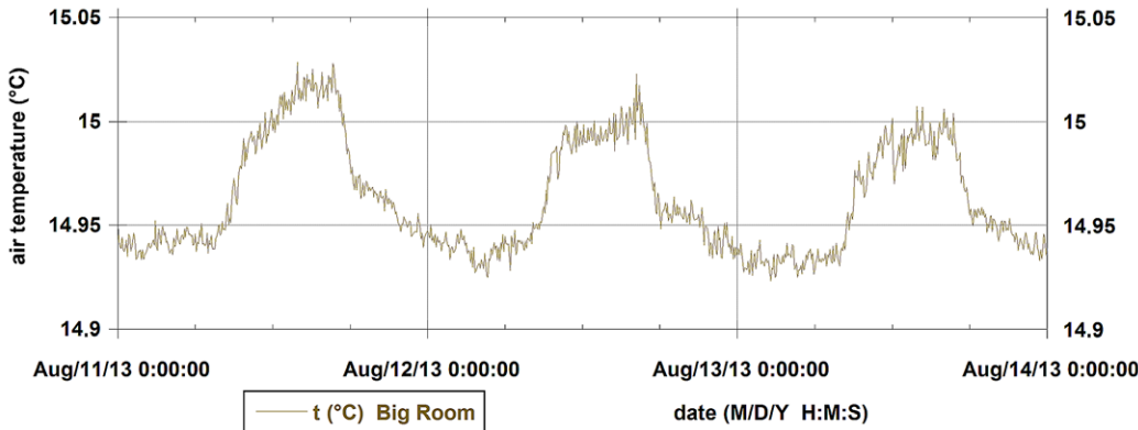
Figure 14. Record of the air temperature in the Big Room inside Carlsbad Cavern on an expanded scale from August 11 through August 13, 2013, recorded every 5 minutes.
