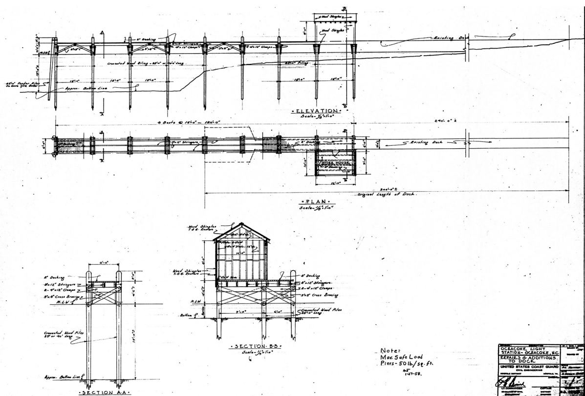
FIGURE 2-110. Repair/addition plans, 1958. (NPS/CAHA Collection)
