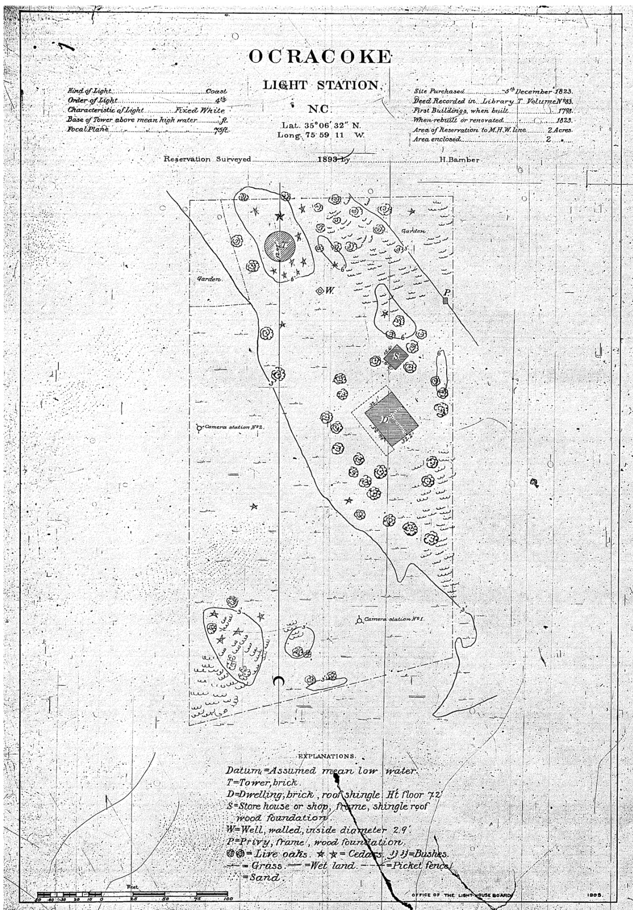
FIGURE B-6. Ocracoke Light Station site plan, 1893. (NPS/CAHA Collection)
