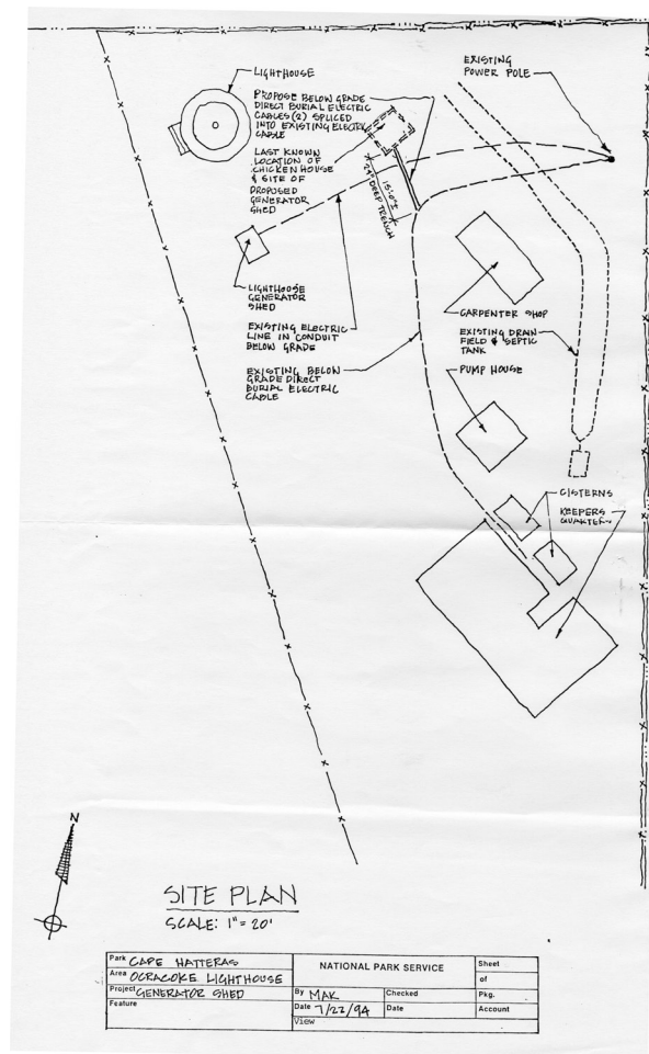
FIGURE 2-46. Site plan showing new generator shed in location of chicken house, 1994. (NPS/CAHA Collection)
