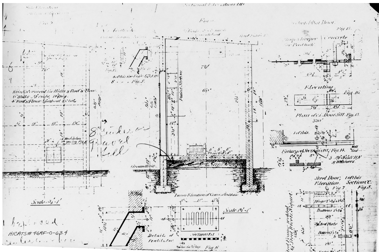
FIGURE 2-87. Concrete oil house drawing, 1913. (NPS/CAHA Collection)
