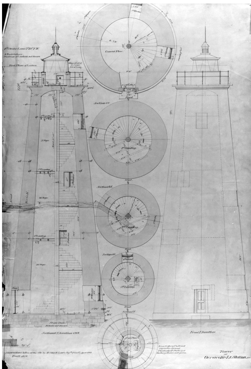
FIGURE 2–68. Lighthouse plan, 1892. (NPS/CAHA Collection)
