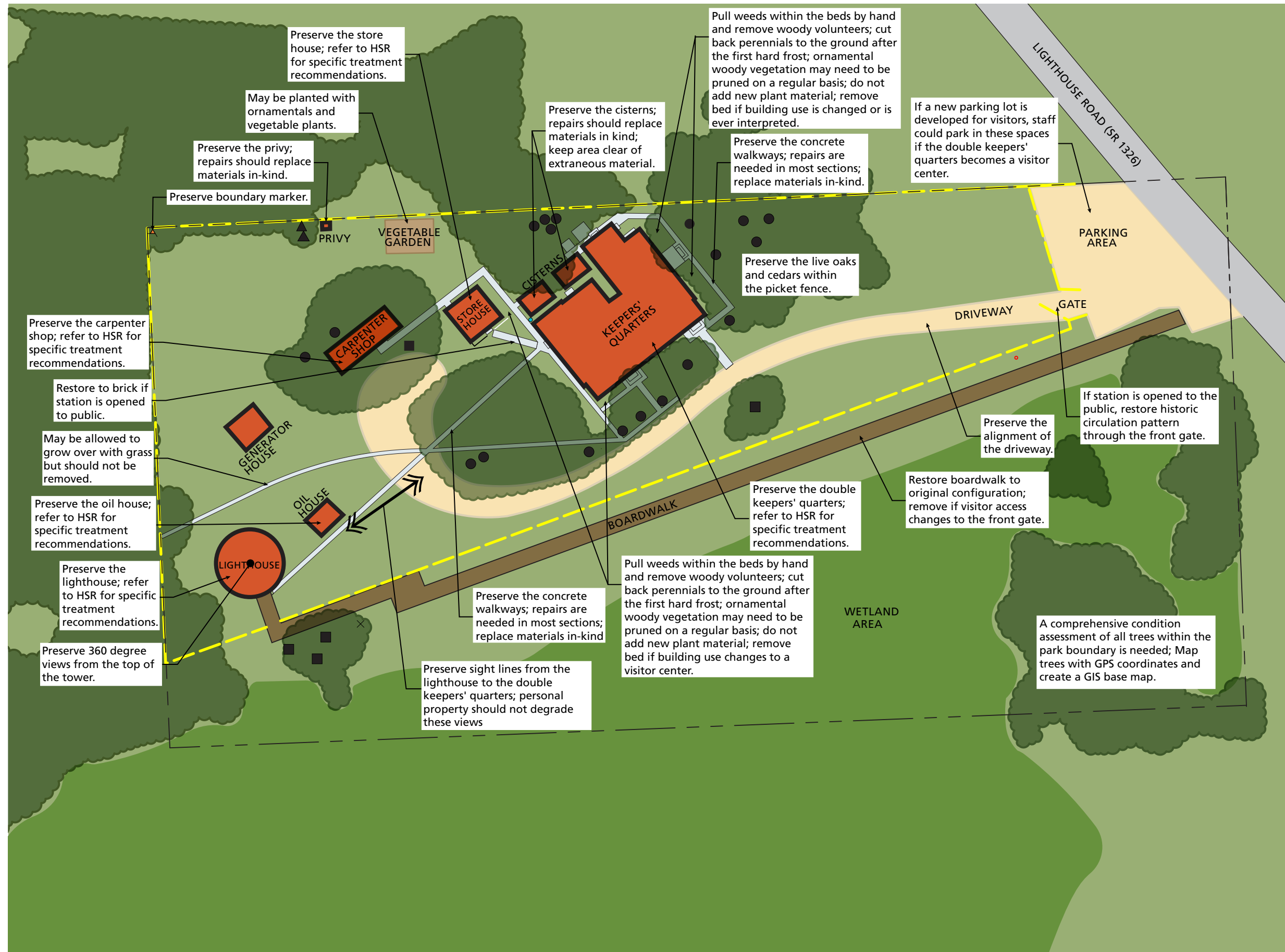
FIGURE 5-24. Ocracoke Light Station Treatment Map
