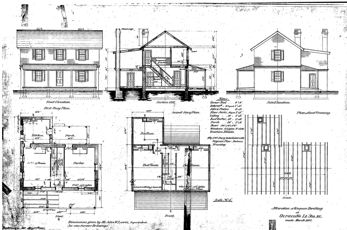
FIGURE 2-81. Plan of second story addition, 1897. (NPS/CAHA Collection)
