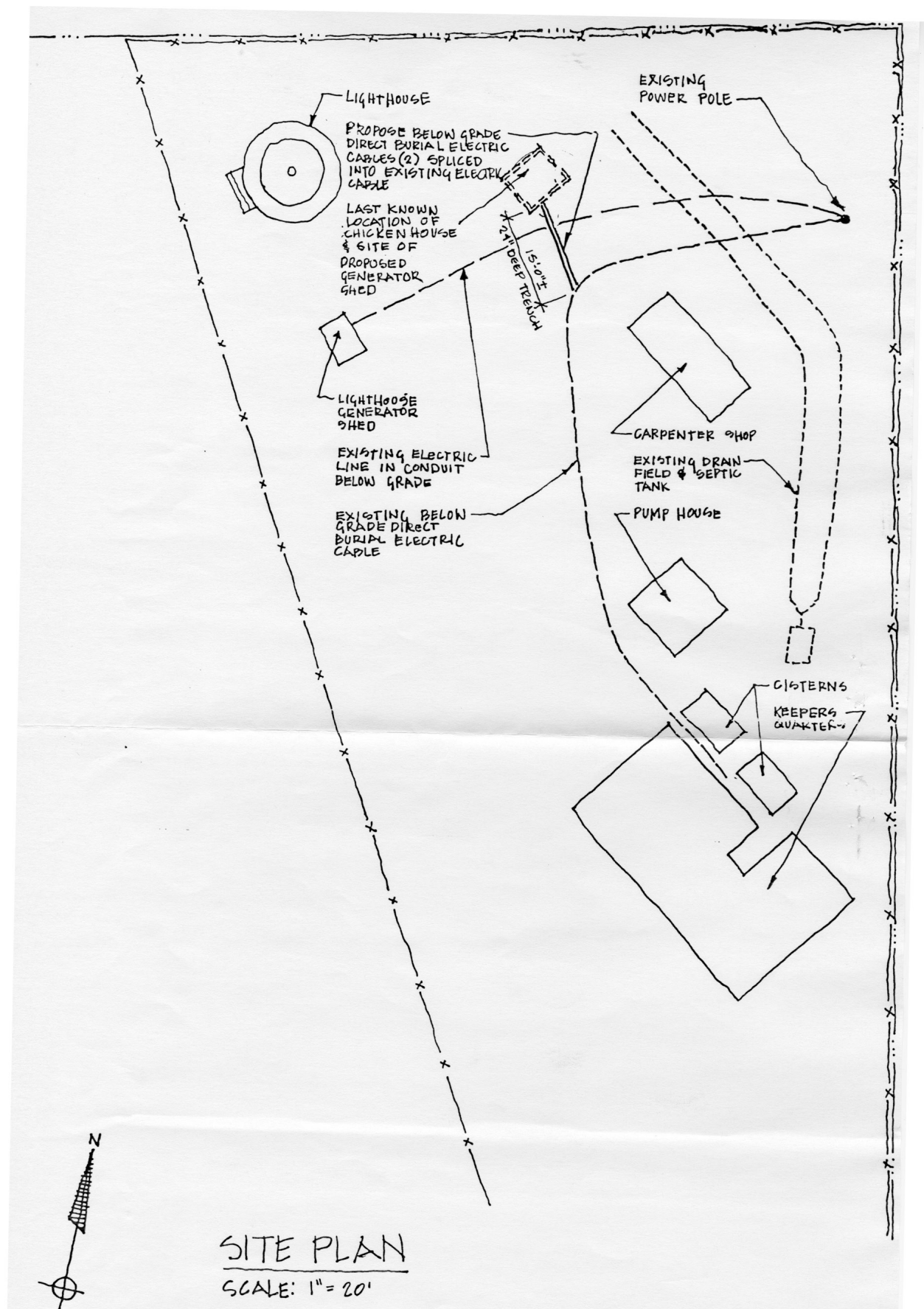
FIGURE B-22. Site plan showing new generator shed in location of chicken house, 1994. (NPS/CAHA Collection)
