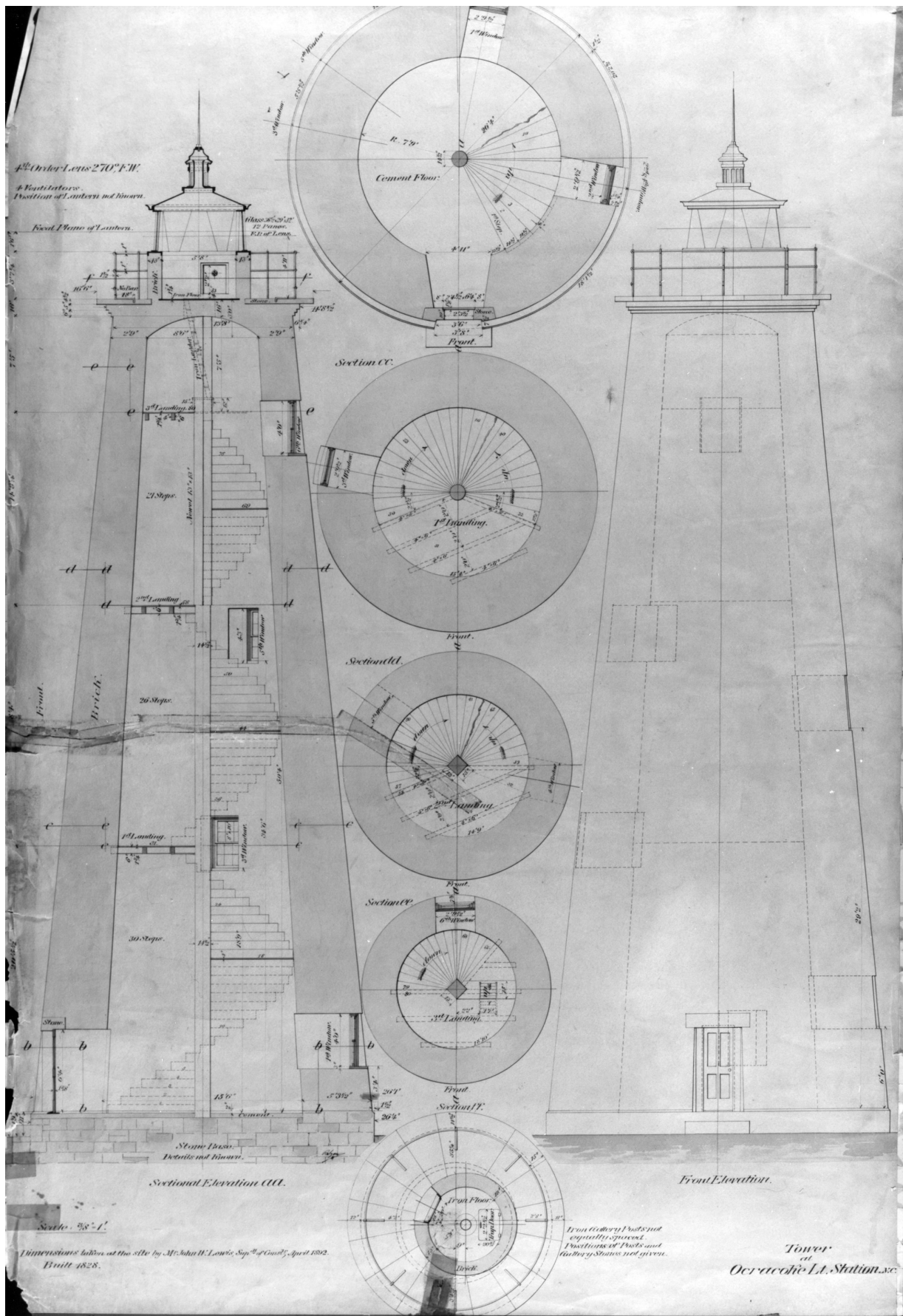
FIGURE B-5. Lighthouse plan, 1892. (NPS/CAHA Collection)
