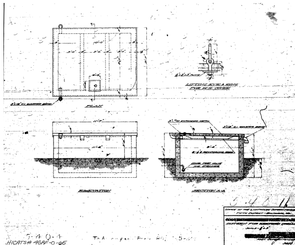
FIGURE 2-91. Plan of north cistern, n.d. (NPS/CAHA Collection)
