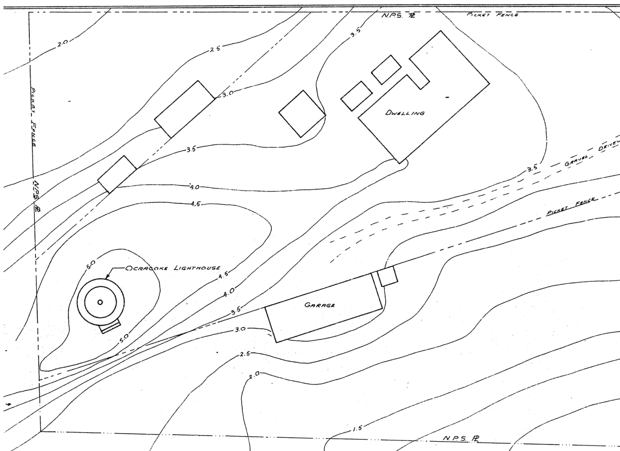
FIGURE 4-1. Topographic base map, 1961. (Denver Service Center etic 603/2172)
