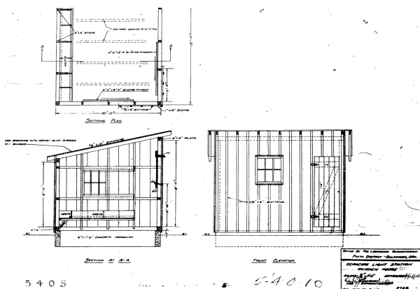
FIGURE 2-103. Plan of chicken house, before 1939. (NPS/CAHA Collection)
