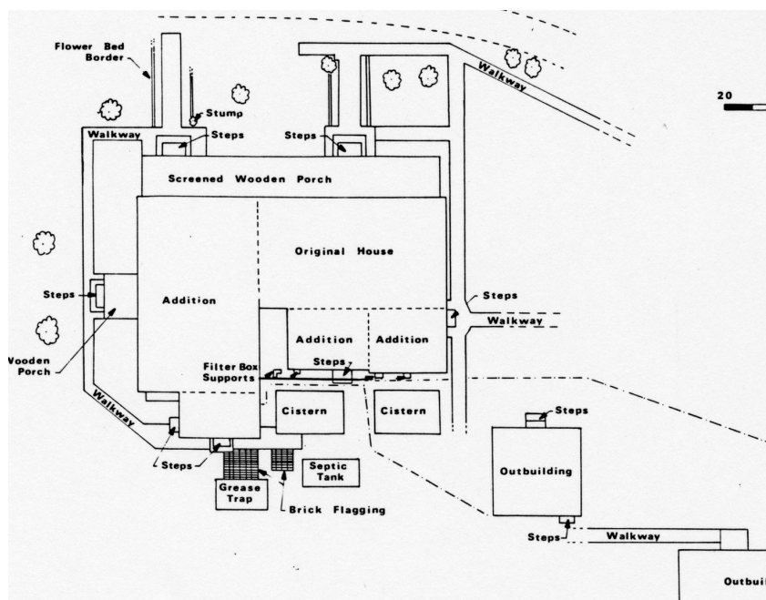
FIGURE 2-114. Layout of walkways from 1987 archeology site plan. (NPS/CAHA Collection)
