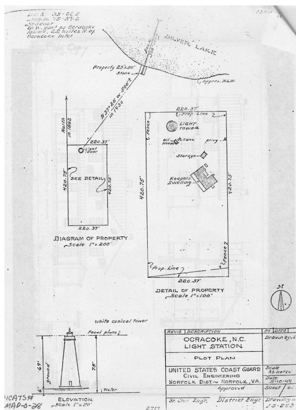
FIGURE 2-43. Plot plan of the light station showing a dock and boathouse on Silver Lake, 1944. (NPS/CAHA Collection)
