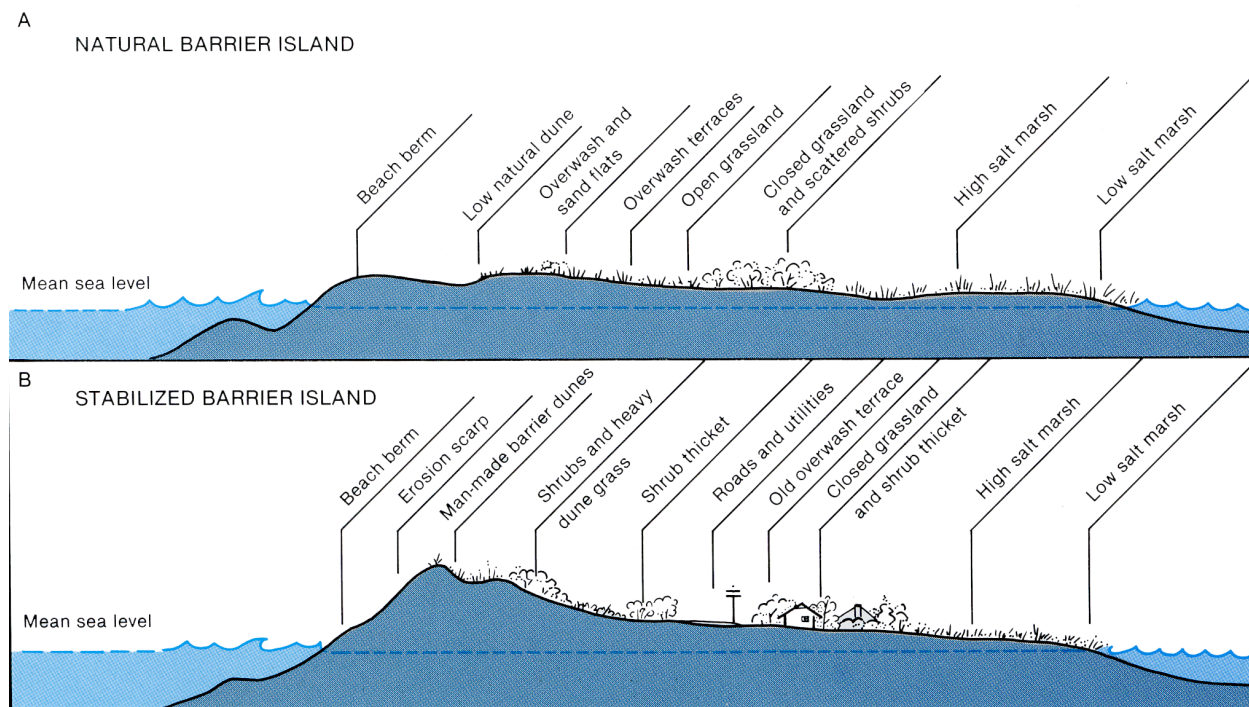
FIGURE 3-12. Natural vs. stabilized barrier island cross section. (Reprinted from Dolan and Lins, The Outer Banks of North Carolina )
