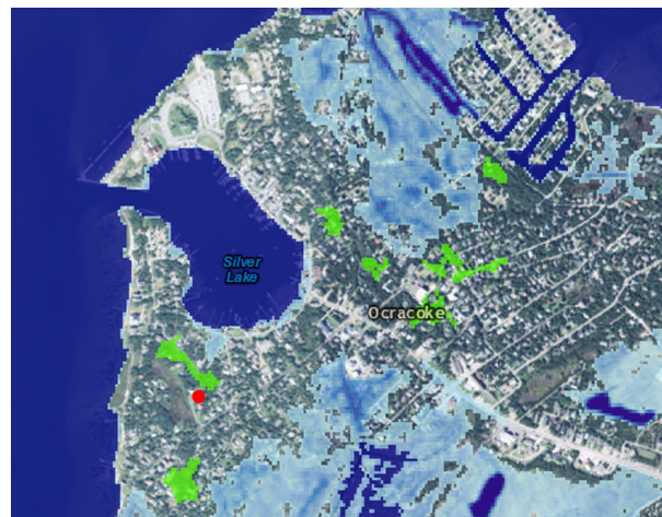
FIGURE 3-76. Inundation map for 1-ft rise in sea-level. Red dot denotes light station. (NOAA)
