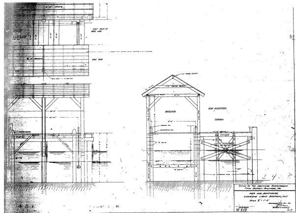
FIGURE 2-109. Plan of pier and boathouse, 1930. (NPS/CAHA Collection)
