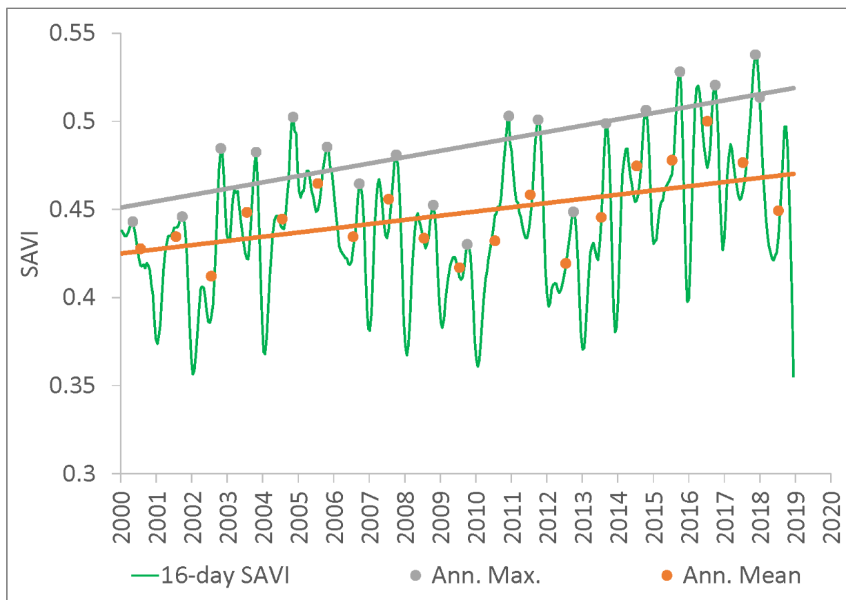
Figure 2. Measures of annual production from a time series of 16-day soil adjusted vegetation index (SAVI) derived from MODIS imagery. Linear trends against time for annual maximum and annual mean values are shown as straight lines.
