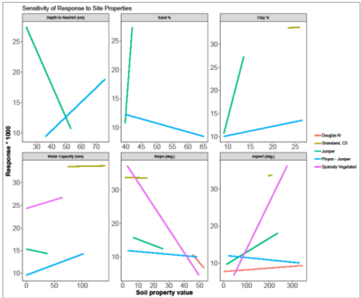
Figure 62. Variation in responses to precipitation as related to soil and site characteristics. Steeper slopes indicate greater sensitivity of responses to site properties. These site properties are important modifiers of climate because they control water retention and distribution in the soil profile and, in the case of site slope and aspect, because they affect the heat load on vegetation.
