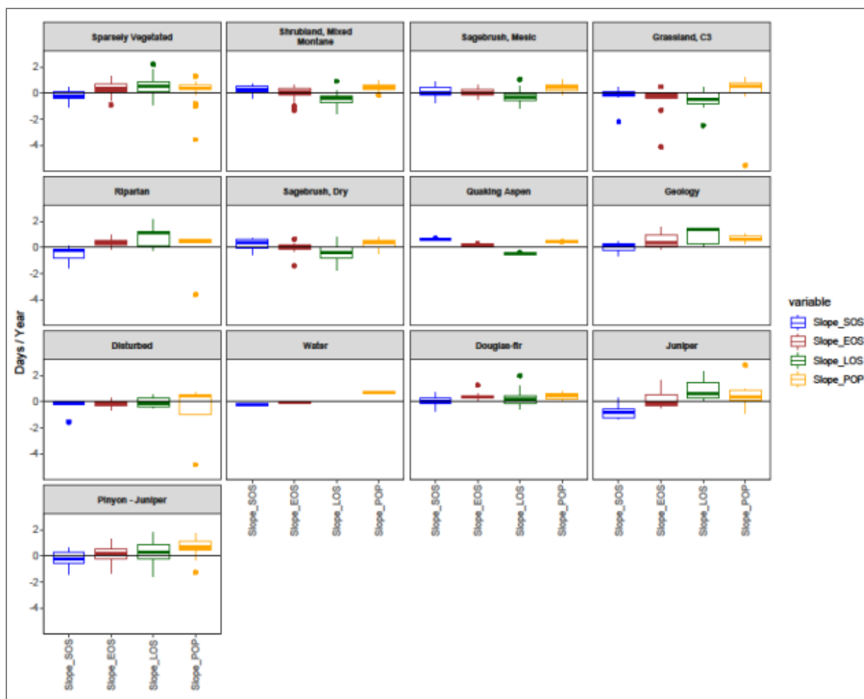
Figure 63. Direction and magnitude of change rate in land surface phenology metrics by alliance group, determined as \pm days per year for start of season date (Slope SOS), end of season date (Slope EOS), length of season (Slope LOS) and timing of peak SAVI (Slope POP). Slope refers to the slope of linear regression of phenology metric versus year for the period 2000–2019. NPS / DAVID THOMA
