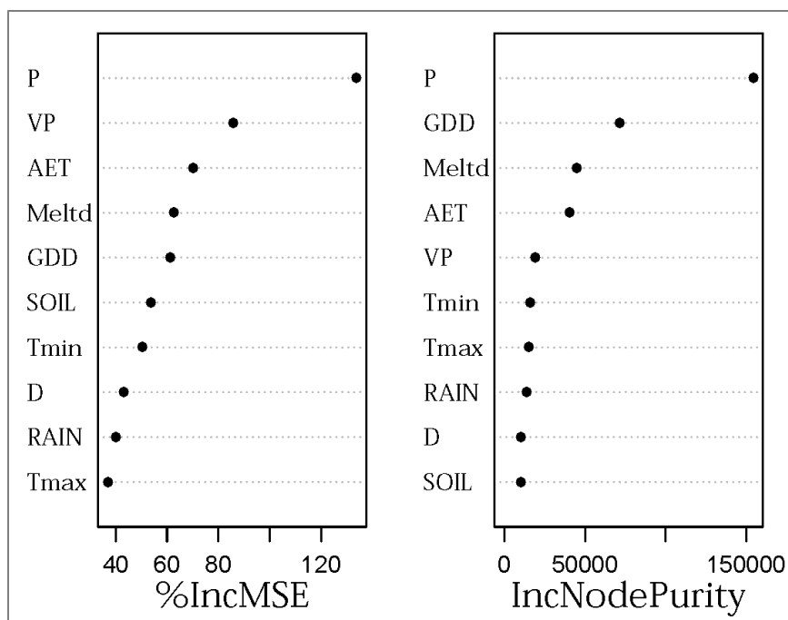
Figure 23. Variable importance in the random-forests model of climate drivers of the start of growing season. Percent increase in mean square error (%IncMSE) is a measure of model performance with each variable. Increase in node purity (IncNodePurity) is the difference in residual sum of squares in regression with or without each variable.
