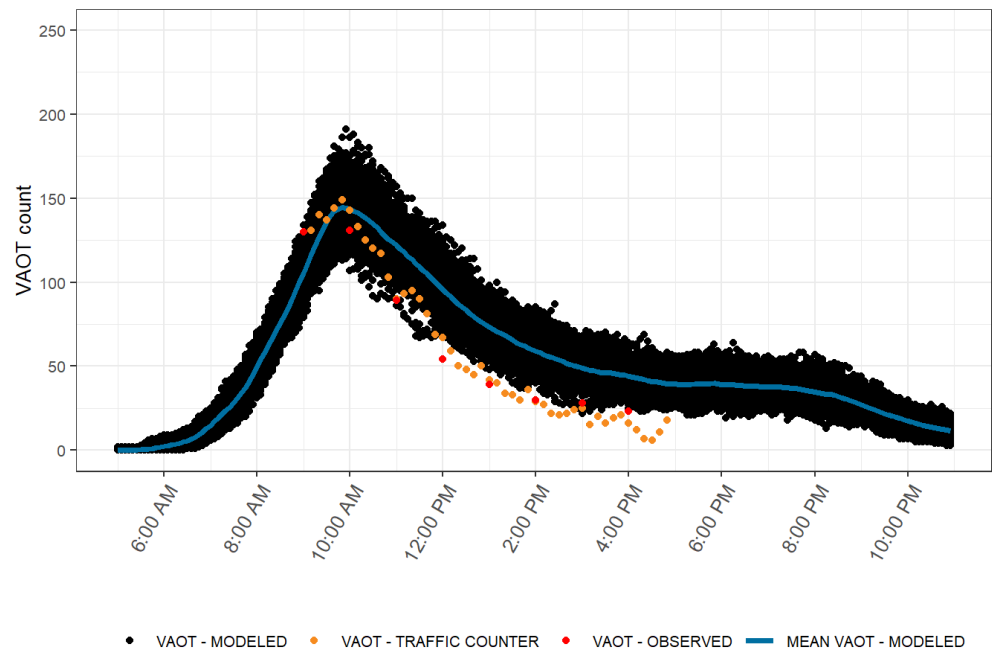
FIGURE 15. MODEL VALIDATION PLOT: VAOT AT DELICATE ARCH (SEPTEMBER 6, 2019)
