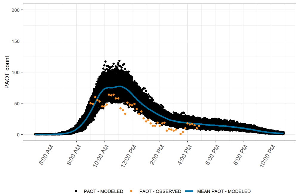
FIGURE 45. MODEL VALIDATION PLOT: PAOT IN THE DELICATE ARCH VIEWSCAPE (SEPTEMBER 9, 2019)
