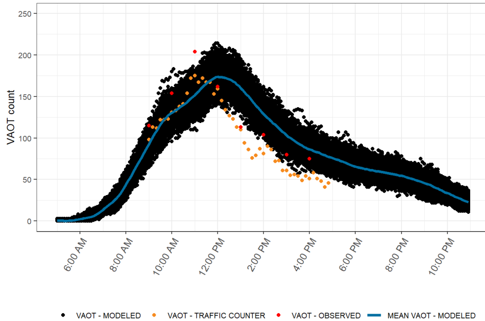
FIGURE 25. MODEL VALIDATION PLOT: VAOT AT DEVILS GARDEN (SEPTEMBER 7, 2019)
