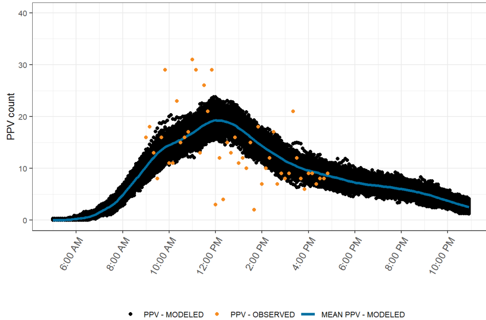
FIGURE 52. MODEL VALIDATION PLOT: PPV IN THE DEVILS GARDEN VIEWSCAPE (SEPTEMBER 7, 2019)
