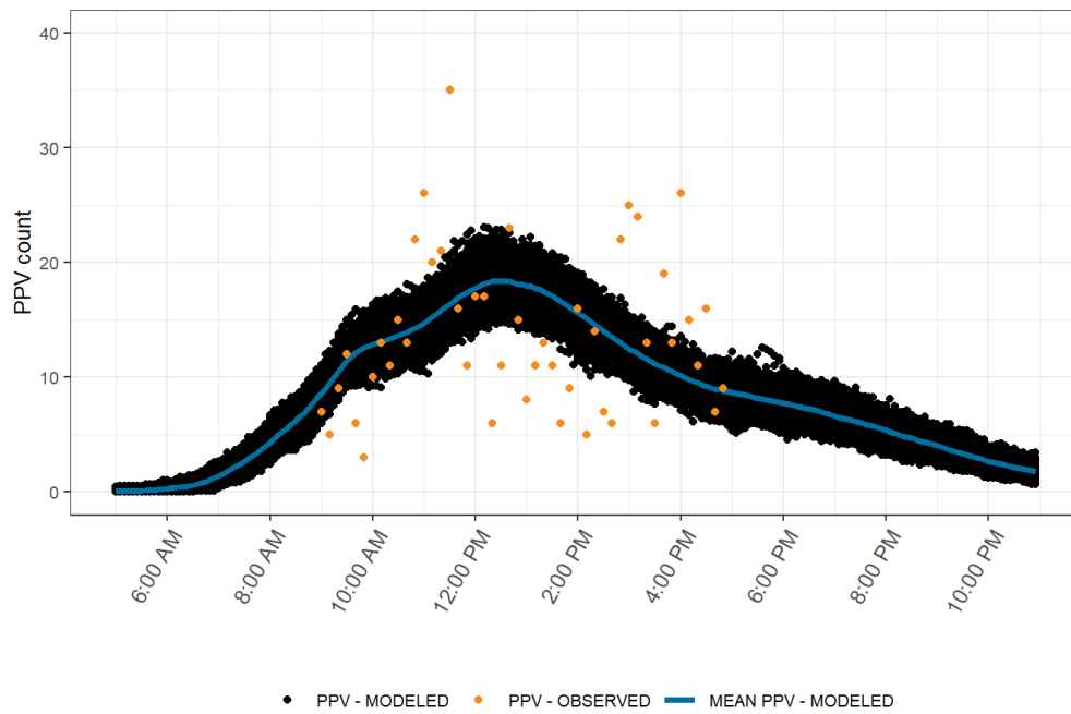
FIGURE 53. MODEL VALIDATION PLOT: PPV IN THE DEVILS GARDEN VIEWSCAPE (SEPTEMBER 8, 2019)
