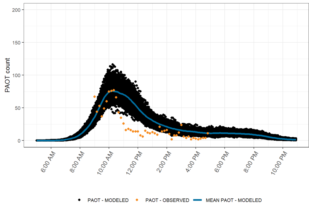
FIGURE 42. MODEL VALIDATION PLOT: PAOT IN THE DELICATE ARCH VIEWSCAPE (SEPTEMBER 6, 2019)
