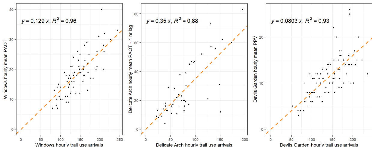
FIGURE 56. HOURLY SITE-LEVEL TRAIL USE ARRIVALS AND HOURLY SITE-LEVEL MEAN PAOT/PPV IN THE VIEWSCAPE, BY STUDY SITE
