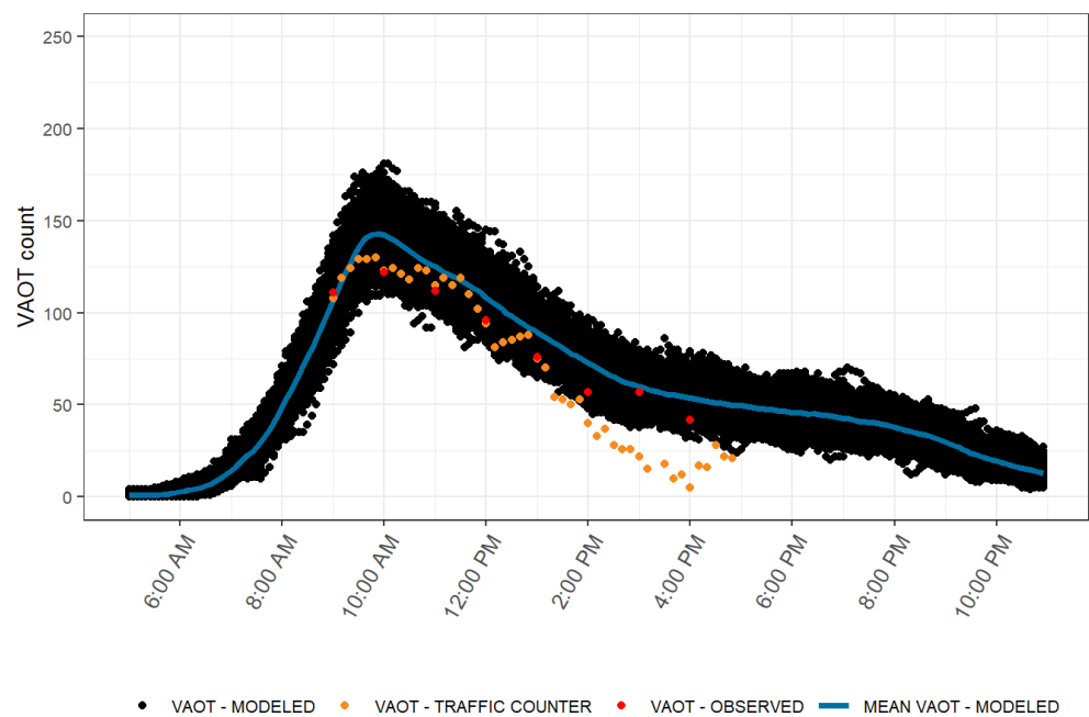
FIGURE 18. MODEL VALIDATION PLOT: VAOT AT DELICATE ARCH (SEPTEMBER 9, 2019)
