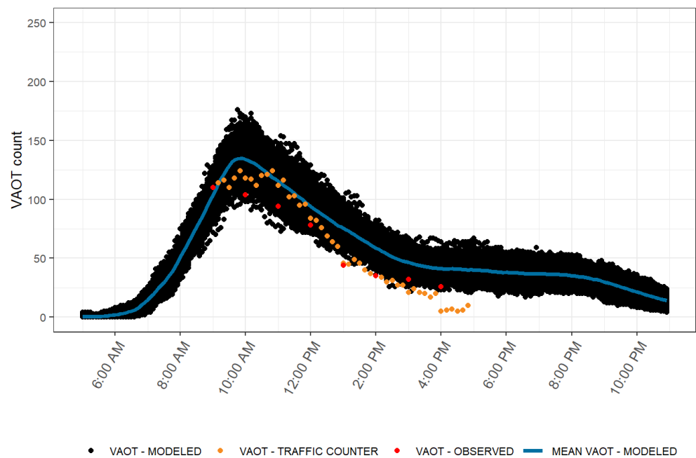
FIGURE 14. MODEL VALIDATION PLOT: VAOT AT DELICATE ARCH (SEPTEMBER 5, 2019)
