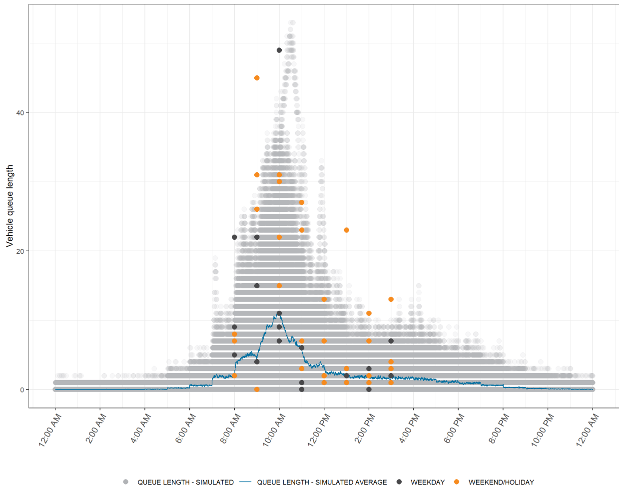
FIGURE 55. MODEL VALIDATION PLOT: ENTRANCE STATION VEHICLE QUEUE LENGTH (ALL STUDY SAMPLING DATES, EXCLUDING 09/01/2019 AND 09/10/2019 8 )
