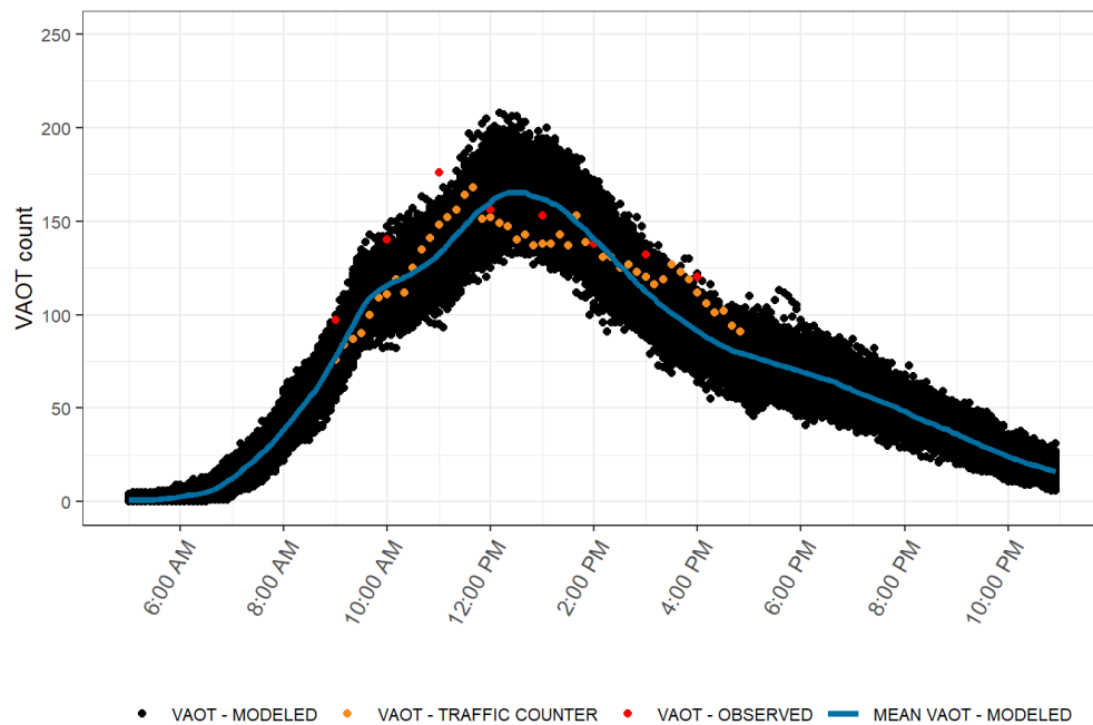
FIGURE 26. MODEL VALIDATION PLOT: VAOT AT DEVILS GARDEN (SEPTEMBER 8, 2019)
