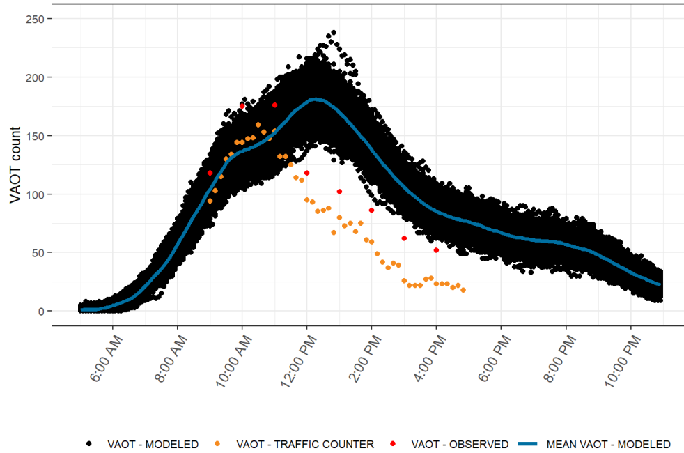
FIGURE 21. MODEL VALIDATION PLOT: VAOT AT DEVILS GARDEN (SEPTEMBER 2, 2019)
