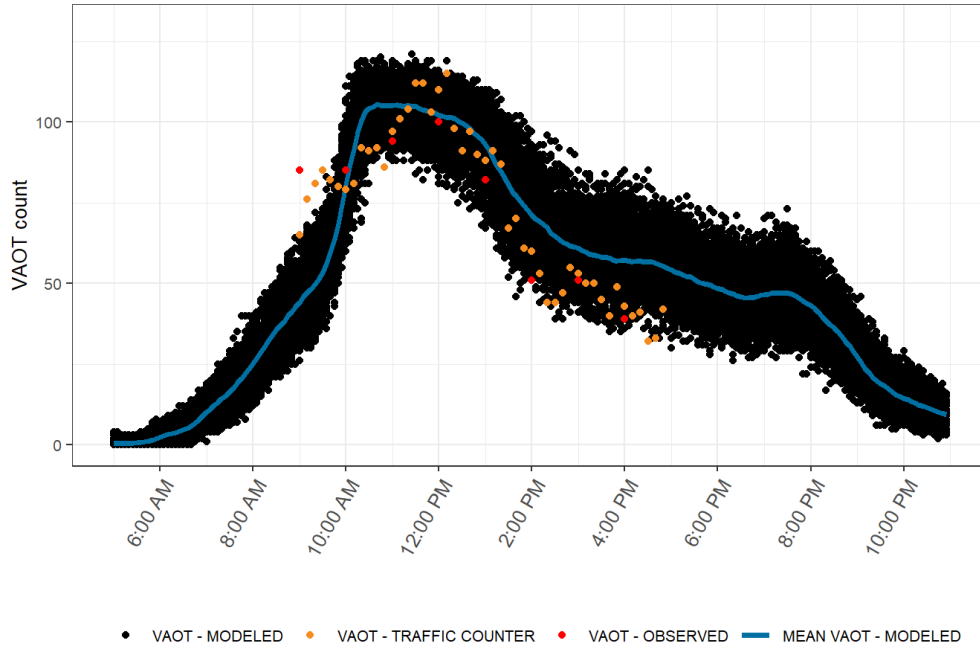
FIGURE 3. MODEL VALIDATION PLOT: VAOT AT THE WINDOWS (SEPTEMBER 2, 2019)
