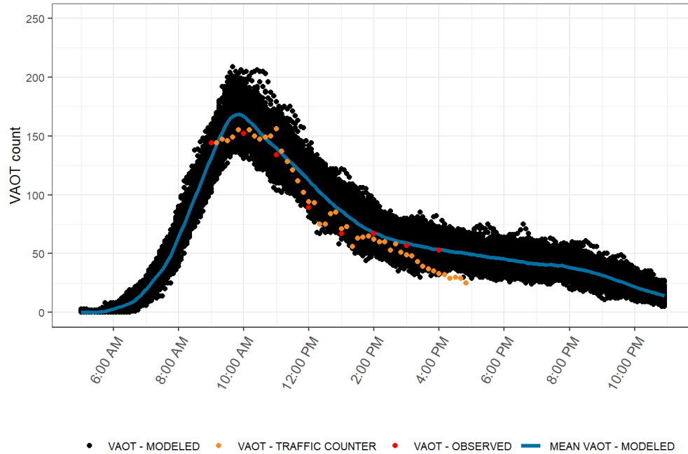
FIGURE 16. MODEL VALIDATION PLOT: VAOT AT DELICATE ARCH (SEPTEMBER 7, 2019)
