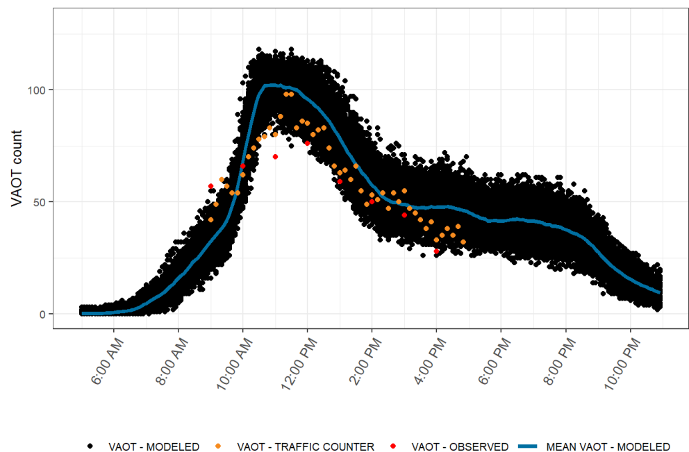
FIGURE 5. MODEL VALIDATION PLOT: VAOT AT THE WINDOWS (SEPTEMBER 5, 2019)
