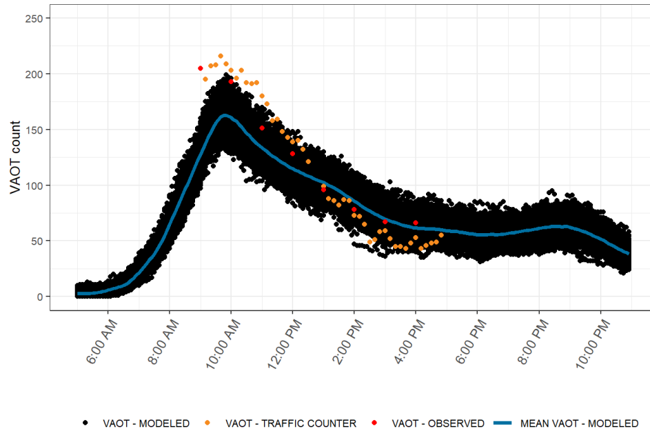
FIGURE 10. MODEL VALIDATION PLOT: VAOT AT DELICATE ARCH (AUGUST 31, 2019)
