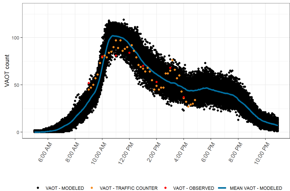
FIGURE 6. MODEL VALIDATION PLOT: VAOT AT THE WINDOWS (SEPTEMBER 6, 2019)
