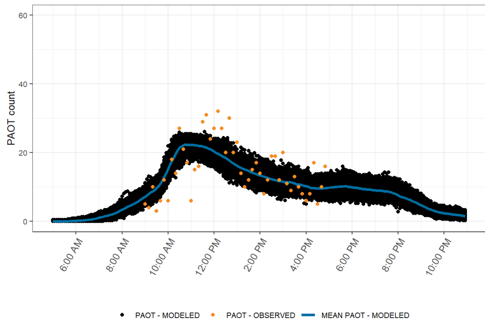
FIGURE 33. MODEL VALIDATION PLOT: PAOT IN THE WINDOWS VIEWSCAPE (SEPTEMBER 6, 2019)
