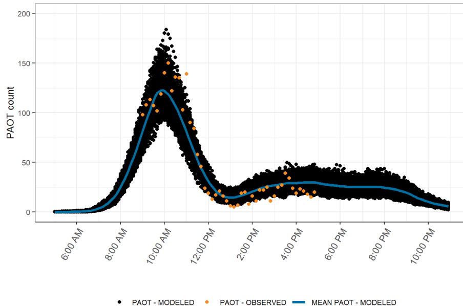
FIGURE 38. MODEL VALIDATION PLOT: PAOT IN THE DELICATE ARCH VIEWSCAPE (SEPTEMBER 1, 2019)
