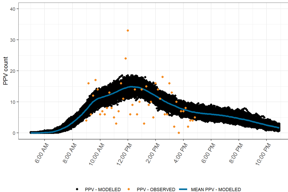
FIGURE 49. MODEL VALIDATION PLOT: PPV IN THE DEVILS GARDEN VIEWSCAPE (SEPTEMBER 4, 2019)
