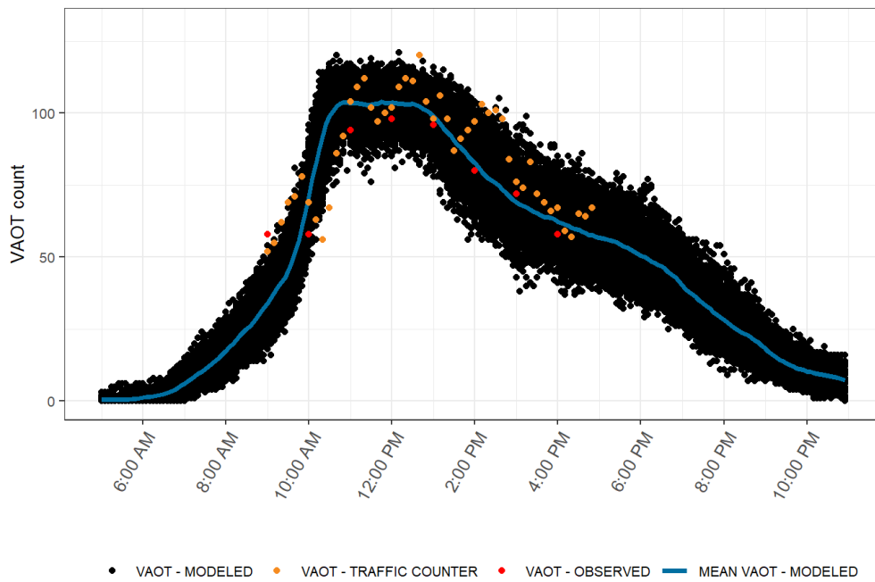
FIGURE 8. MODEL VALIDATION PLOT: VAOT AT THE WINDOWS (SEPTEMBER 8, 2019)
