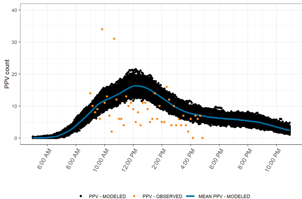
FIGURE 50. MODEL VALIDATION PLOT: PPV IN THE DEVILS GARDEN VIEWSCAPE (SEPTEMBER 5, 2019)
