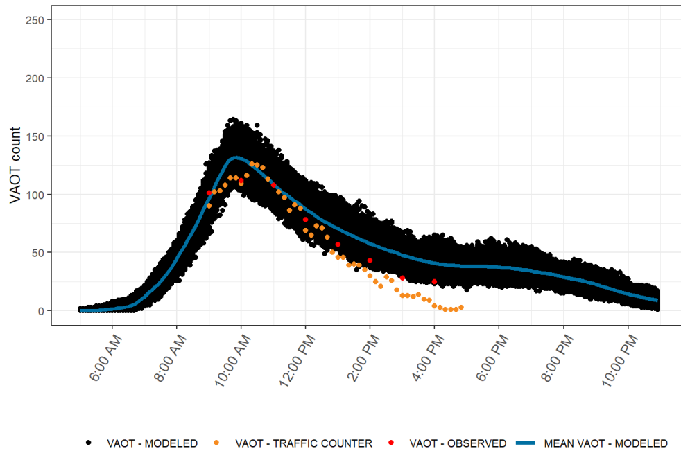
FIGURE 13. MODEL VALIDATION PLOT: VAOT AT DELICATE ARCH (SEPTEMBER 4, 2019)
