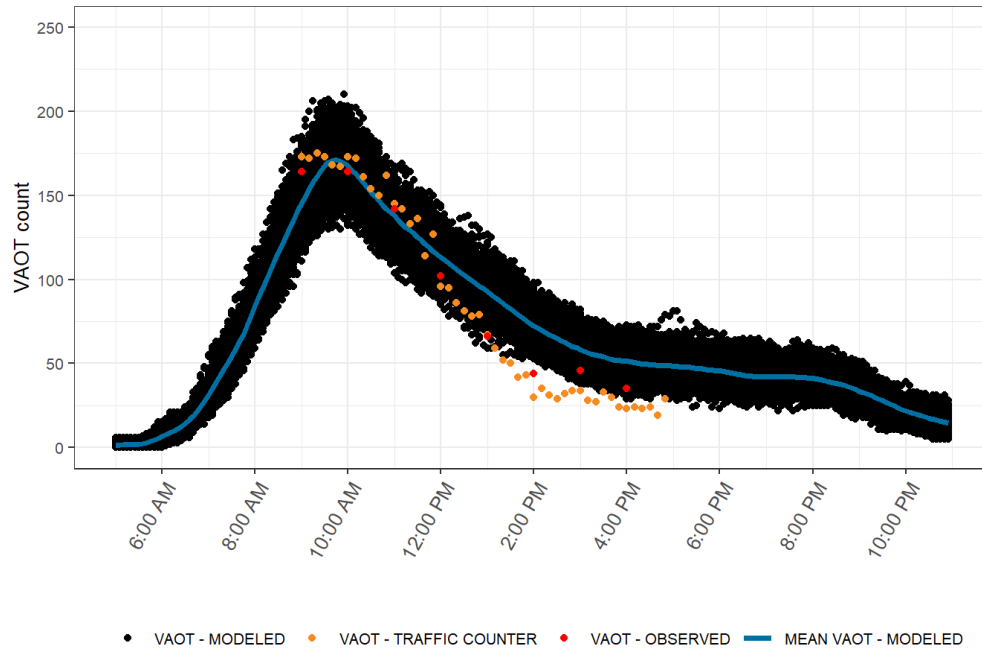
FIGURE 12. MODEL VALIDATION PLOT: VAOT AT DELICATE ARCH (SEPTEMBER 2, 2019)
