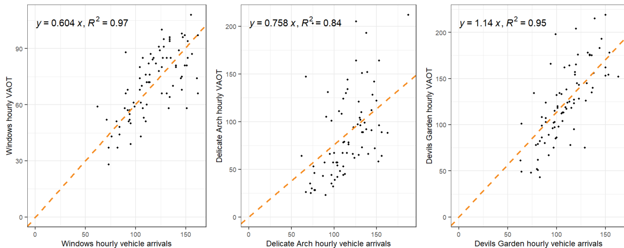
FIGURE 53. HOURLY SITE-LEVEL VEHICLE ARRIVALS AND HOURLY SITE-LEVEL PARKING ACCUMULATION (VAOT), BY STUDY SITE
