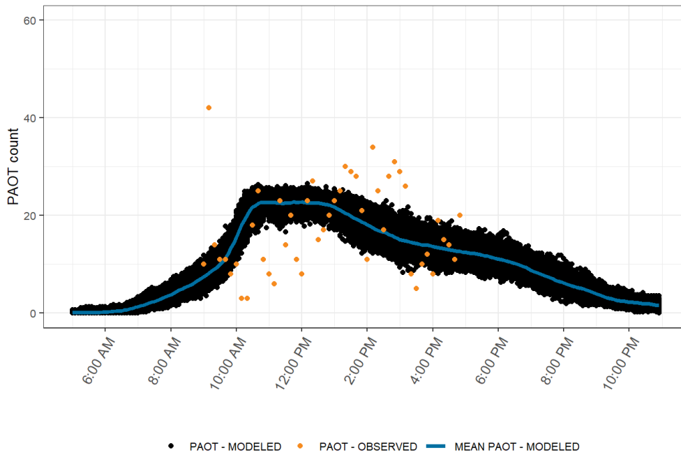
FIGURE 35. MODEL VALIDATION PLOT: PAOT IN THE WINDOWS VIEWSCAPE (SEPTEMBER 8, 2019)
