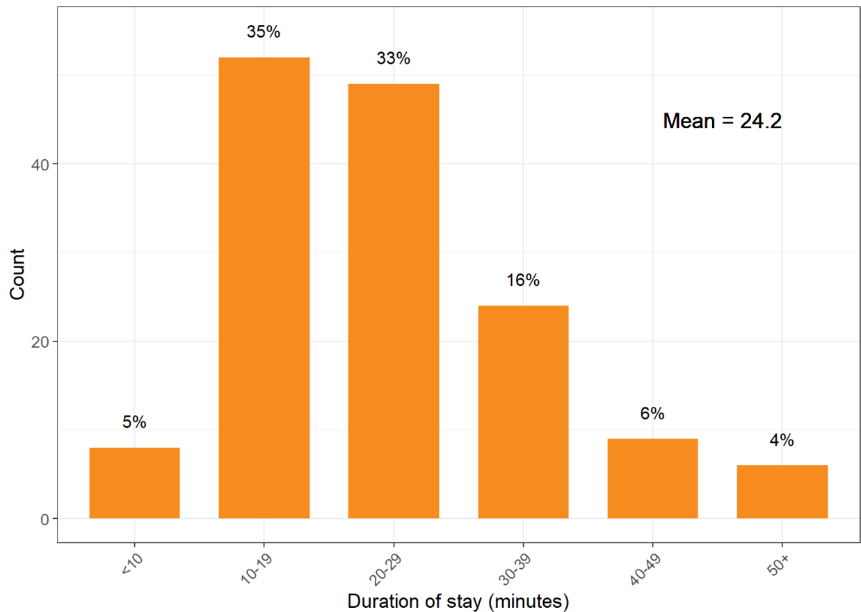
FIGURE 50. FREQUENCY DISTRIBUTION OF DELAY CARD-BASED DWELL TIMES: DELICATE ARCH VIEWSCAPE
