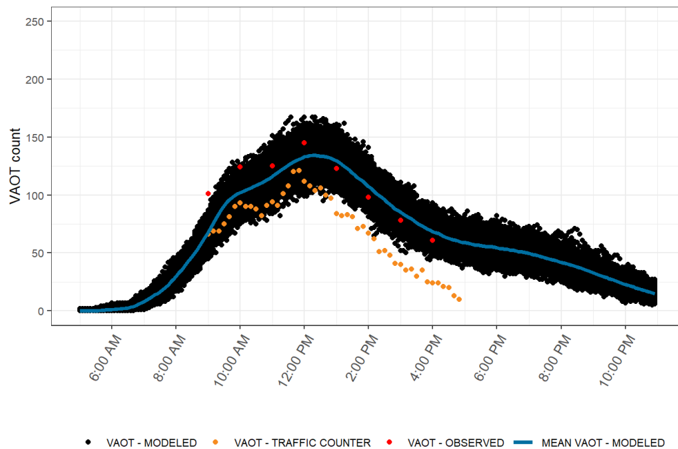
FIGURE 22. MODEL VALIDATION PLOT: VAOT AT DEVILS GARDEN (SEPTEMBER 4, 2019)
