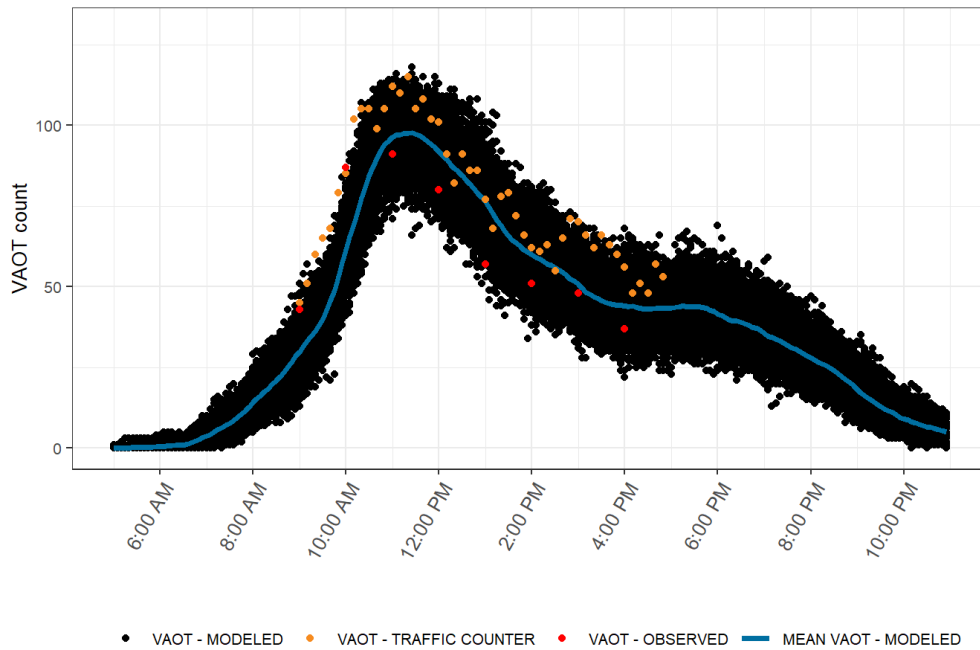
FIGURE 4. MODEL VALIDATION PLOT: VAOT AT THE WINDOWS (SEPTEMBER 4, 2019)
