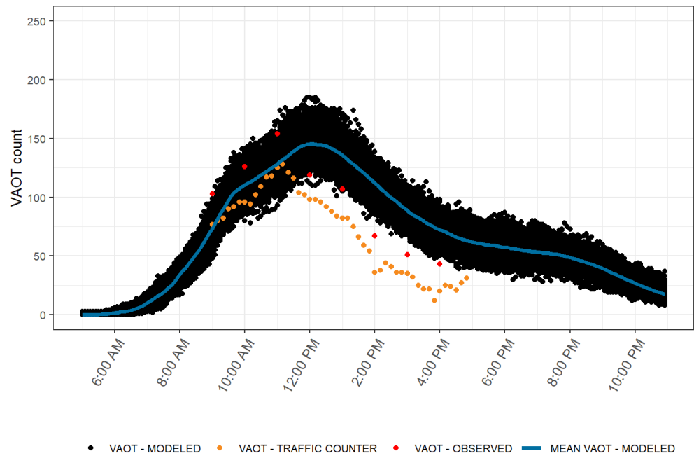
FIGURE 24. MODEL VALIDATION PLOT: VAOT AT DEVILS GARDEN (SEPTEMBER 6, 2019)
