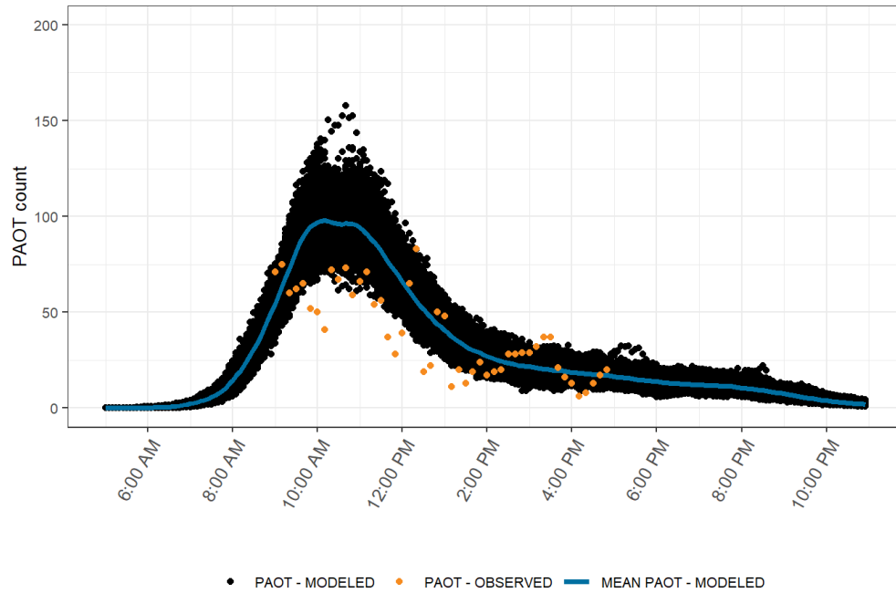
FIGURE 43. MODEL VALIDATION PLOT: PAOT IN THE DELICATE ARCH VIEWSCAPE (SEPTEMBER 7, 2019)
