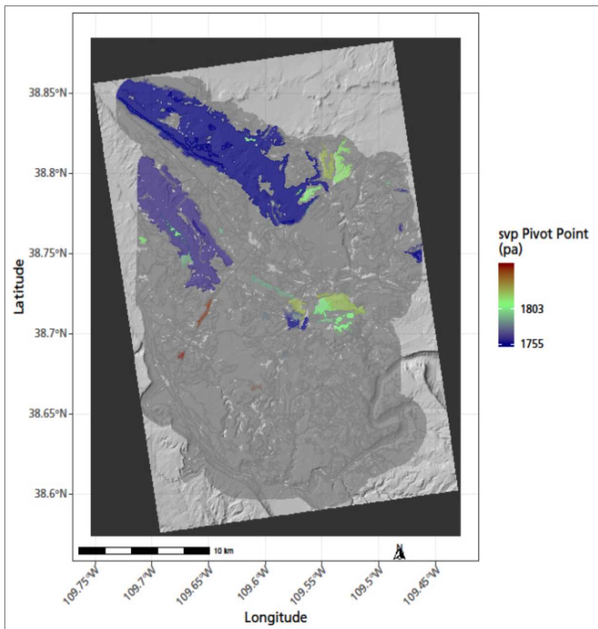
Figure 52. A map showing the locations of polygons where saturation vapor pressure was significantly related to interannual variation in production (p-value < 0.05). Climate data summarized by water year. NPS / DAVID THOMA
