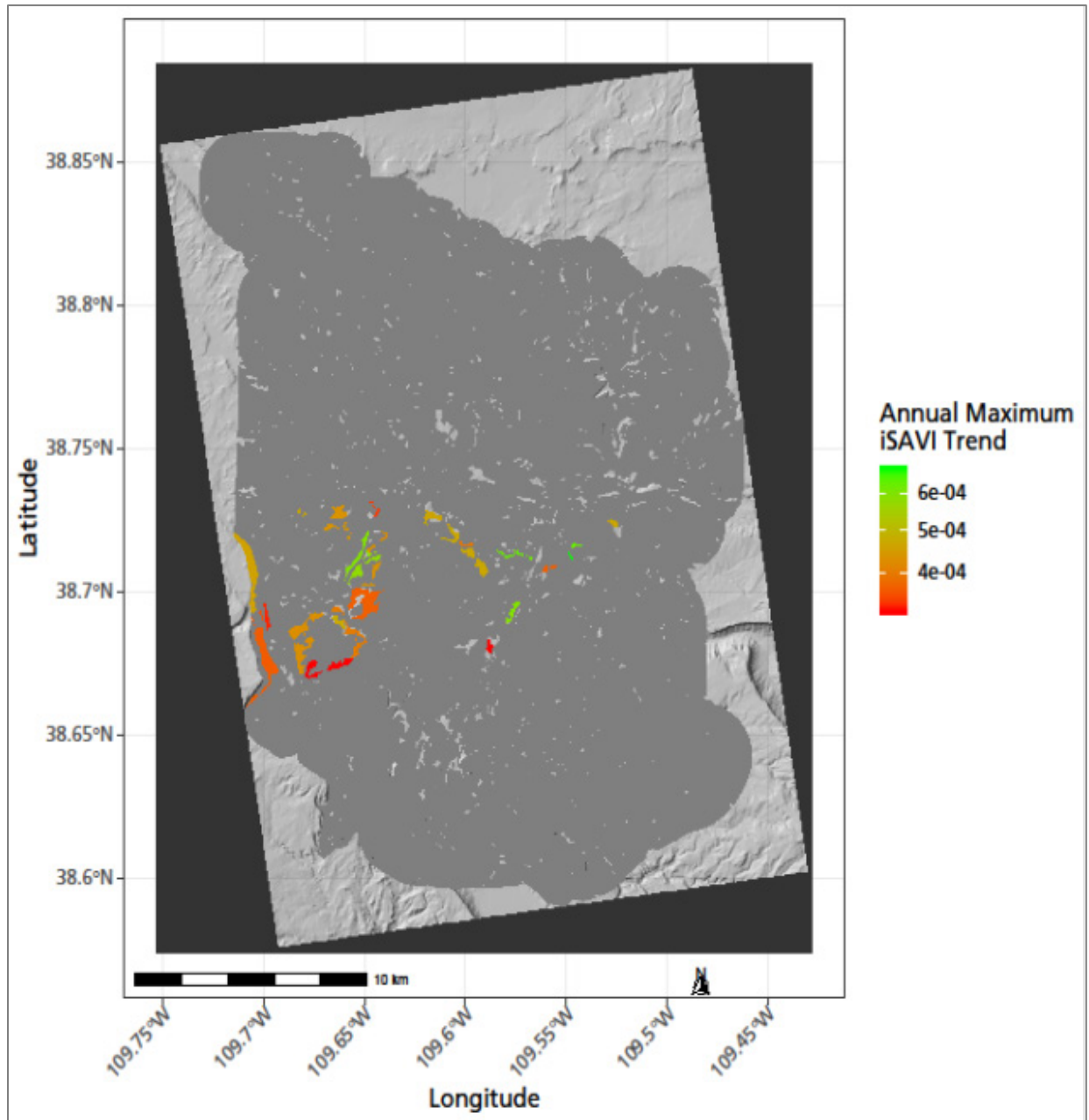
Figure 28. Spatial pattern of trends in maximum annual iSAVI. Trend is average change in iSAVI per year for the period 2000–2019.
