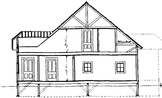
Section through A-B
