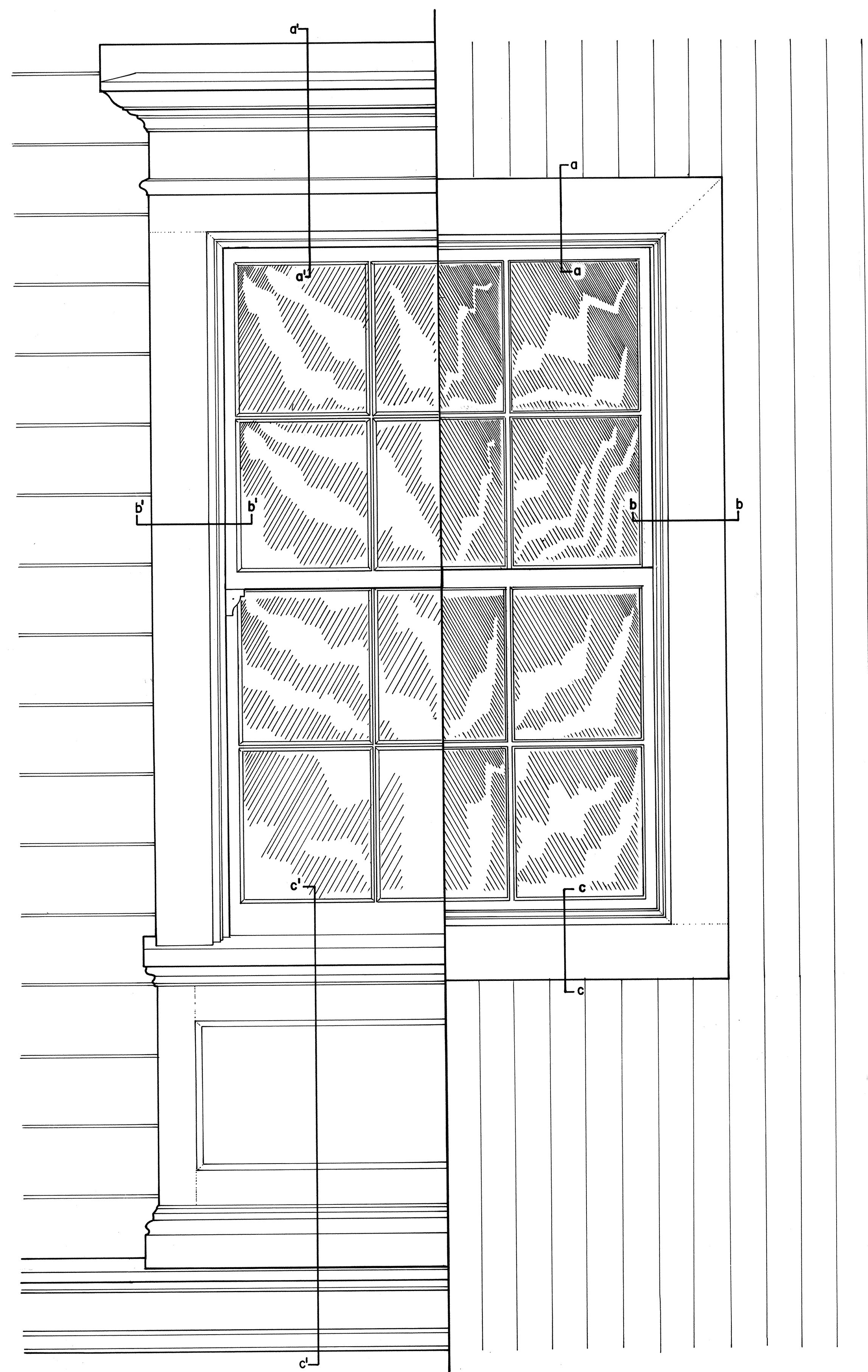
WINDOW ELEVATION
