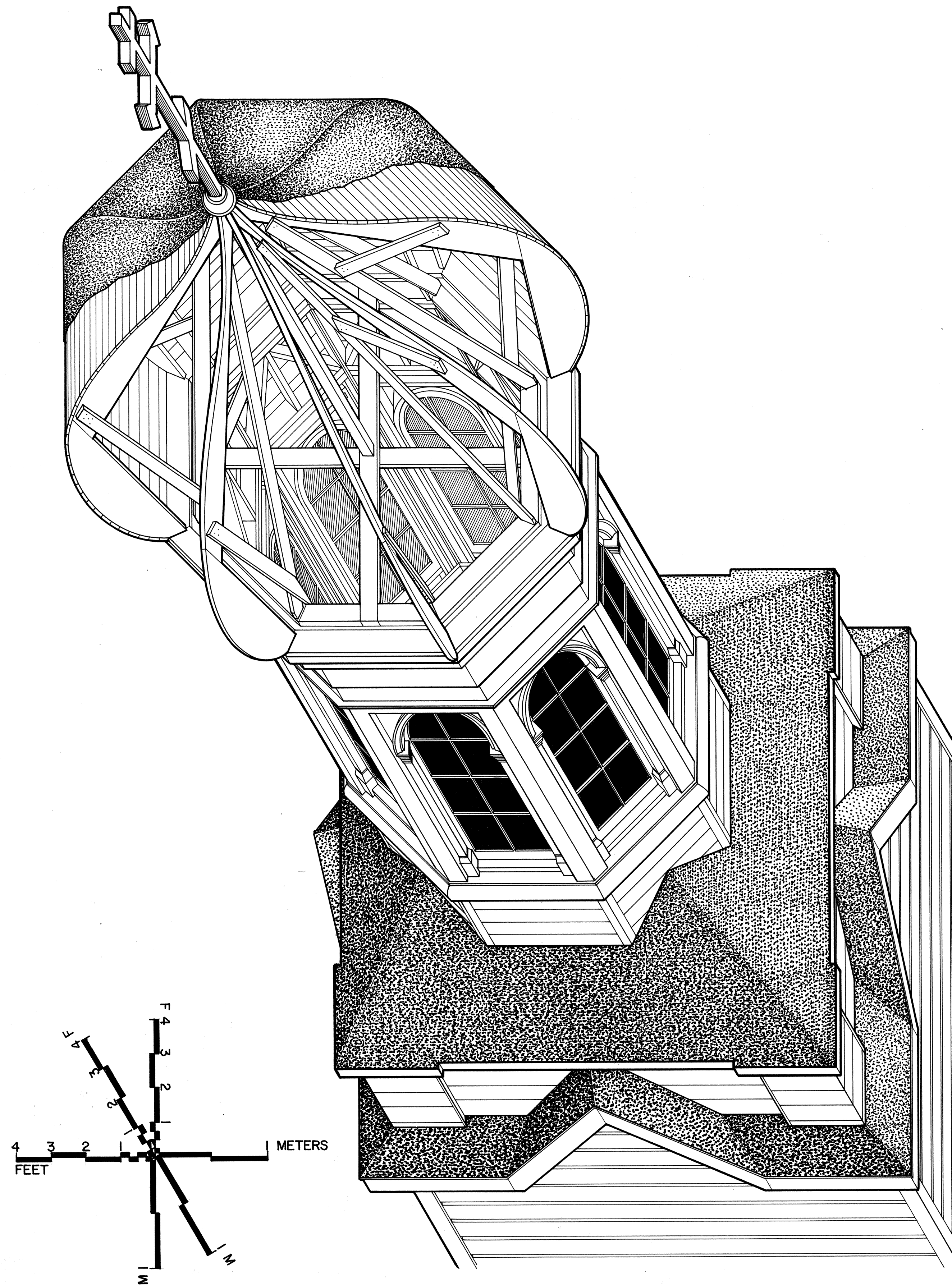
AXONOMETRIC OF BELL TOWER DOME
