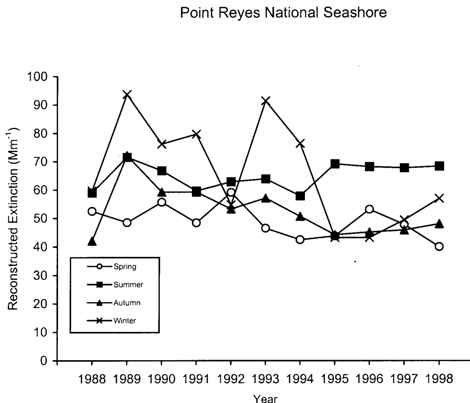
Figure VII-4. Seasonal average reconstructed extinction ( \text{Mm}^{-1} ), PORE, March 1988 through February 1999.
