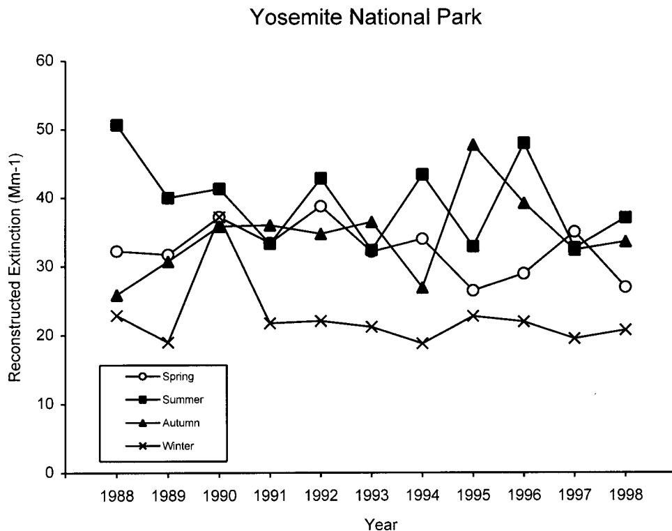
Figure X-4. Seasonal average reconstructed extinction ( \text{Mm}^{-1} ) at YOSE, March 1988 through February 1999.
