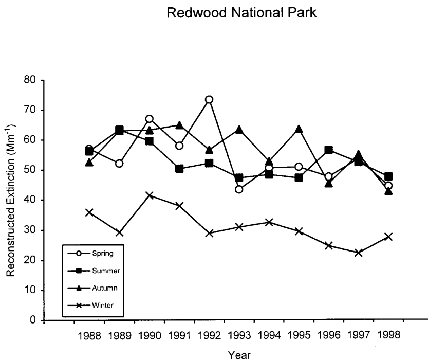
Figure VIII-4. Seasonal average reconstructed extinction ( Mm^{-1} ) in REDW, March 1988 through February 1999.
