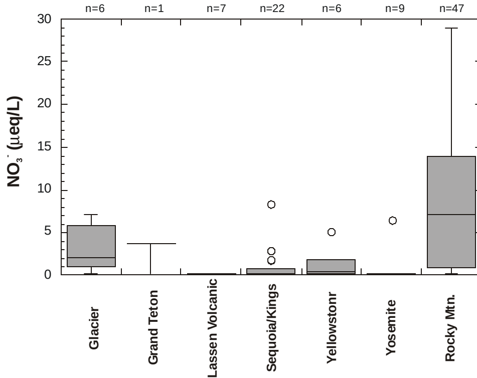
Figure IV-5. NO 3 - concentrations in high-elevation lakes sampled in 1999 in seven national parks by Clow et al. (2000).
