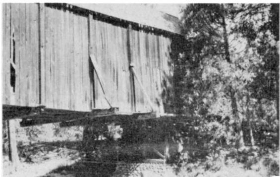
Bridge detail.
