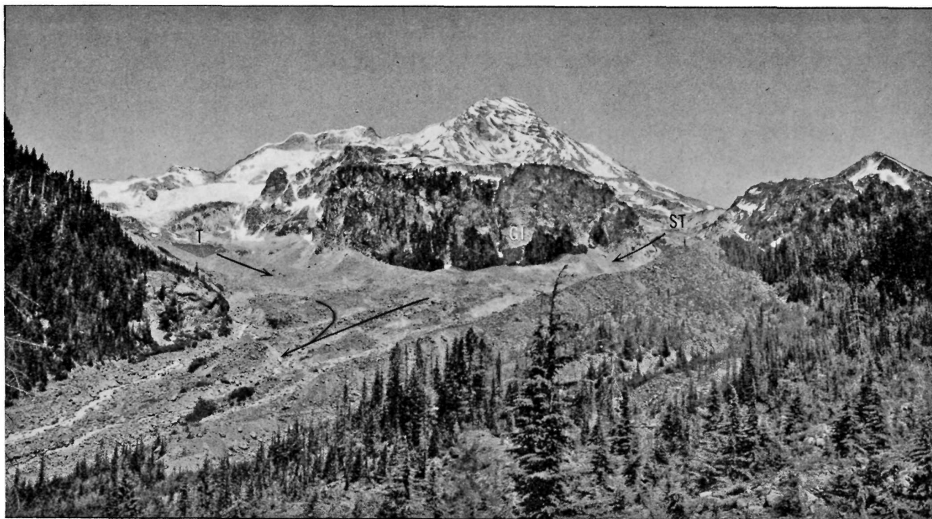
FIGURE 3.—South Tahoma Glacier (ST) and Tahoma Glacier (T) joined in 1910 below Glacier Island (GI) and extended out of view to the lower left. July 15, 1960.
