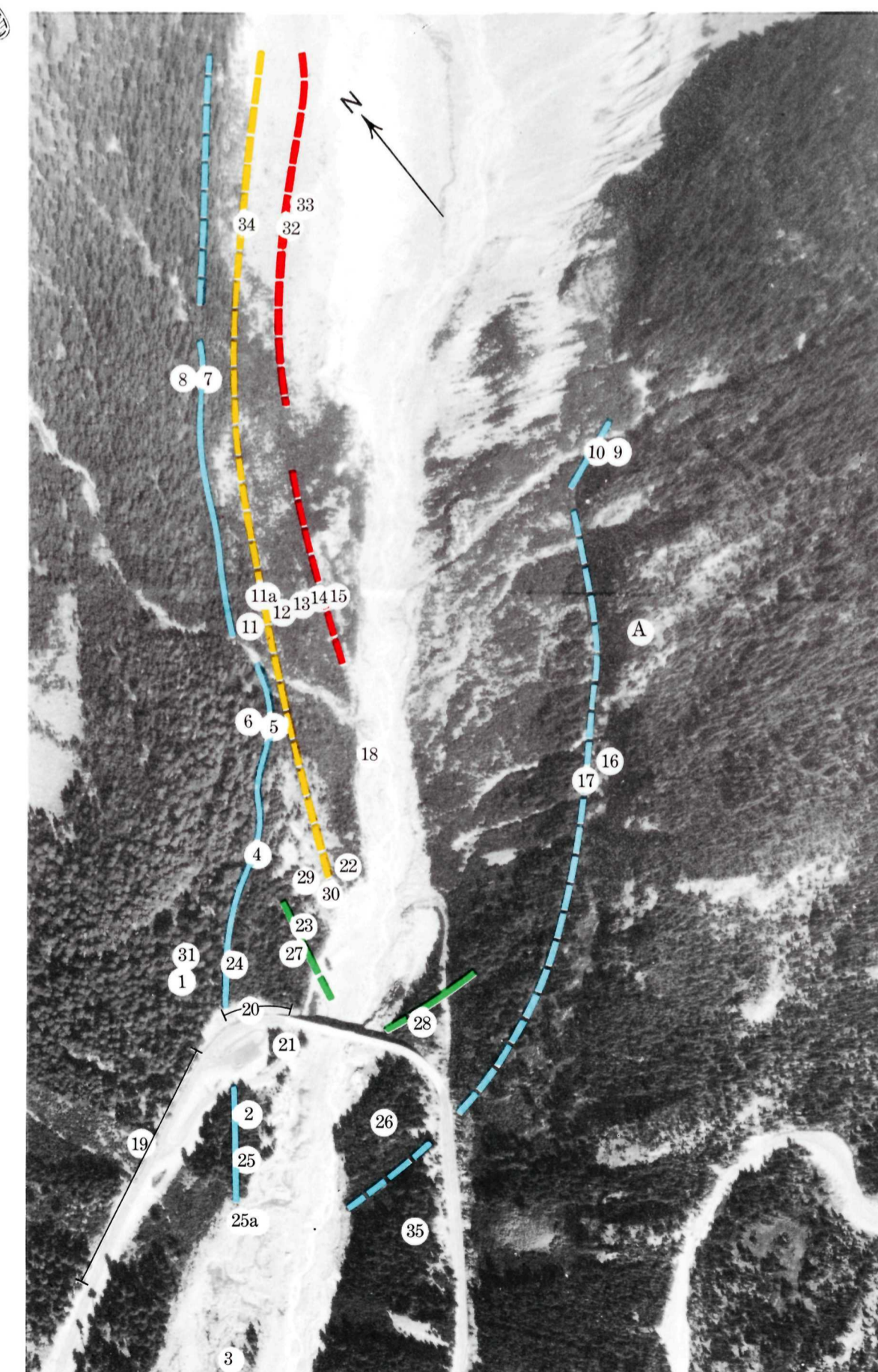
FIGURE 3.—Vertical photograph of Nisqually River valley in the vicinity of the bridge, taken on Aug. 16, 1967, and showing sample areas and moraines.
