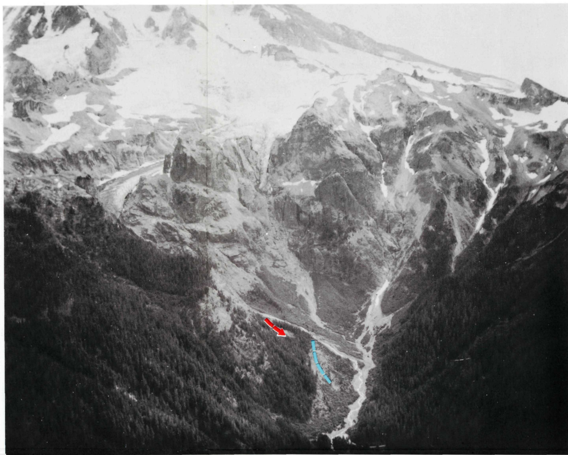
FIGURE 2.—Oblique view of Puyallup Glacier below Sunset Amphitheater which is the nearly vertical bedrock cliff below the crest of the mountain. Puyallup Glacier, which here curves around the prominent bedrock knob to the left of center and pokes through the narrow canyon in the center, plunged over the cliffs and flowed nearly to the parking area at the end of West Side Road in the early 19th century. Aug. 29, 1969.
