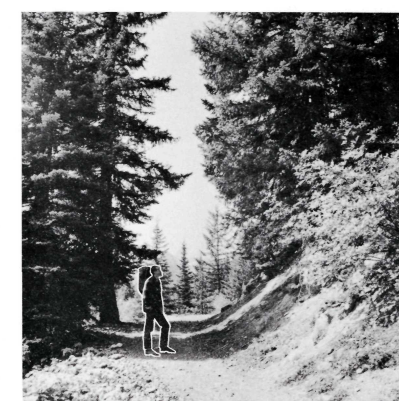
FIGURE 1.—Man in this photograph is standing on Glacier Basin Trail looking at the truncated end of the moraine from which Emmons Glacier started to recede about 1835, where it is cut by Inter Fork about one-half mile west of White River Campground. The prominent ridge form of the moraine can be seen at this site by climbing up the bank 15 feet to right in the trees. (See fig. 2, this plate). Sept. 8, 1967.
