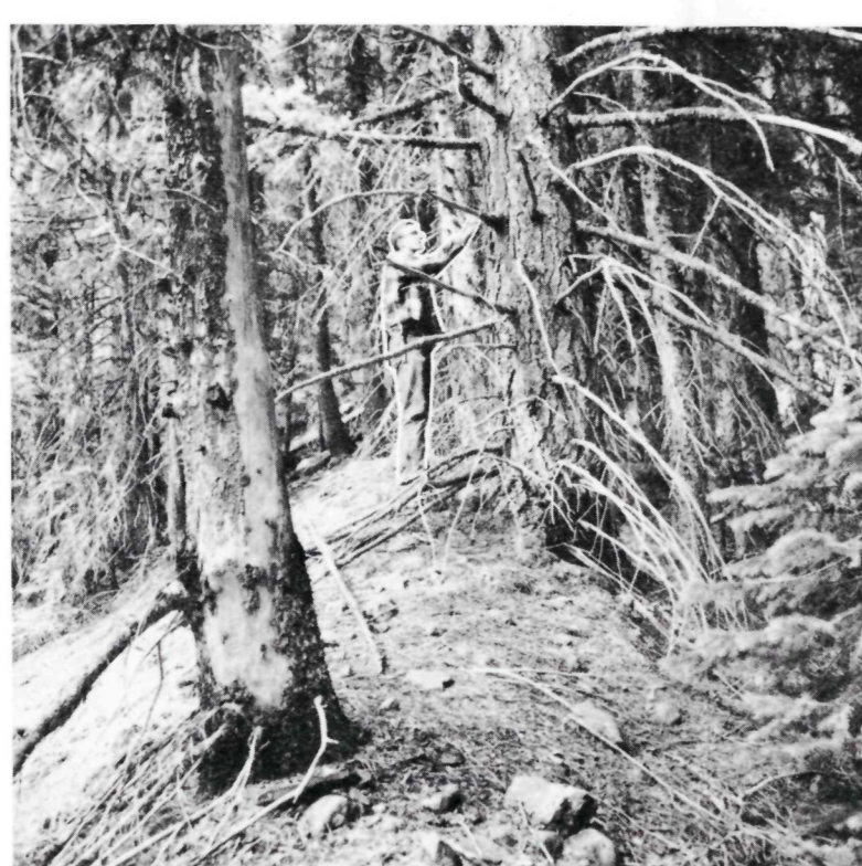
FIGURE 2.—The oldest tree on this moraine, just upslope and to the north of the one shown in figure 1, was 2 feet tall in A.D. 1842 (Area 31). Sept. 8, 1967.
