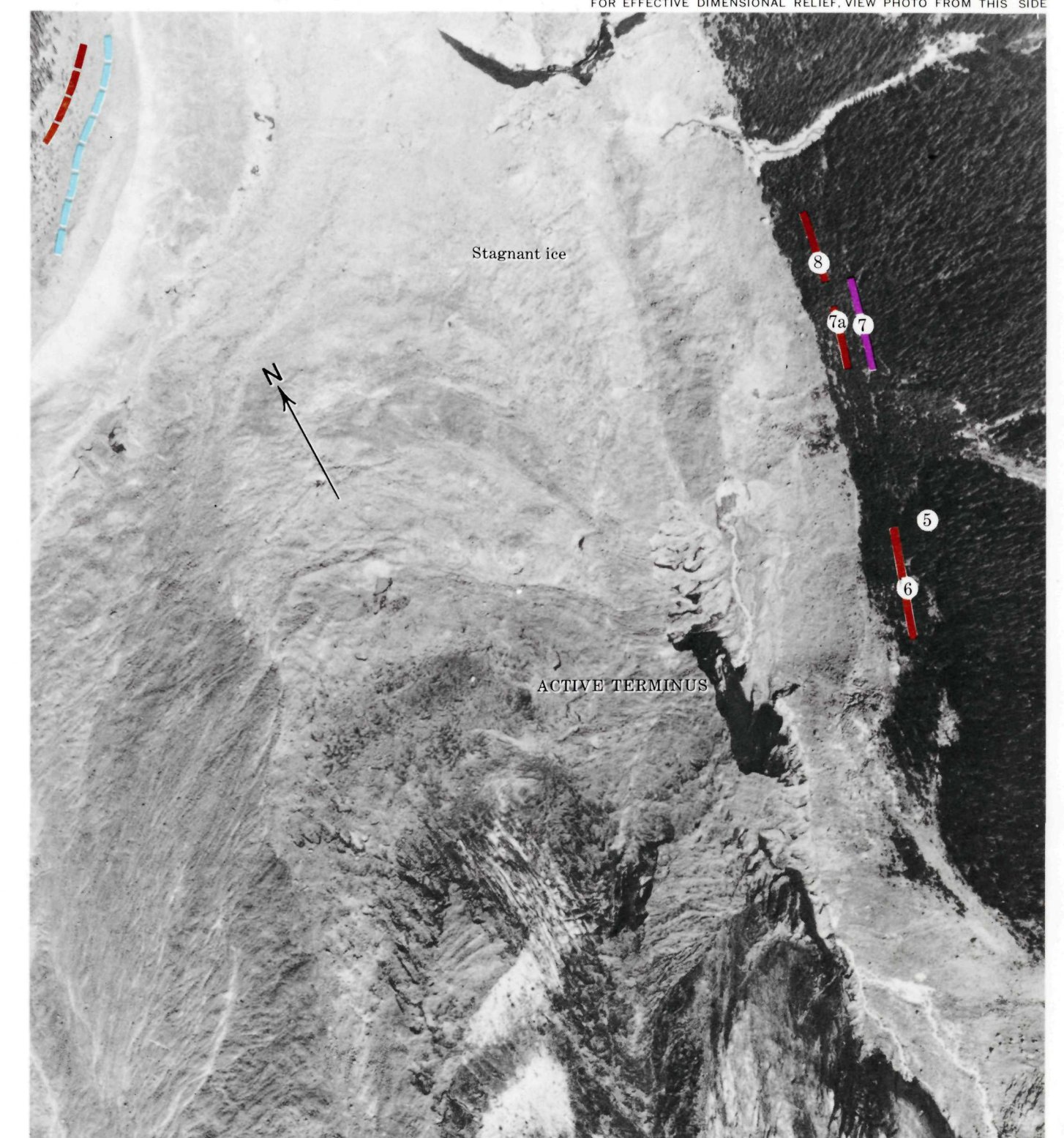
FIGURE 4.—Vertical photograph of the active terminus of Winthrop Glacier and of the upvalley end of the stagnant ice. Area photographed is just south of the area shown in figure 5 and shows sample areas and locations of the A.D. 1650 and 1765 moraines. Aug. 16, 1967.
