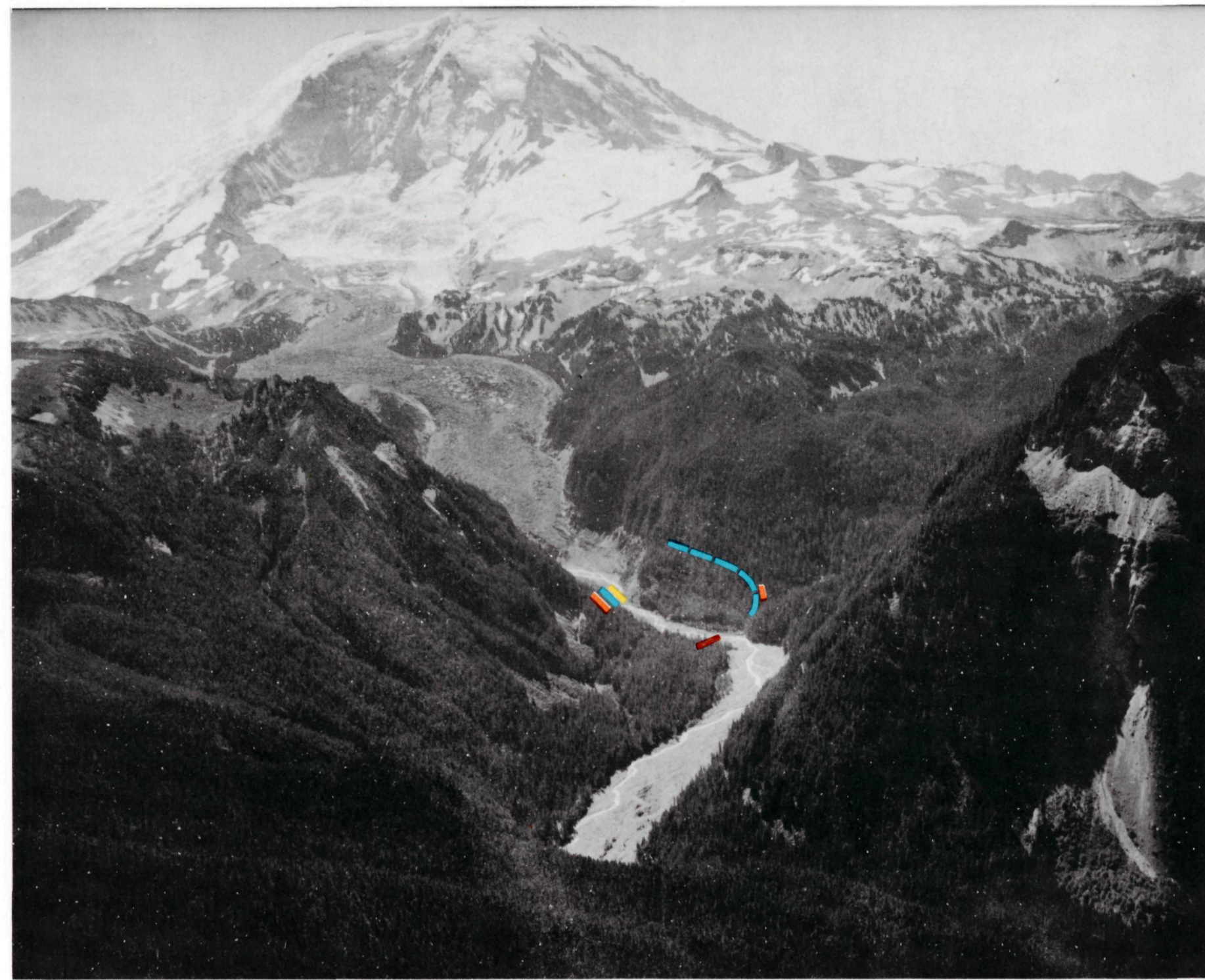
FIGURE 1.—Oblique view of the advancing terminus of Carbon Glacier shows its closeness to the maximum advance in 10,000 years marked by the brown and orange lines. The terminus started to recede from the area marked by the brown line about A.D. 1760. Earlier, near the end of the 15th century, the glacier was broader near the terminus and left moraines marked by orange lines. Cataract Creek, not clearly visible in the photograph, occupies the valley in the foreground flowing from the right to Carbon River in left center. View is southeastward. Aug. 29, 1969.
