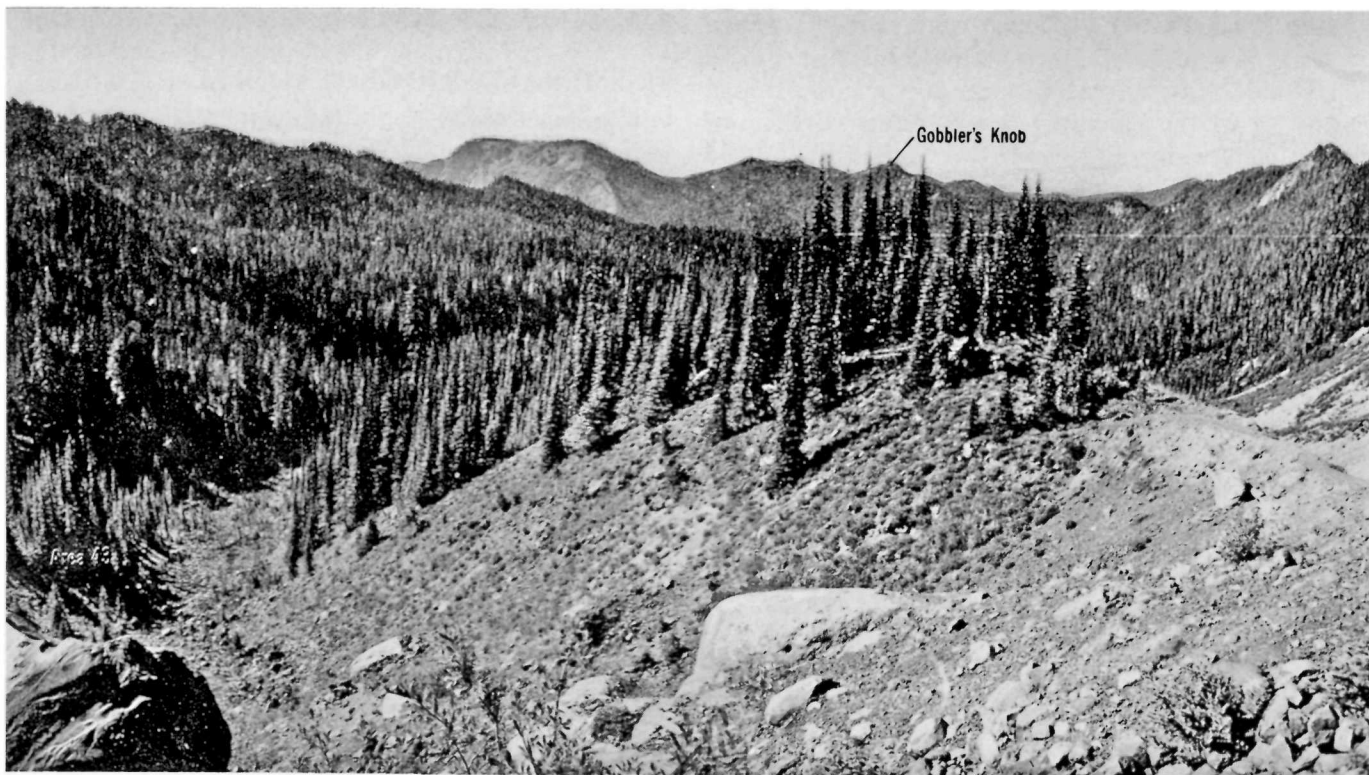
FIGURE 8.—Wonderland Trail follows the narrow ridge extending from the trees in the right foreground to margin of photograph at the right. Tahoma Glacier extended down the steeply sloping valley on the left and formed a moraine which is out of sight. On the left the open valley supporting small scattered trees is floored with gravel deposited before 1865. This gravel was eroded by melt water between 1865 and 1910.
