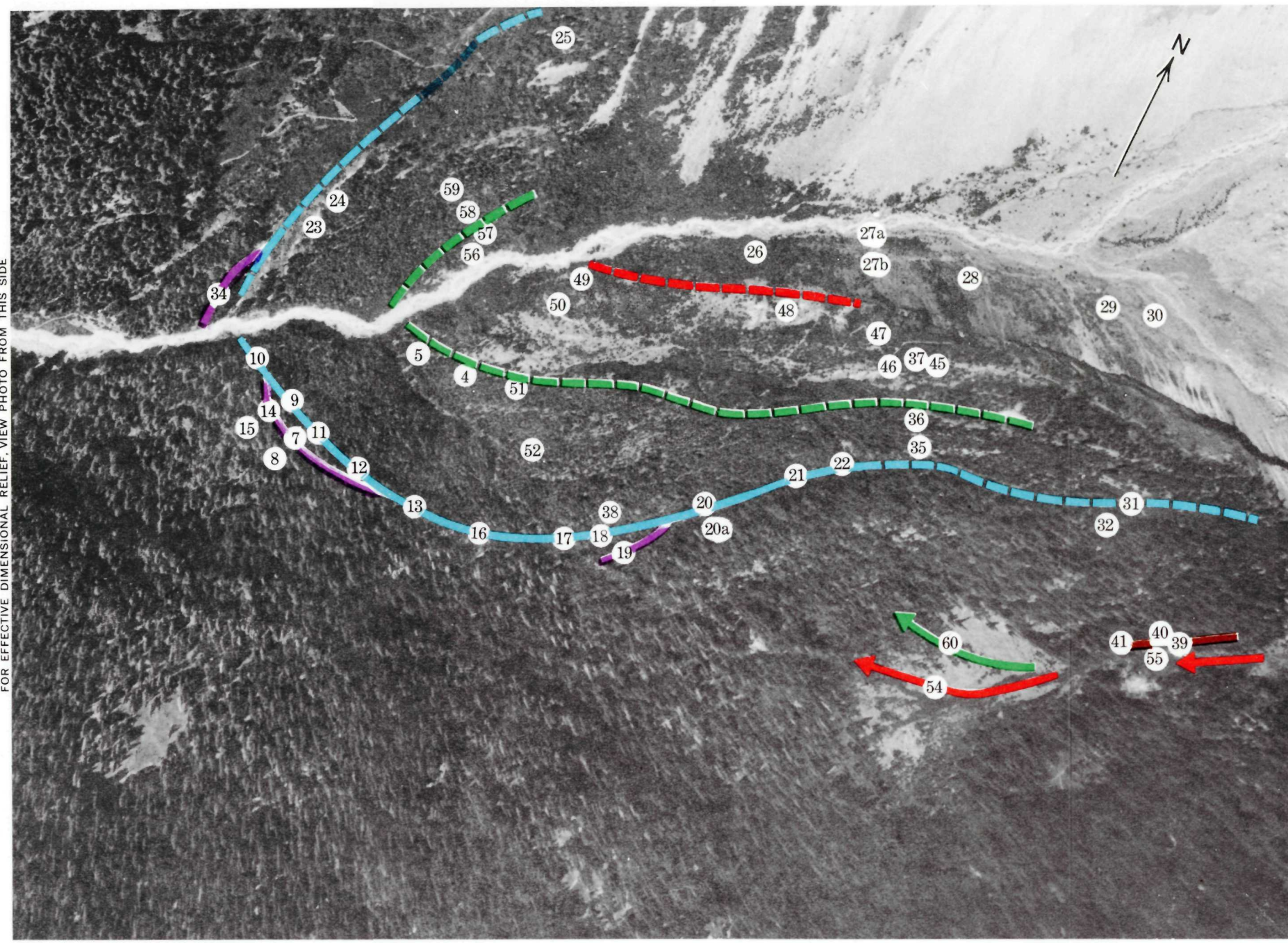
FIGURE 3.—Vertical photograph of South Puyallup River showing location of sample areas, Tahoma Glacier moraines, and melt-water channels. When the glacier filled the valley marked by the dashed green lines, some melt water flowed to the south as shown by the green arrow. Runoff in these channels ceased or markedly declined in volume and later began to flow, until about 1910, in the area shown by the red arrow, Aug. 16, 1967.
