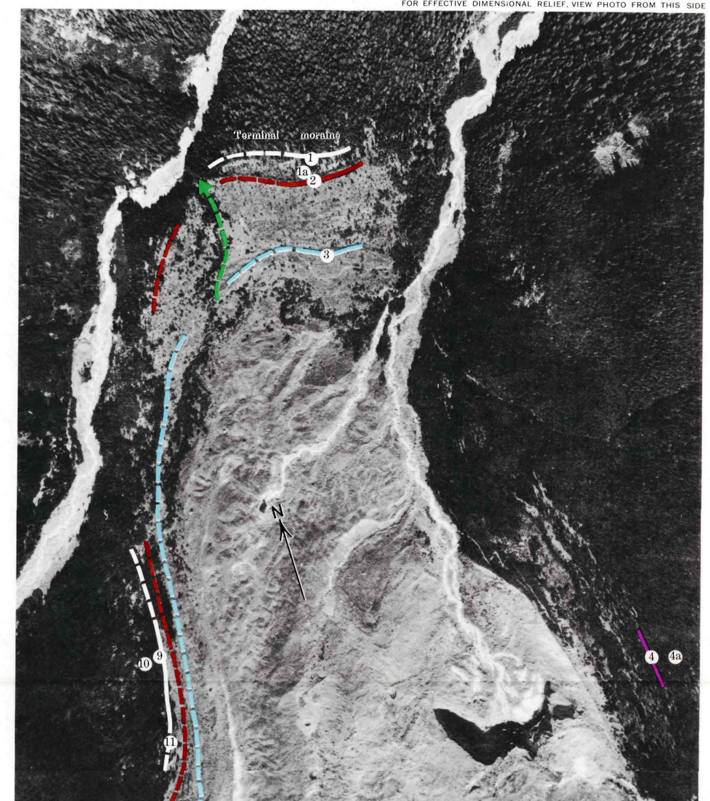
FIGURE 5.—Vertical photograph of West Fork and Winthrop Creek valleys near Winthrop Glacier showing location of the terminal moraine and the lower parts of lateral moraines of Winthrop Glacier, sample areas, and inferred locations of A.D. 1650-70, 1710-20, and 1810 moraines. Surface that appears flat and free of boulders southeast of area 3 and south of the trail is underlain by sediment deposited in a pond dammed by the moraine (fig. 3). For a considerable distance across the relatively bare part of the valley Wonderland Trail follows the A.D. 1810 moraine. Aug. 16, 1967.
