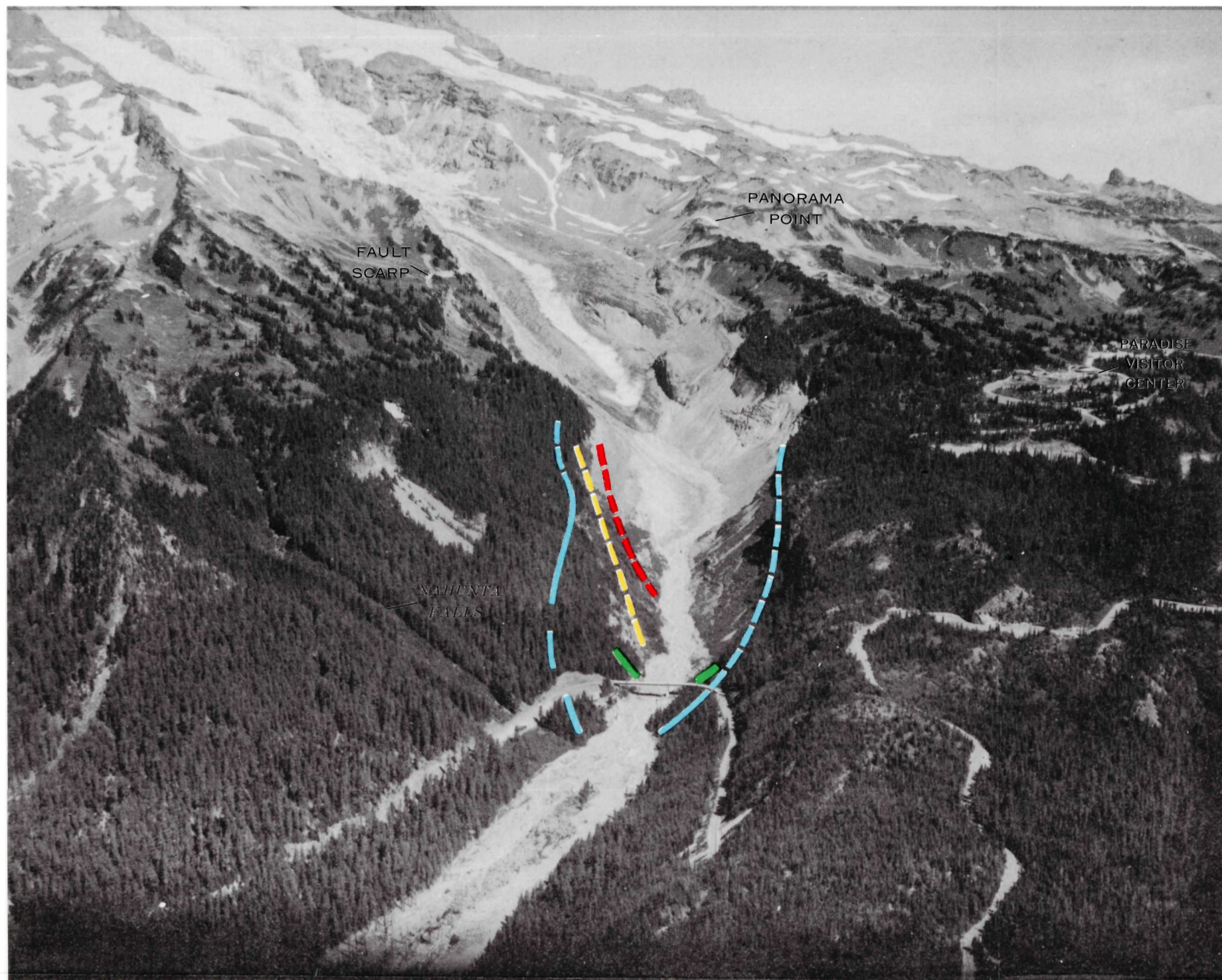
FIGURE 1.—Oblique view of the lower part of Nisqually Glacier taken on Sept. 22, 1966. About 130 years ago, the glacier extended about 600 feet below the bridge and filled the valley from wall to wall within the area enclosed by the blue lines. The terminus could not have been beyond the green line when Lt. A. V. Kautz saw it in 1857. The yellow line marks the glacier's approximate position in 1870 and the red line in 1900. Aug. 29, 1969
