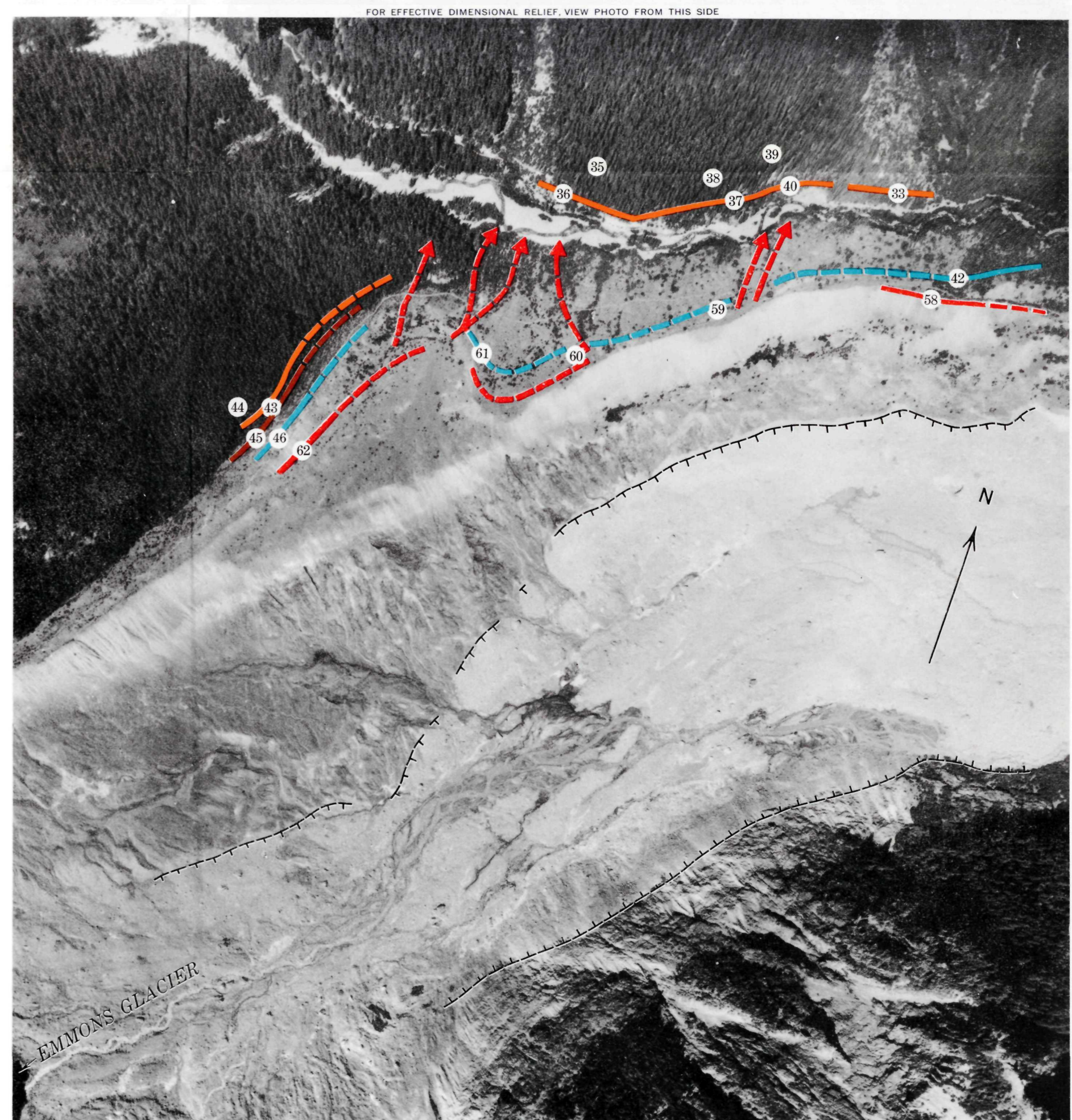
FIGURE 7.—Vertical aerial photograph of a part of Inter Fork and White River valleys showing positions of Emmons Glacier lateral moraines and sample areas. The A.D. 1550-1600 moraine, shown in black, marks the maximum known extent of Emmons Glacier in 10,000 years. The stream across the top third of the picture is Inter Fork, and paralleling it on the north side is Glacier Basin Trail, Aug. 16, 1967.
