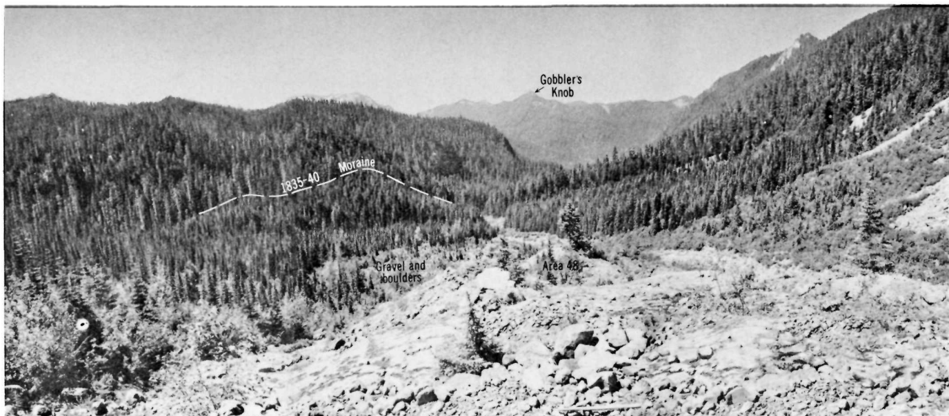
FIGURE 7.—Tahoma Glacier covered the rocks in the foreground and filled the lowland of South Puyallup River to the left of and just beyond gravel and boulders as recently as 1860. About 1835-40, Tahoma Glacier started to recede from area of the dashed line.
