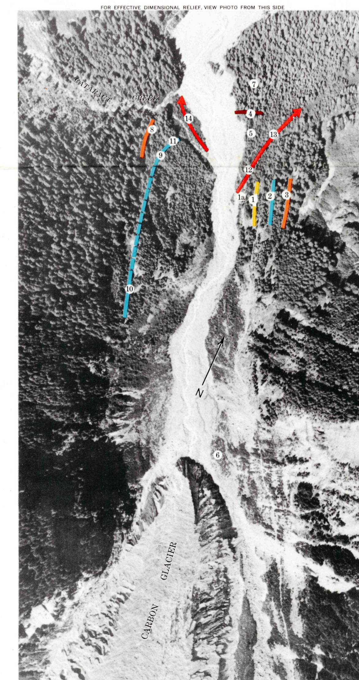
FIGURE 4.—Vertical photograph of Carbon Glacier showing sample areas and moraines. Wonderland Trail can be seen northwest from area 1 along the west side of the valley to the bottom of the photograph. Prior to a flood in 1959, which destroyed the trail bridge, Wonderland Trail crossed Carbon River near the mouth of Cataract Creek and remnants can be seen near area 1 and between areas 14 and 11. Comparison of the position of Carbon Glacier in this photograph taken on Aug. 16, 1967, with that in figure 1, taken on Sept. 2, 1962, indicates that the glacier was farther downvalley in 1967.
