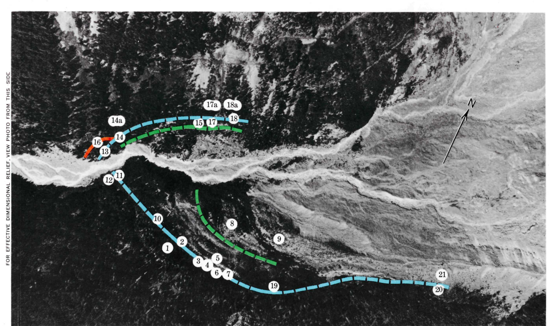
FIGURE 6.—Vertical photograph of South Tahoma Glacier valley showing location of sample areas and moraines. In the early 16th century South Tahoma Glacier was nearly as extensive as it was 130 years ago. A fragment of 1550 moraine lies at the junction of Tahoma Creek Trail and Wonderland Trail (area 16) and extends southward toward Tahoma Creek. Photograph taken Aug. 16, 1967.
