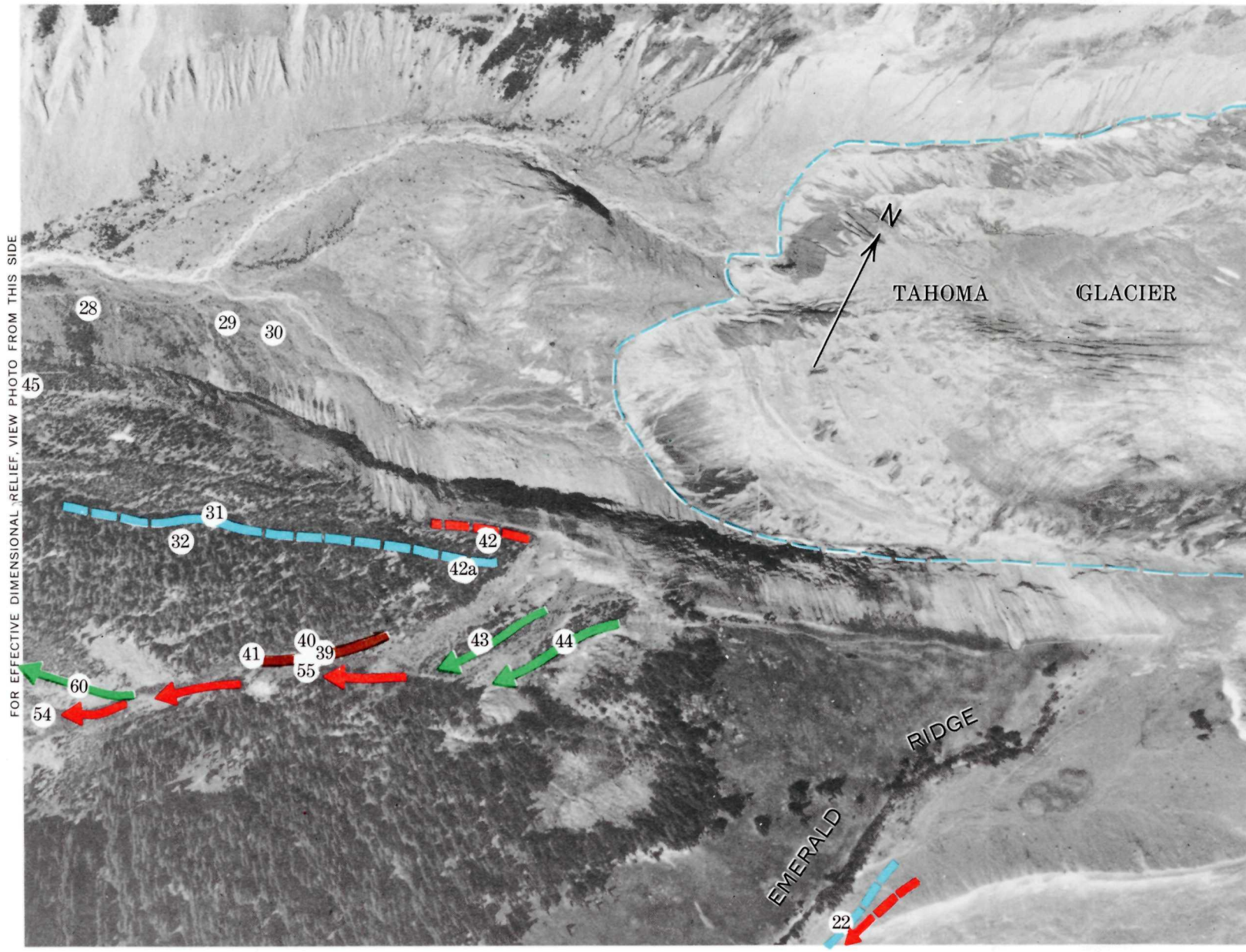
FIGURE 2.—Vertical photograph of South Puyallup River and terminus of Tahoma Glacier marked by this blue dashed line. The red and green arrows mark a valley through which melt water flowed until about 1910. Aug. 16, 1967.
