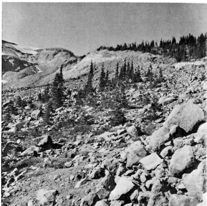
FIGURE 13.—These trees are the closest to Ohanapecosh Glacier, and the oldest was 3 inches tall in 1878. Pumice erupted by Mount Rainier between 115 and 150 years ago is present on the surface here; so the moraine is older. The bare bouldery surface on the right is older than the surface upon which the trees are growing and does not support trees, presumably because no fine soil is present in which seed can germinate. Ohanapecosh Glacier is out of view to the left. Sept. 26, 1967.
