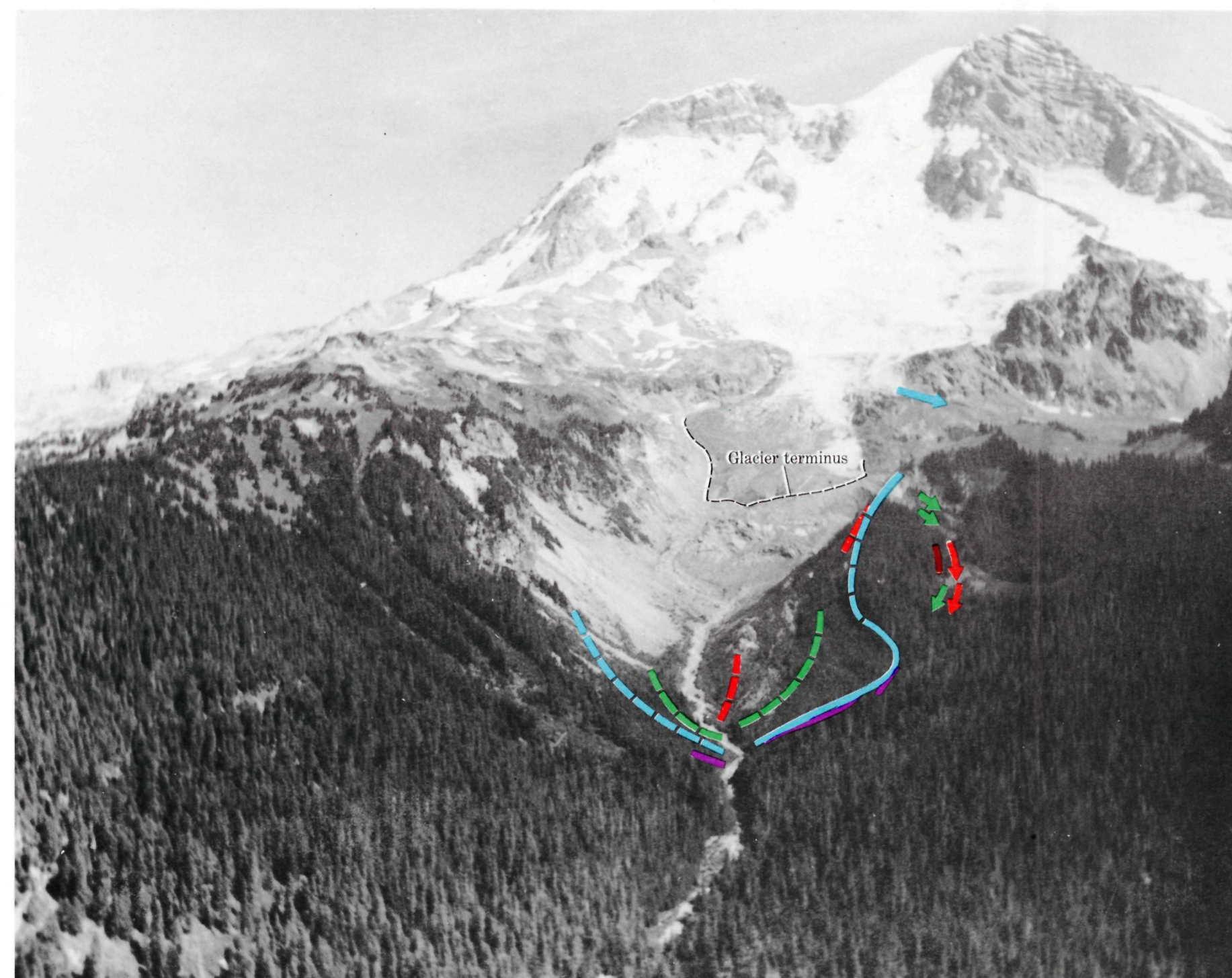
FIGURE 5.—Oblique view from the west of Tahoma Glacier which filled the valley in the center within the area marked by the blue line. It also flowed southward (blue arrow) to join South Tahoma Glacier. Aug. 29, 1969.
