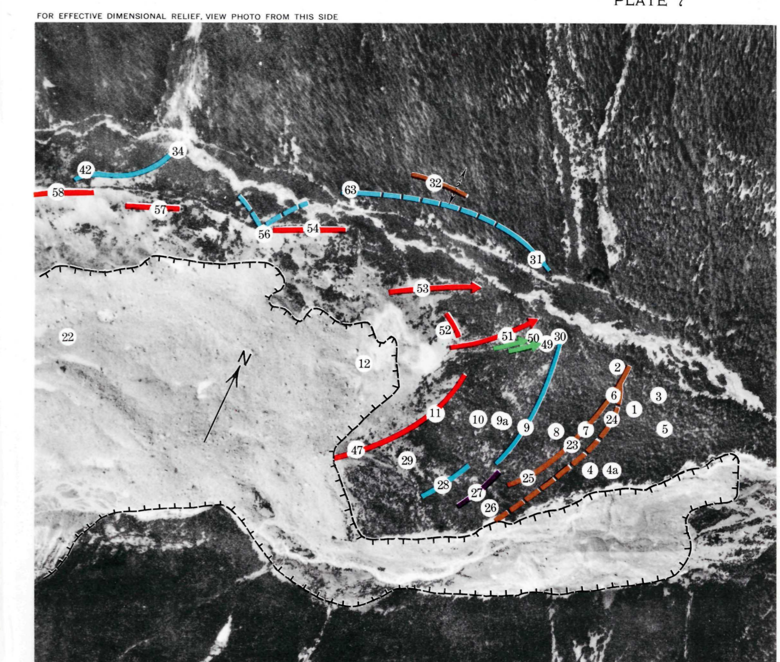
FIGURE 9.—Vertical photograph of Emmons Glacier terminal moraine about one-half mile west of White River Campground shows sample areas, moraines, and melt-water channels. Dashed brown line represents the maximum known downvalley limit of Emmons Glacier within the last 10,000 years. It had receded an unknown distance by A.D. 1655. The solid brown line represents a moraine crest upon which the oldest trees were 2 feet tall in A.D. 1745. The blue and red lines represent moraine crests successively younger, and the red line is at the approximate position of the glacier when mapped in 1910-13 as part of the Mount Rainier National Park topographic quadrangle. Photograph taken Aug. 16, 1967.
