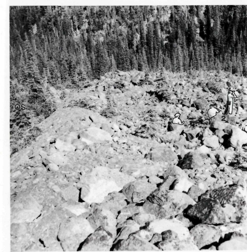
FIGURE 2.—Rock covered surface at the left of center (area 1) is the modern terminal moraine of Winthrop Glacier. The oldest tree here was 2 feet tall in A.D. 1730. Trees at the extreme left are on an older surface (OS). Man is standing in area 2 where the oldest tree was 2 feet tall in A.D. 1760. The younger moraine, area 3, is out of the picture to the right. Winthrop Creek is at the base of the hill in background flowing to the left in a northward direction. View is easterly. July 22, 1962.
