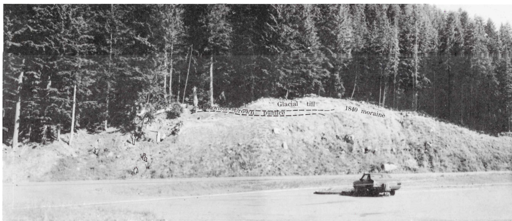
FIGURE 2.—Terminal moraine of Nisqually Glacier is cut by the road at the west end of the bridge and continues downslope through the forest to the river. Nisqually Glacier started to recede from here about 1840, as the oldest trees along this moraine were 2 inches to 2 feet tall in 1842-47. This position marks the maximum advance of Nisqually Glacier in 10,000 years. To the left, downvalley, trees are large and old, and the forest floor is covered with logs in all stages of decay. Beneath the humus here is a sandy yellowish pumice that was deposited 3,900 to 3,500 years ago. Aug. 1969
