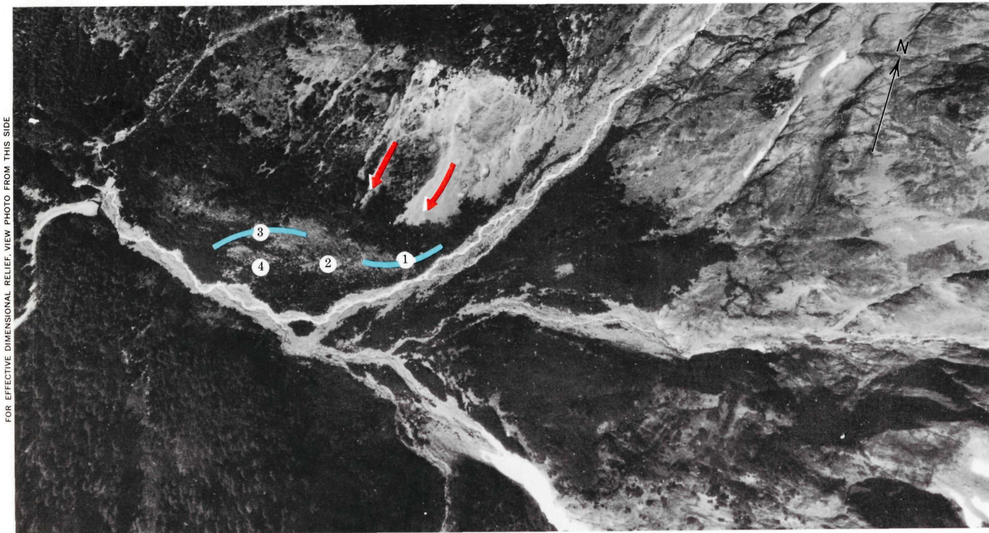
FIGURE 1.—Vertical photograph of North Puyallup River valley showing sample areas, location of early 19th century position of the Puyallup Glacier, and two active rock taluses that have buried the moraine or destroyed the trees on it. Trees felled by wind or snow avalanching are seen between areas 1 and 3. Parking area at end of abandoned part of West Side Road is visible near the center at left. Glacier is out of view at the right. Photograph taken Aug. 16, 1967.
