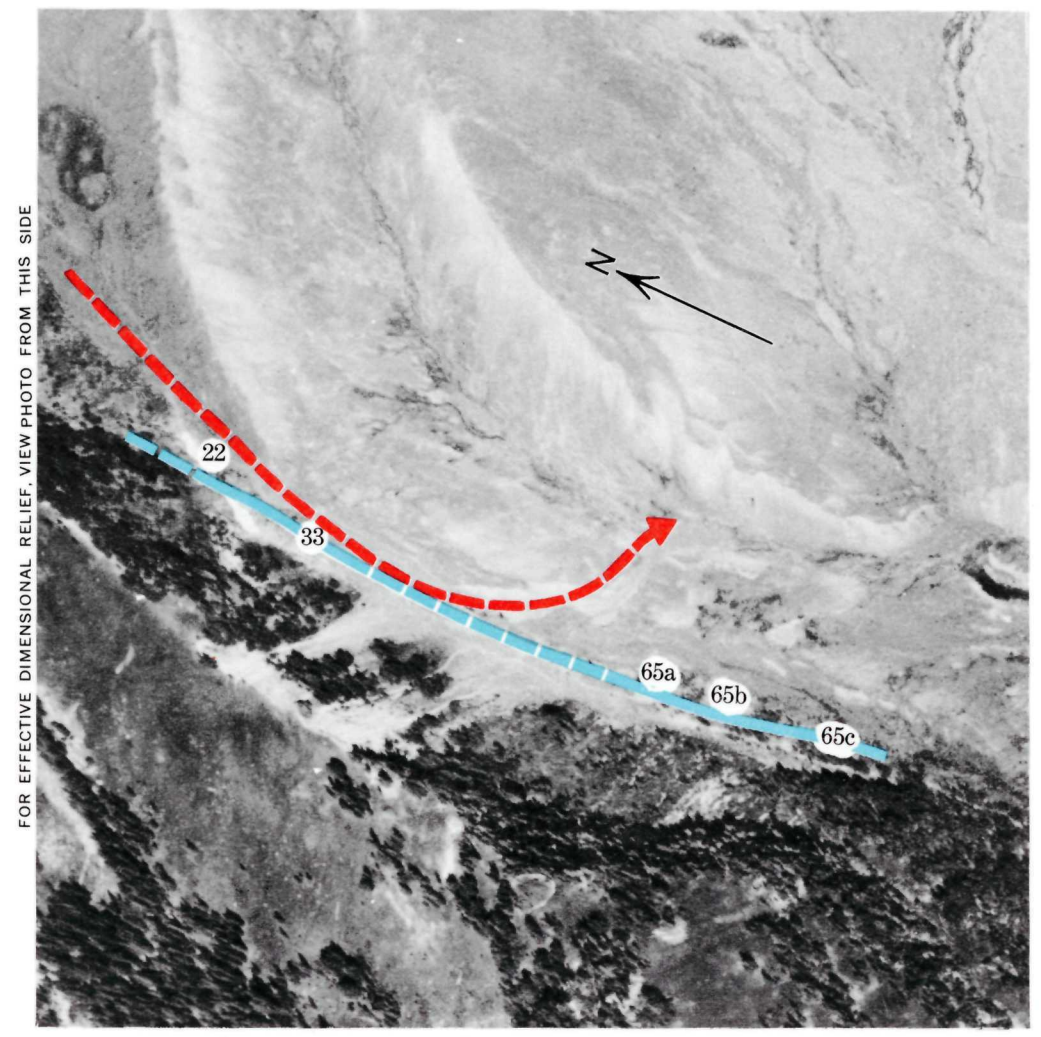
FIGURE 1.—Vertical photograph of Emerald Ridge showing moraines, sample areas, and a large abandoned melt-water channel (red arrow). The glacier started to recede from the moraine before 1850 at the time it started to recede from moraines southwestward in Tahoma Creek valley (map and fig. 6). Melt-water from the receding glacier cut a deep channel through the moraine sometime late in the last century. Aug. 16, 1967.
