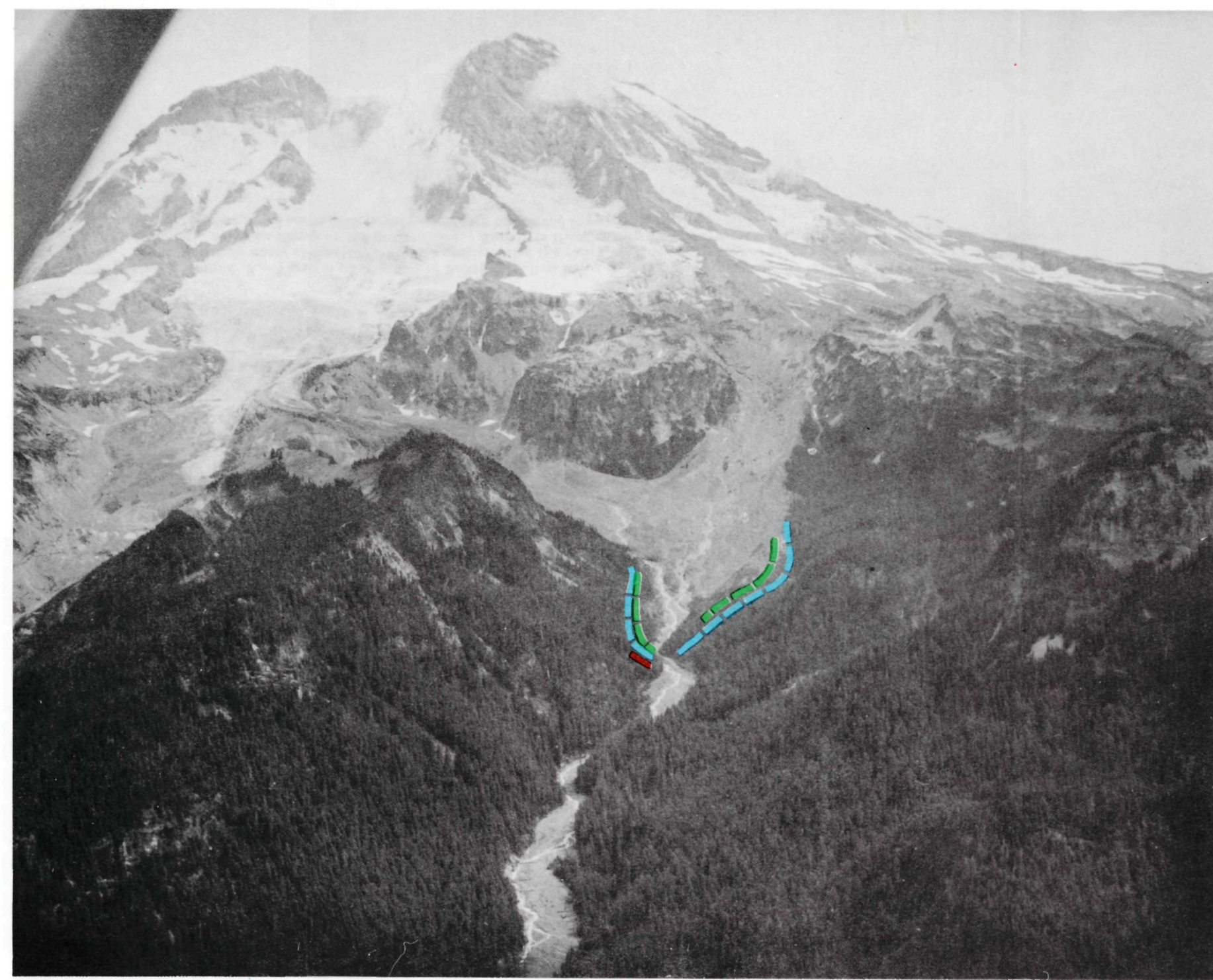
FIGURE 4.—Oblique view from the west of South Tahoma Glacier which 130 years ago filled the valley in the foreground within the area marked by the blue line. It was joined by the left arm of Tahoma Glacier, which occupied the barren valley extending left to right, and left moraines on the west side of the valley below the prominent hill (Glacier Island) in the foreground and on Emerald Ridge on the left. Aug. 29, 1969.
