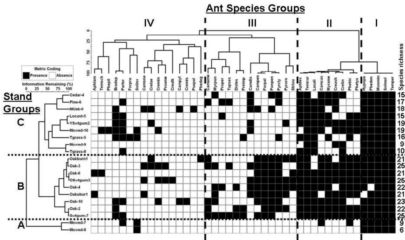
Figure 2. Dendrogram providing a 2-dimensional picture of the combined relationships among stands (rows) and ant species (columns) at Arkansas Post National Memorial. See methods for stand descriptions. Three stand groups were identified: Group A representing mowed sites without trees, Group B successional “older” stands, and Group C successional “younger” stands. Four ant species groups were also identified: Group I included the 5 most ubiquitous ants; Group II, 9 common ants that occur in most stands in Groups B and C, but were mostly absent from Group A; Group III, 13 less common ants, that were more species rich in Group B than Group C, and were absent from Group A; and Group IV, 16 ants that were hard to characterize to habitat, and included all 6 rare species (found in only one stand type). Cluster “breaks” within the dendrogram were on a sliding scale with a value of 100 being most similar and 0 being very dissimilar. Natural groups had longer stems in the dendrogram, and very divergent groups were typically linked where the information remaining scale shows zero.
